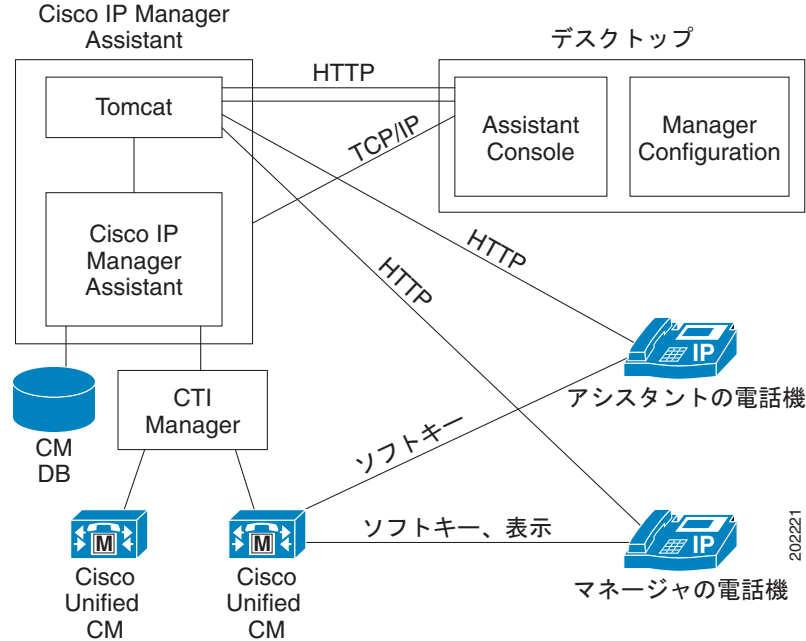
図 11-1 Cisco Unified Communications Manager Assistant のアーキテクチャ
