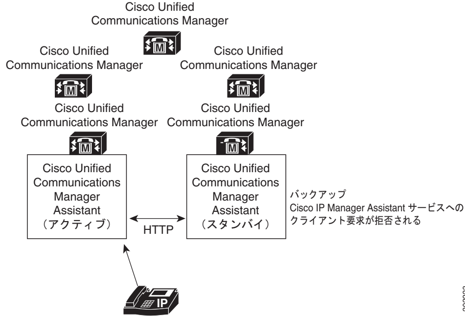
図 11-3 Cisco Unified Communications Manager Assistant の冗長性
