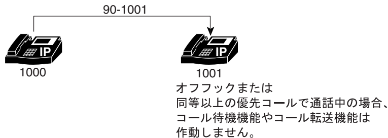
図 12-11 Blocked Precedence Announcement の例
