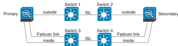
図 5: Connecting with a Secure Switch
