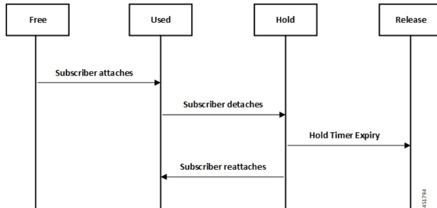
Figure 20: Address State Change with Hold Timer
