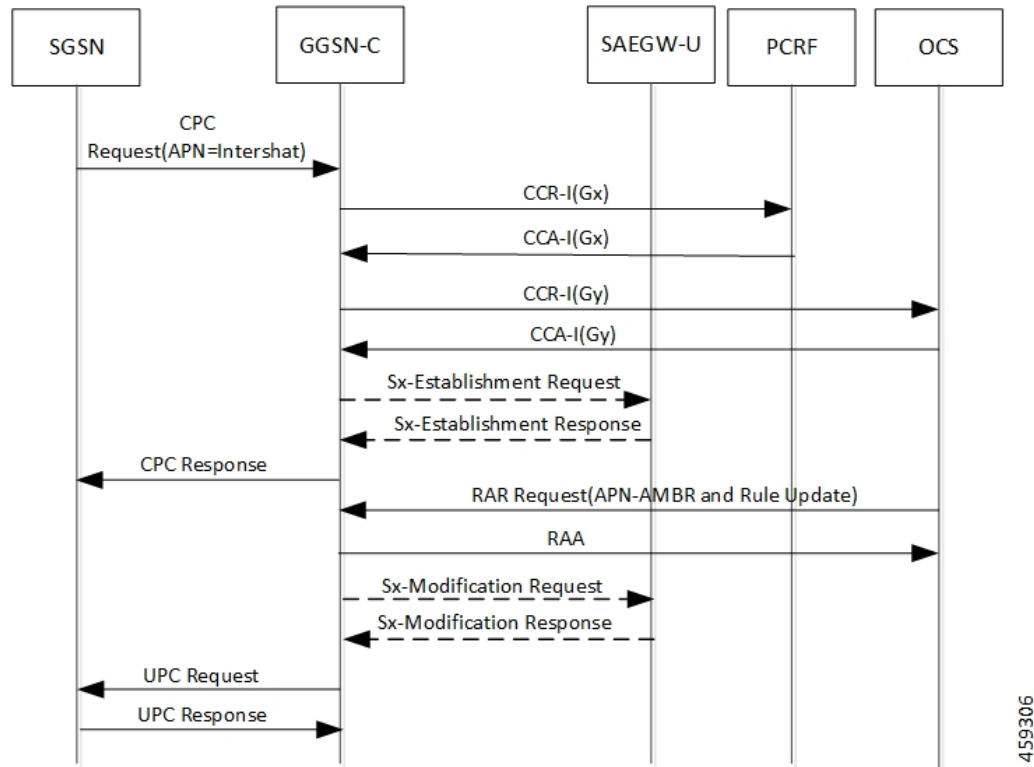
Figure 52: VAPN Selection
