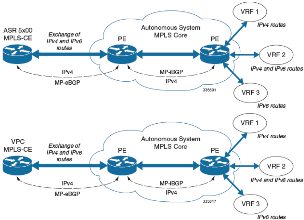
Figure 29: VPNv6 Sample Configuration
