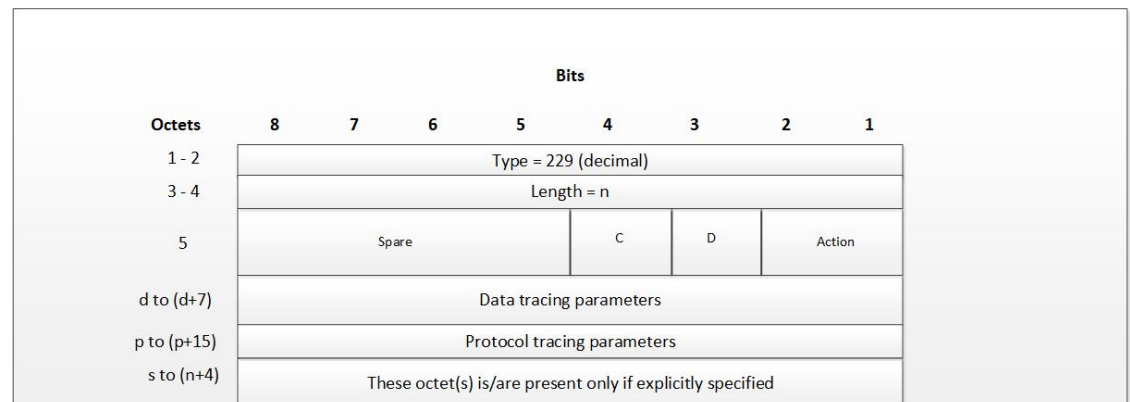
Figure 22: Subscriber Tracing
