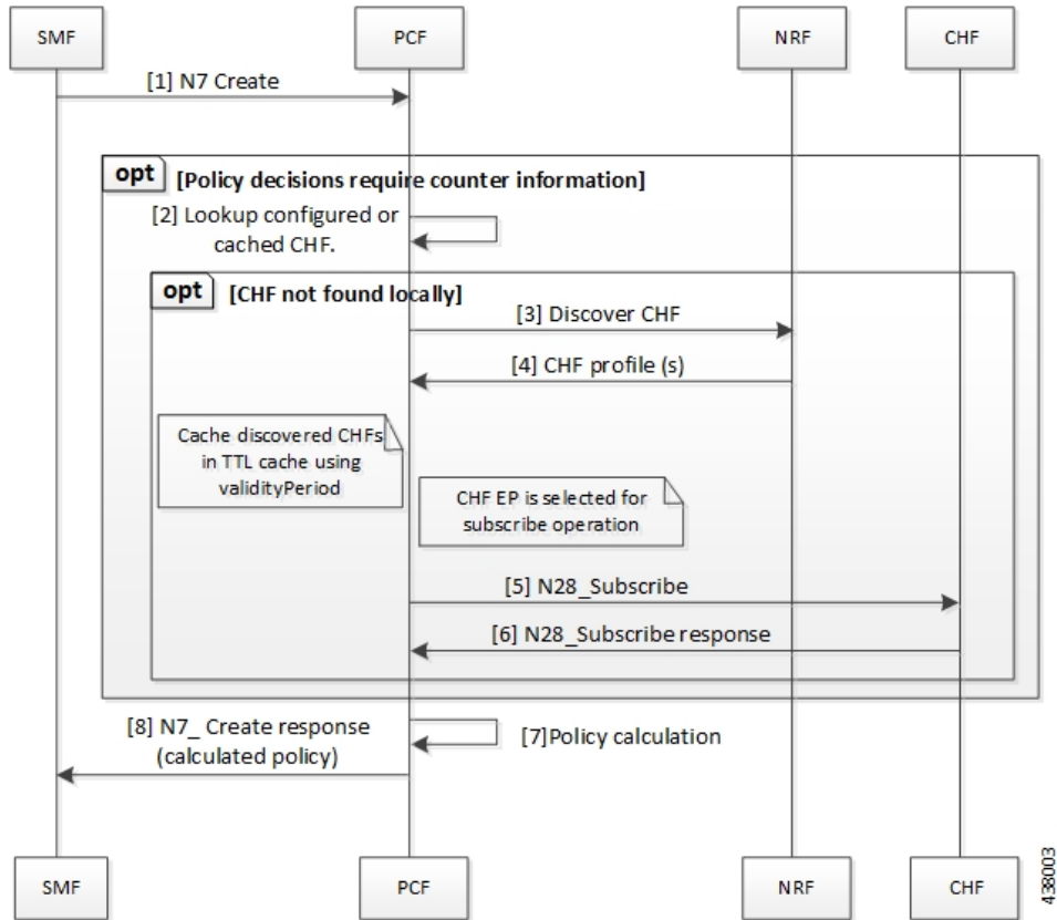
Figure 40: N28 Subscribe (N7 Create) Call Flow
