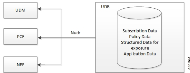
Figure 77: N36 Reference Point
