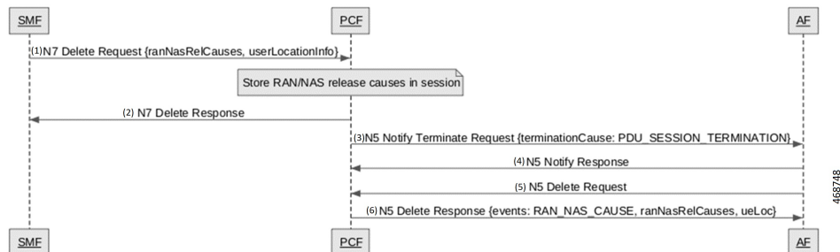
Figure 57: PCC Rule Installation and Modification Failures Call Flow
