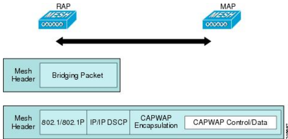
Figure 51: Encapsulating Mesh Traffic
