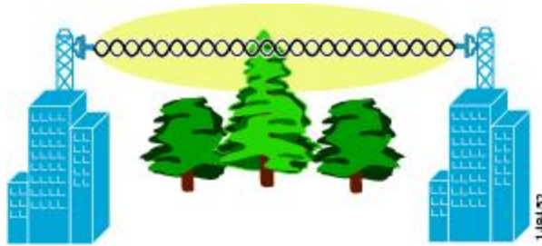
Figure 12: Typical Obstructions in a Fresnel Zone
