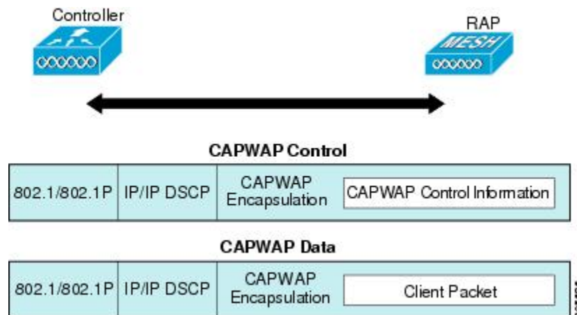
Figure 29: Mesh Network Traffic Termination
