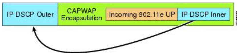
Figure 53: MAP to RAP Path
