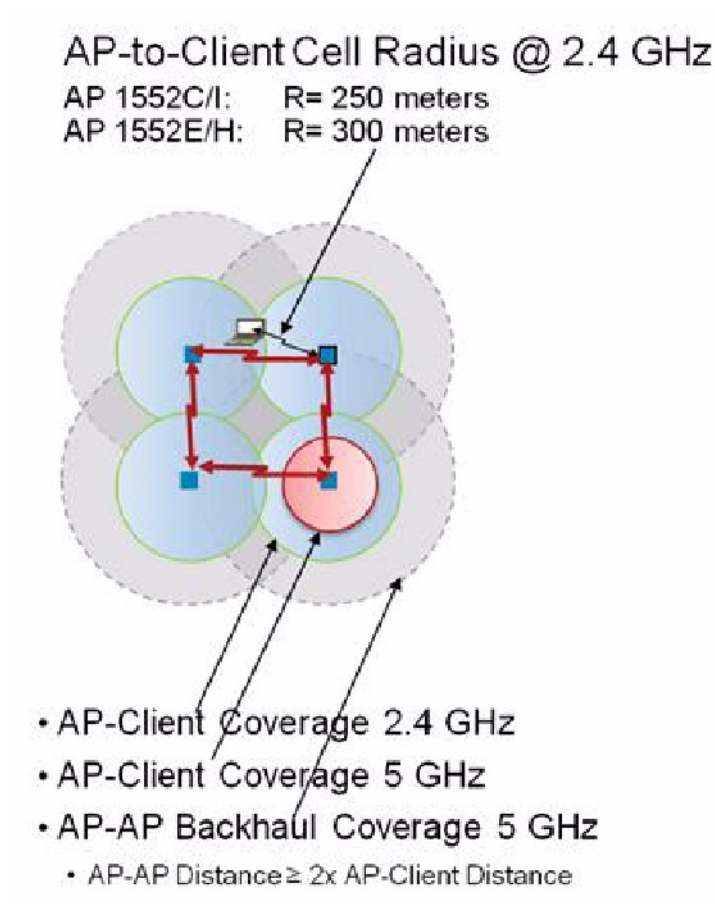
Figure 19: AP-to-Client Cell Radius at 2.4 GHz
