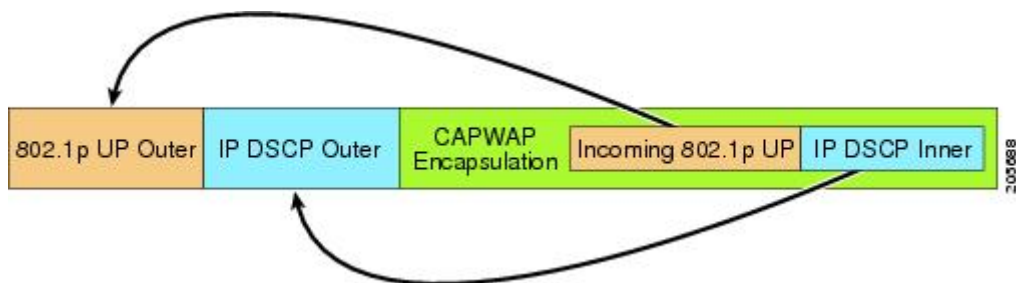
Figure 52: Controller to RAP Path
