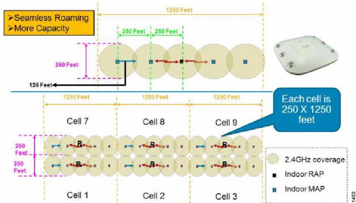
Figure 25: Cell Radius of 125 Feet (38 meters) and Access Point Placement for Indoor 11n Mesh Networks
