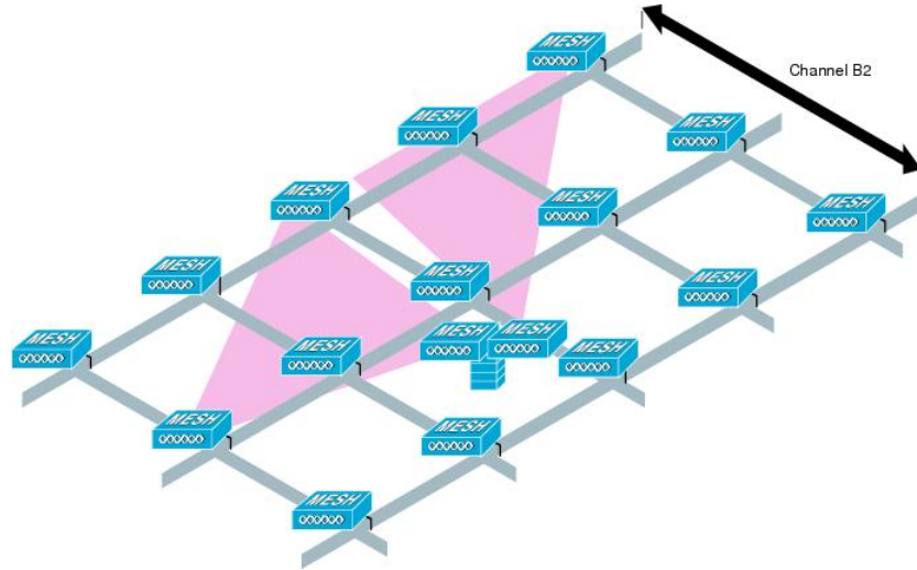
Figure 28: Two RAPs per Cell on Different Channels
