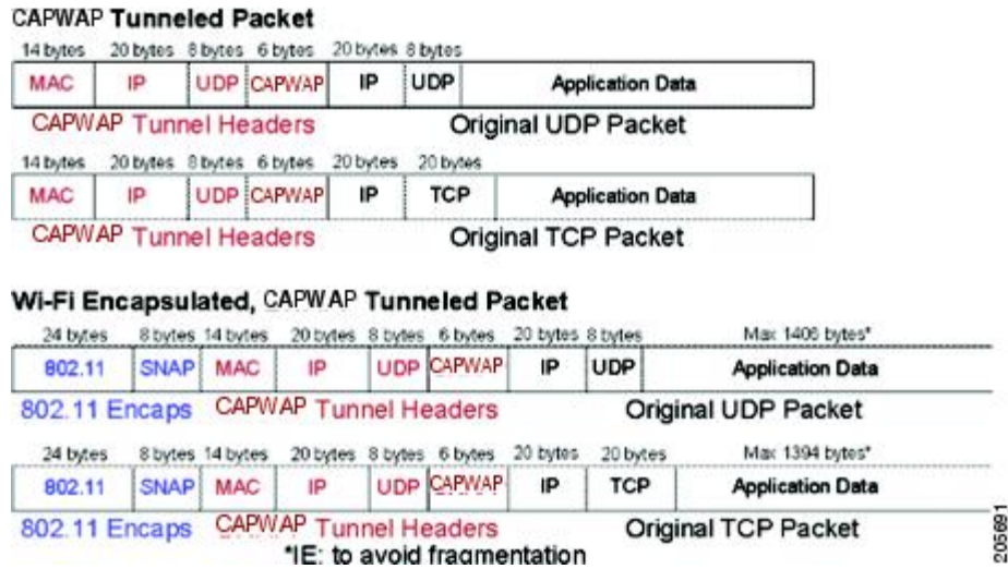
Figure 9: CAPWAP Tunneled Packets
