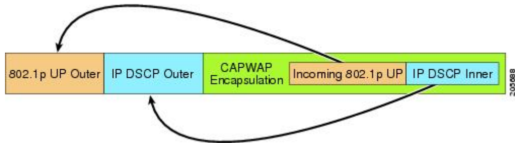
Figure 61: Controller to RAP Path
