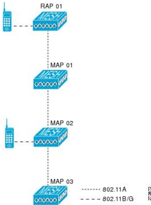
Figure 63: Mesh Network Example
