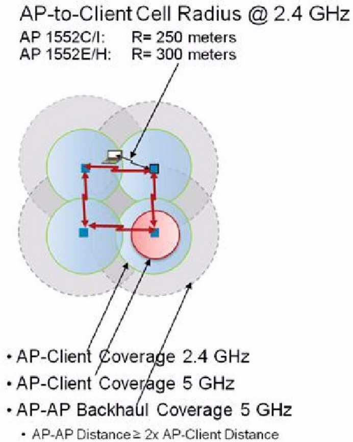
Figure 27: AP-to-Client Cell Radius at 2.4 GHz
