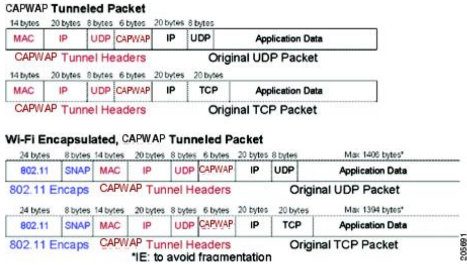
Figure 74: CAPWAP Tunneled Packets
