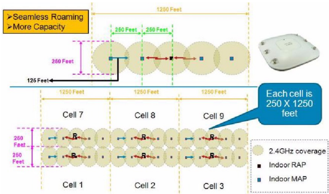
Figure 33: Cell Radius of 125 Feet (38 meters) and Access Point Placement for Indoor 11n Mesh Networks
