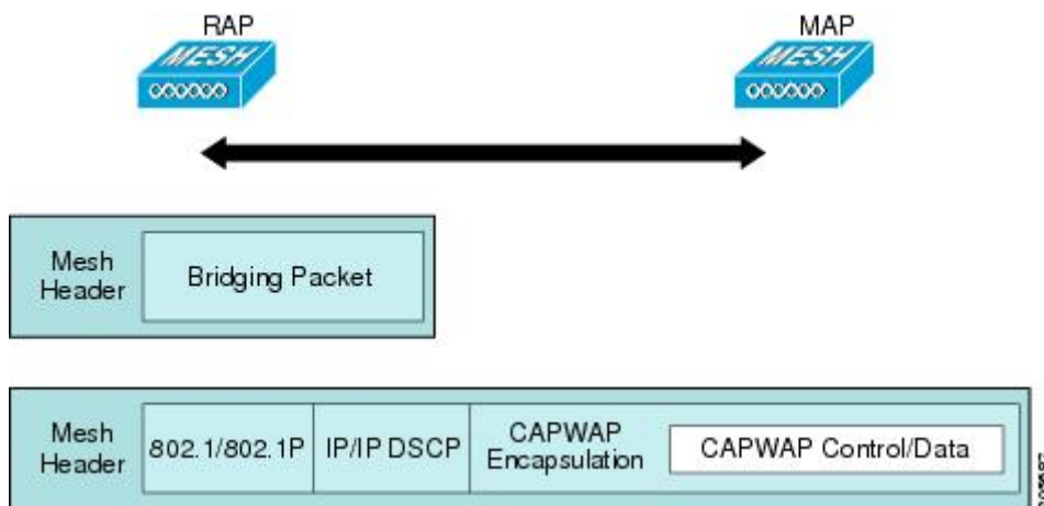
Figure 60: Encapsulating Mesh Traffic
