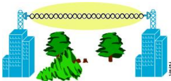
Figure 21: Removing Obstructions in a Fresnel Zone
