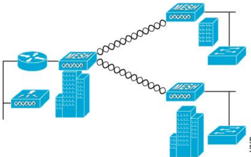
Figure 40: Point-to-Multipoint Bridging
