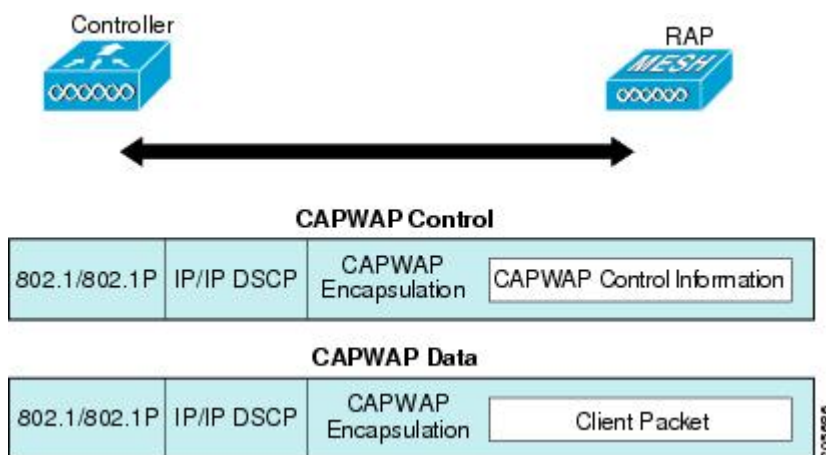
Figure 54: Encapsulations
