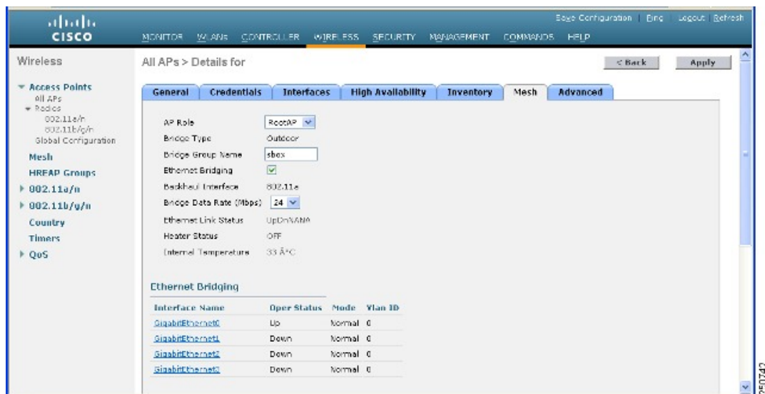
Figure 36: All APs > Details for (Mesh) Page
