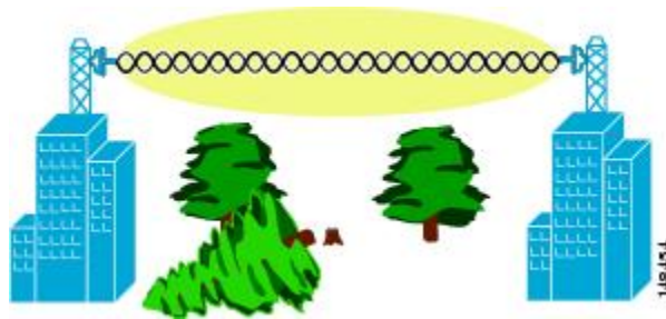
Figure 17: Removing Obstructions in a Fresnel Zone
