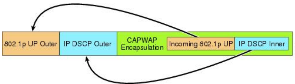
Figure 56: Controller to RAP Path
