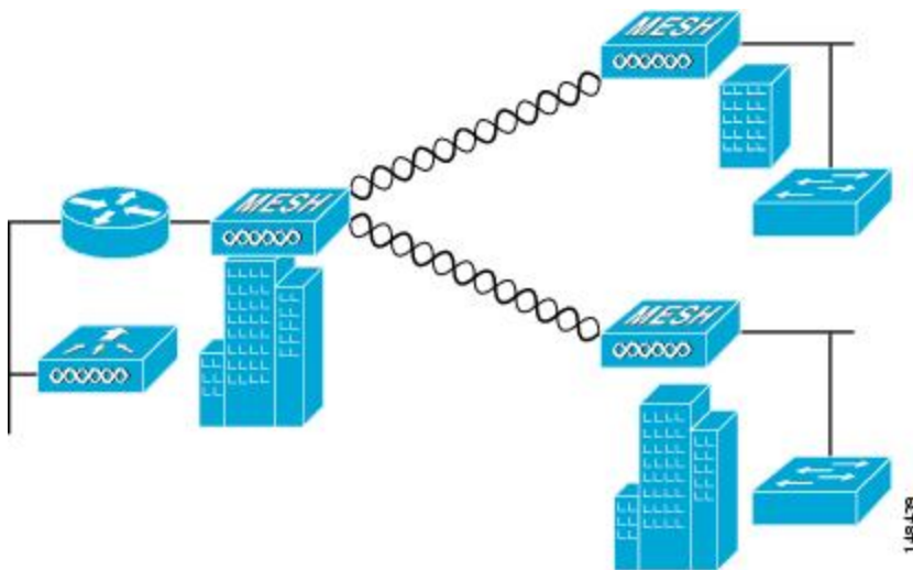
Figure 40: Point-to-Multipoint Bridging
