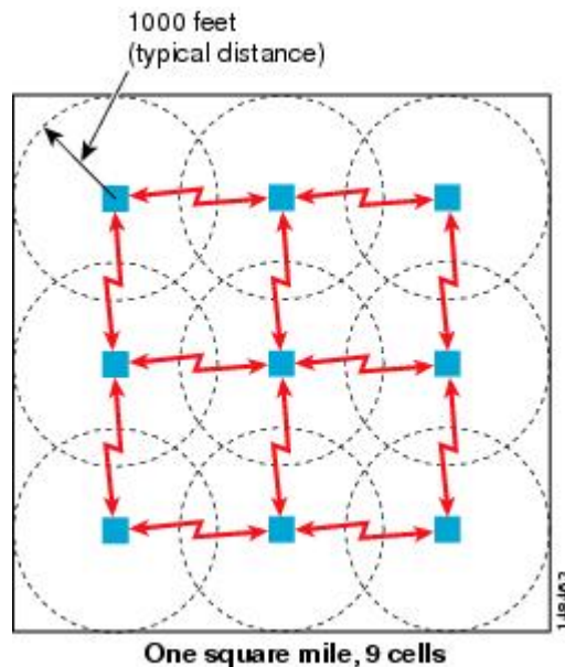
Figure 19: Cell Radius of 1000 Feet and Access Point Placement for Nonvoice Mesh Networks
