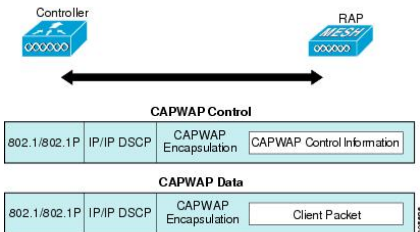
Figure 54: Encapsulations
