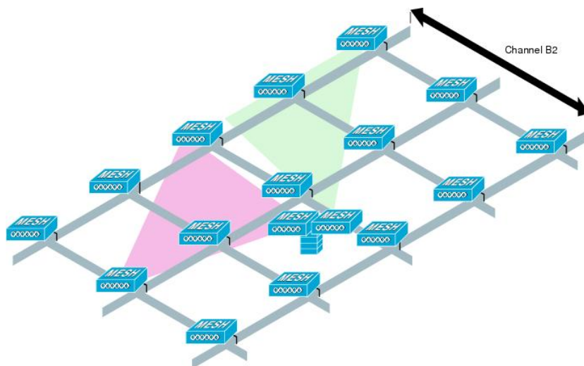
Figure 32: Two RAPs per Cell on Different Channels
