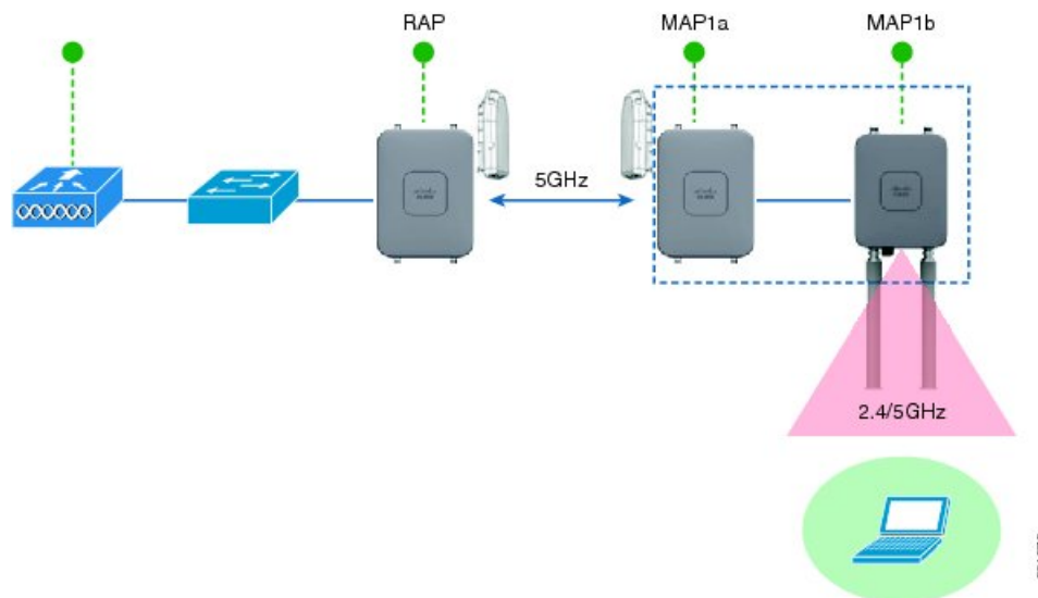
Figure 64: Daisy Chaining to Extend Universal Access
