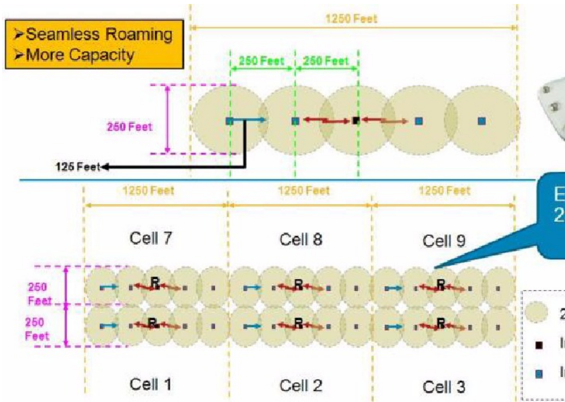
Figure 29: Cell Radius of 125 Feet (38 meters) and Access Point Placement for Indoor 11n Mesh Networks
