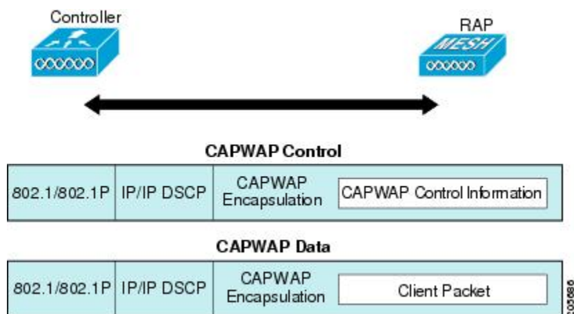
Figure 33: Mesh Network Traffic Termination
