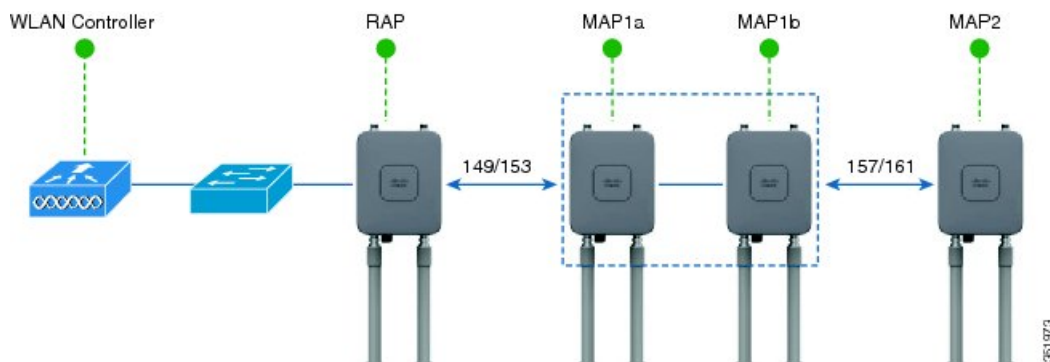
Figure 63: Daisy Chaining with Serial-Backhaul Mesh
