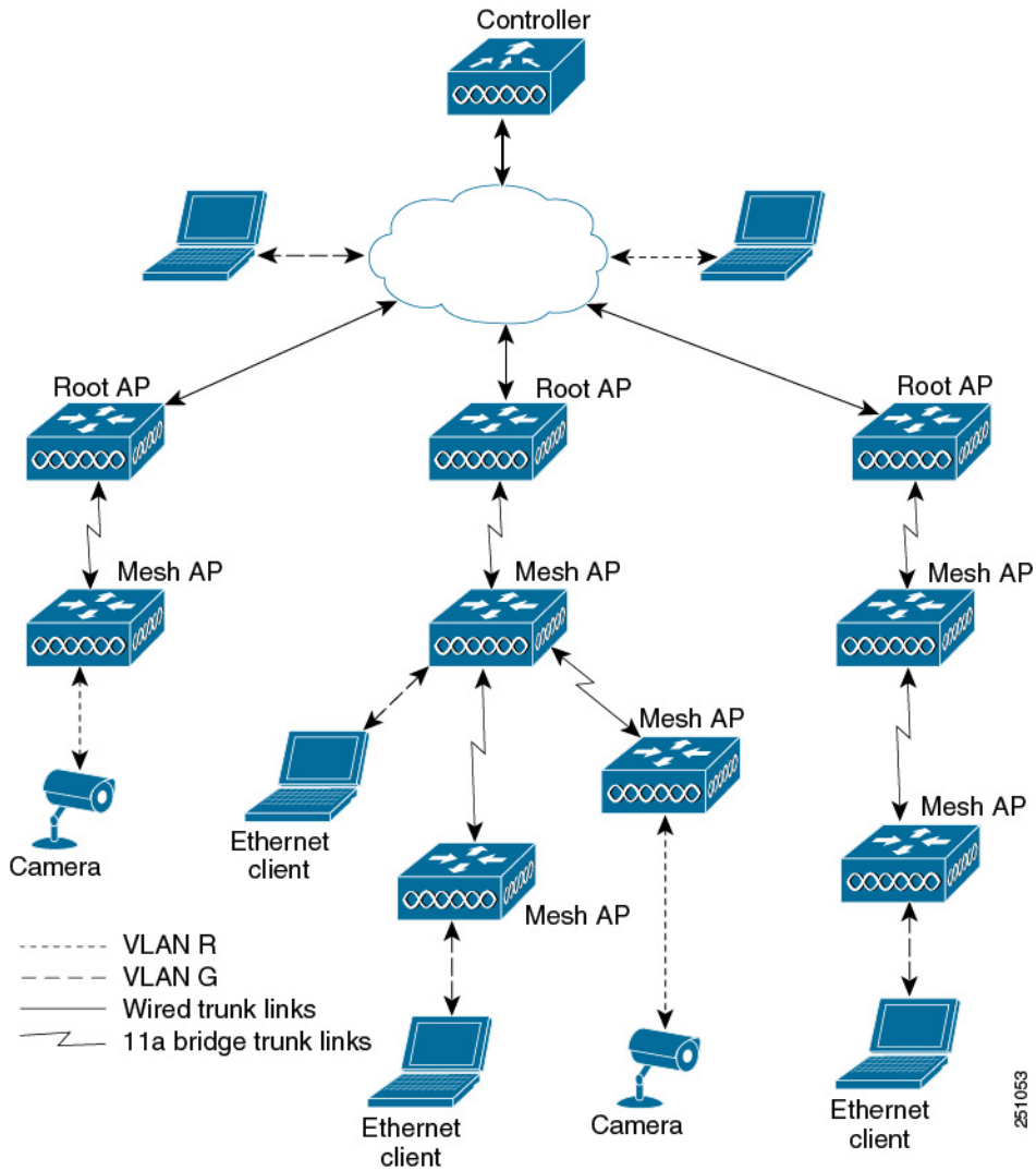
Figure 42: Ethernet VLAN Tagging
