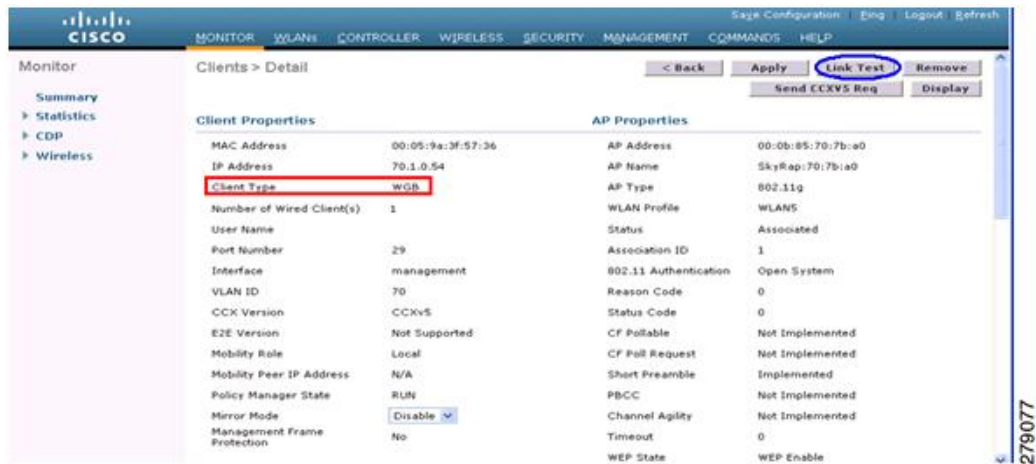
Figure 52: Updated WGB Clients
