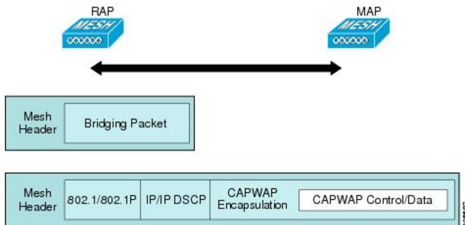
Figure 55: Encapsulating Mesh Traffic
