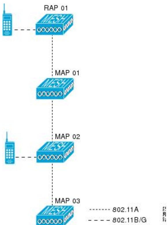
Figure 58: Mesh Network Example
