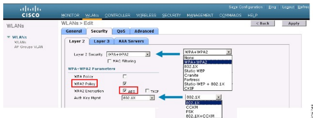
Figure 45: WPA-2 Security Settings for a WGB
