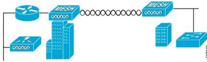
Figure 14: Point-to-Point Bridging Example
