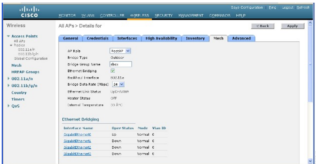
Figure 36: All APs > Details for (Mesh) Page
