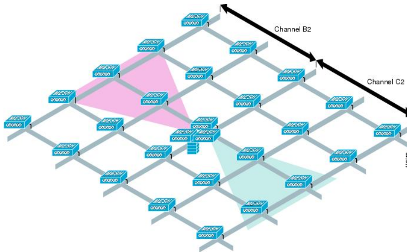
Figure 24: PoP with Multiple RAPs
