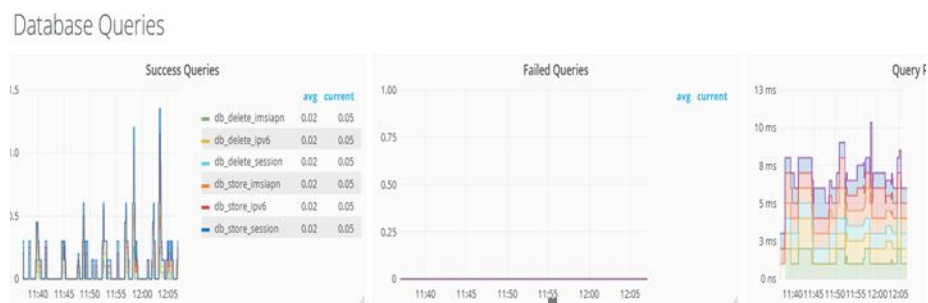
Figure 9: Database Queries
