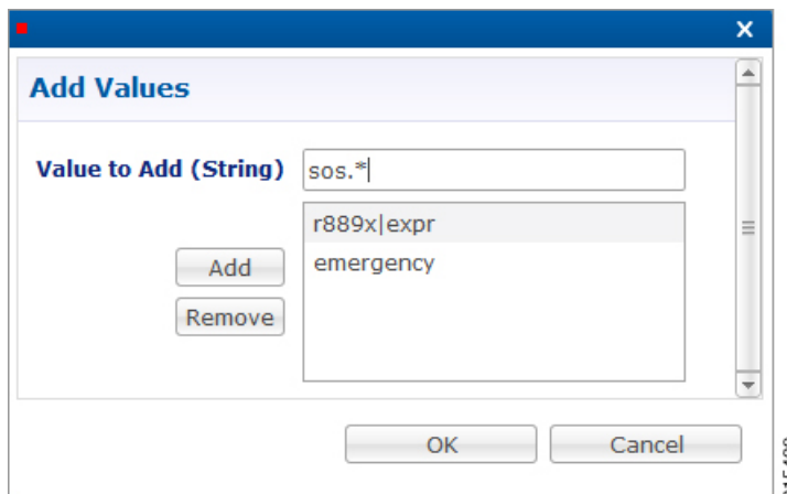
Figure 15: Add Values
