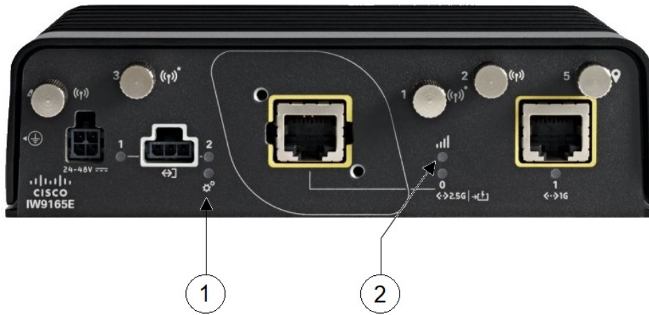
Figure 2: IW9165E LEDs
