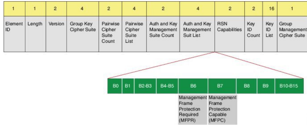
Figure 28: 802.11w Information Elements
