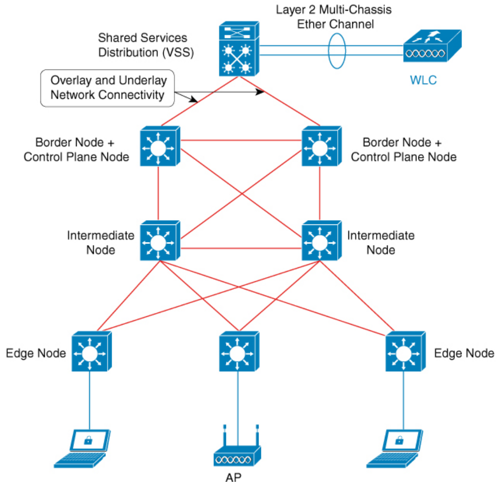
Figure 24: SD-Access Wireless
