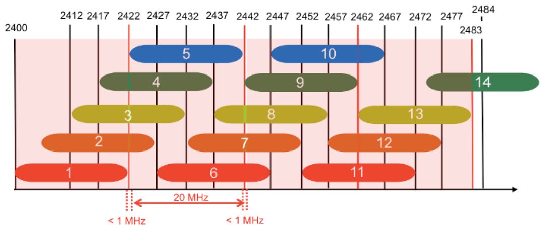
Figure 3-4 2.4 GHz Channels Showing 1/5/9/13 Selected
