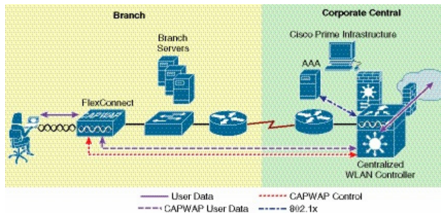
Figure 7-2 Authentication-Central/Switch-Central WLAN
