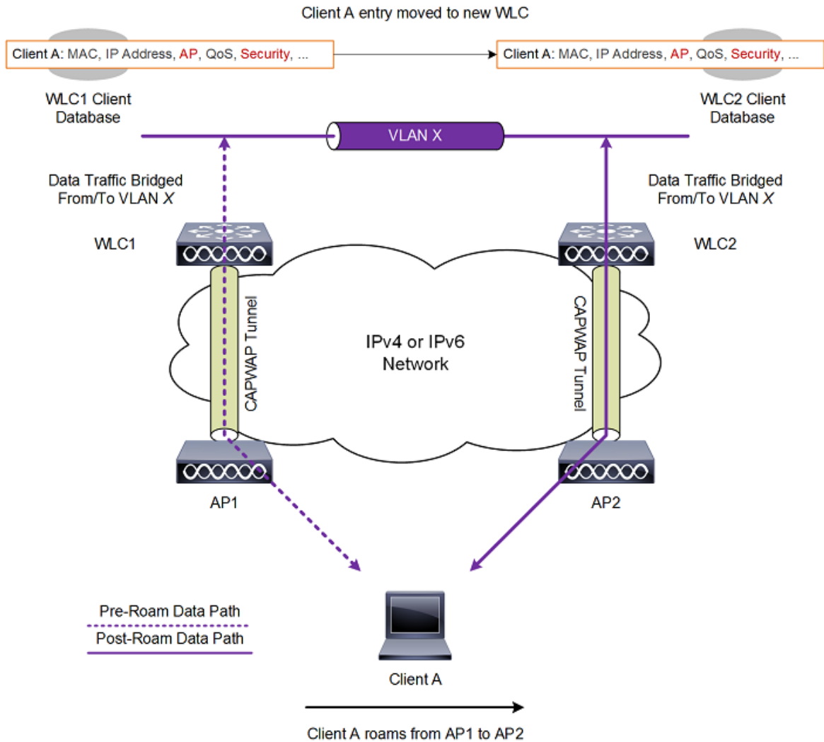
Figure 2-31 Inter-Controller Roaming
