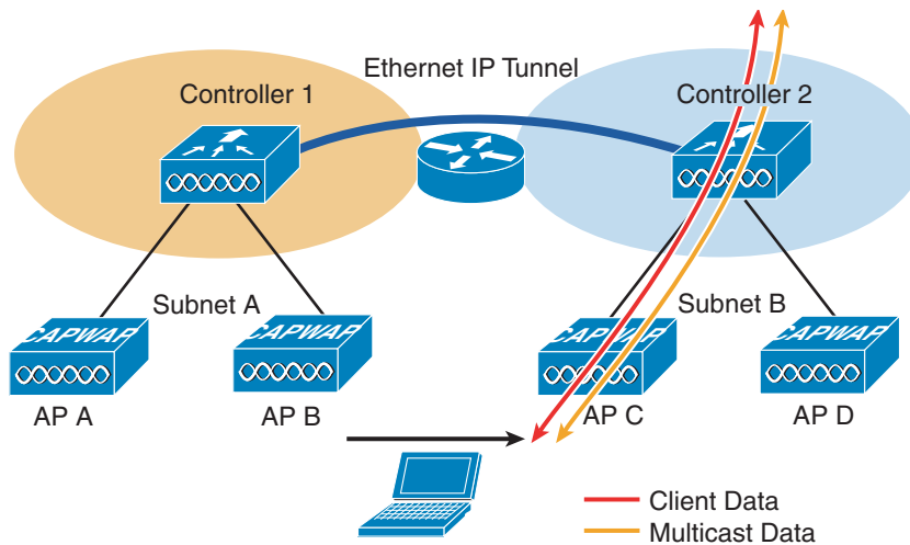
Figure 6-2 Asymmetric Tunneling
