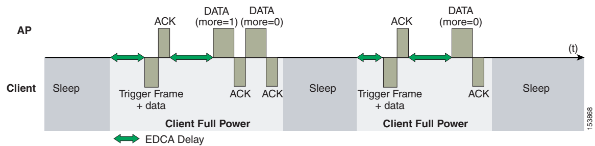
Figure 5-12 U-APSD
