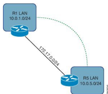
Figure 43: Route-based VPN
