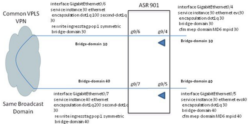
Figure 2: Configuring Multi-NNI CFM in the Same VPN
