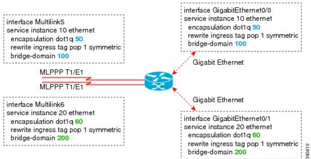
Figure 47: Multilink with a Single EFP
