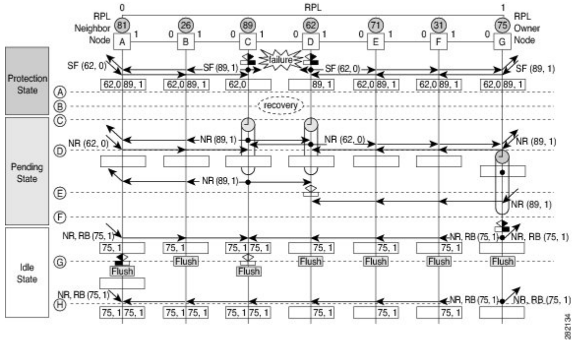
Figure 56: Single-Link Failure Recovery (Revertive Operation)
