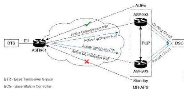
Figure 16: Pseudowire Redundancy with Unidirectional Active-Active
