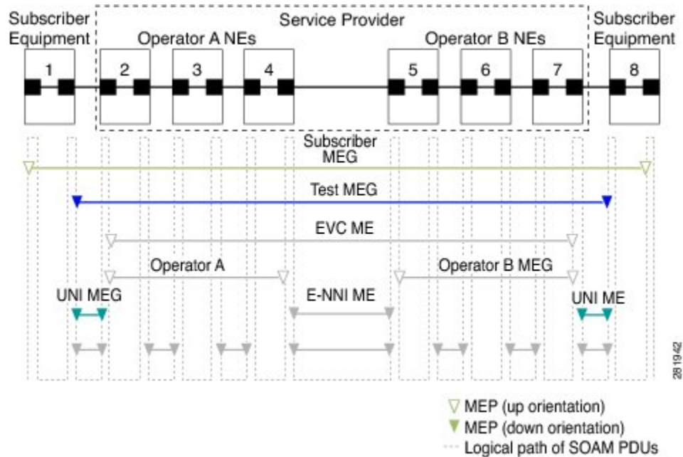
Figure 6: A Point-to-Point Metro Ethernet Deployment with Typical Maintenance Entities and Maintenance Points
