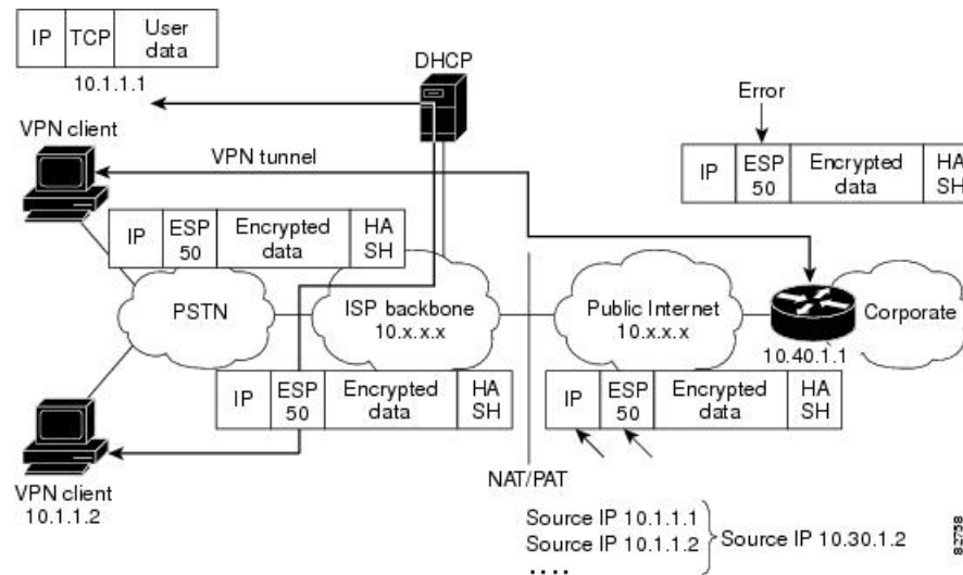
Figure 44: Standard IPsec Tunnel Through a NAT/PAT Point (No UDP Encapsulation)
