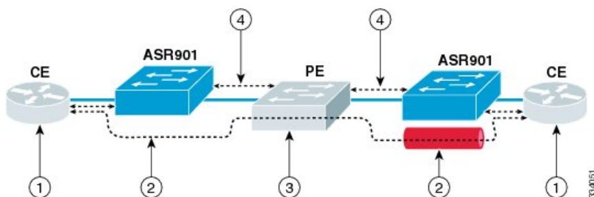
Figure 38: Layer 2 Forwarding
