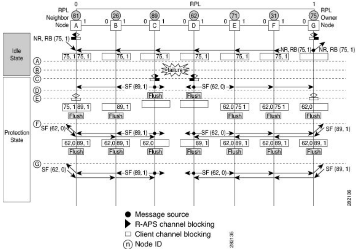
Figure 55: G.8032 Ethernet Ring Protection Switching in a Single-Link Failure
