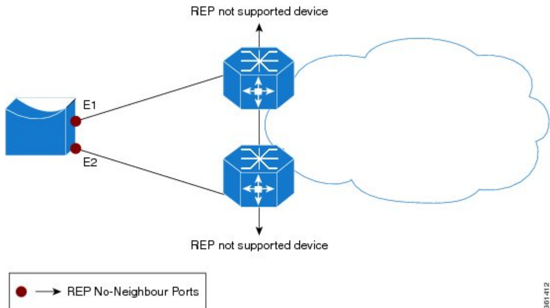
Figure 11: Dual Edge No-neighbor Topology
