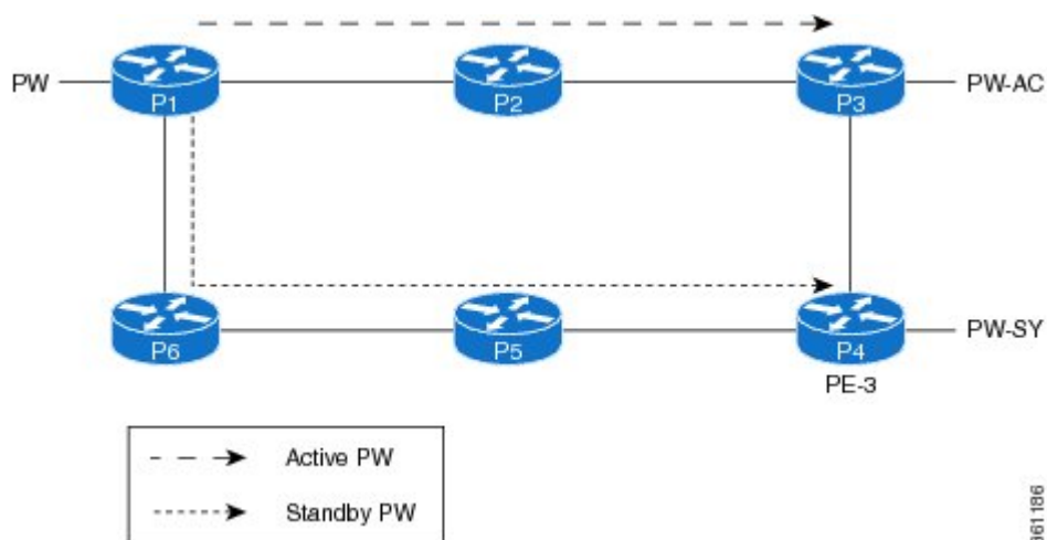
Figure 41: Pseudowire Redundancy Over FRR
