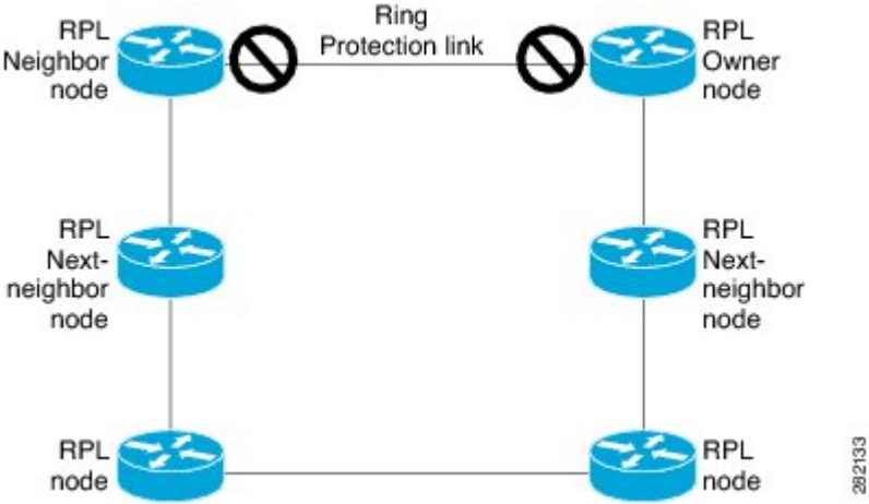
Figure 52: G.8032 Ethernet Ring Topology
