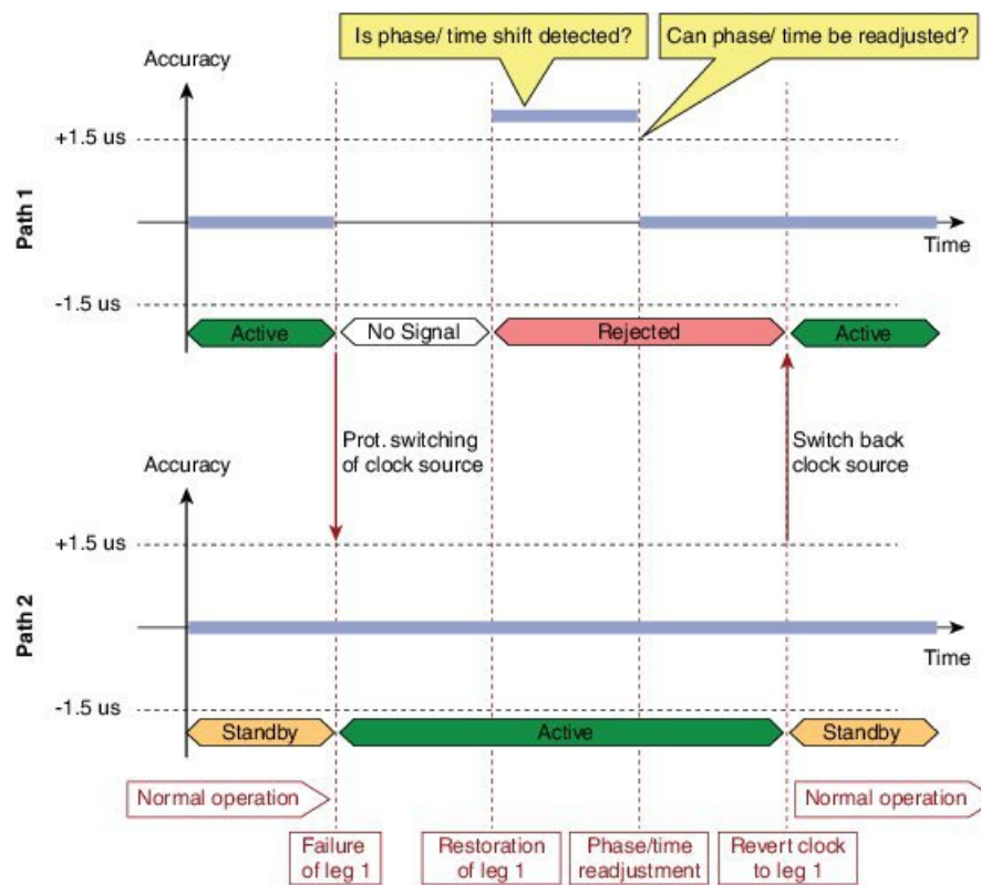
Figure 22: 1588v2 Phase Asymmetry Correction
