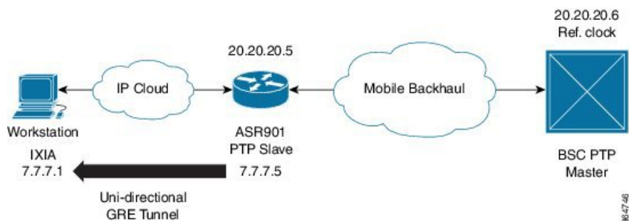
Figure 57: Topology: Unidirectional Tunnel with Slave Device
