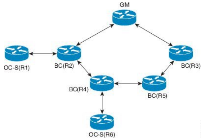
Figure 19: PTP Topology in Multicast Mode
