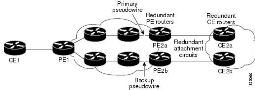
Figure 15: Configuring Redundant Pseudowires
