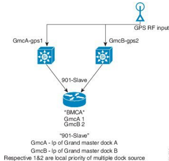
Figure 18: Sample IEEEV2 BMCA Topology
