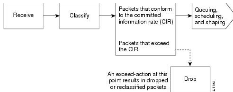
Figure 34: Policing of Classified Packets
