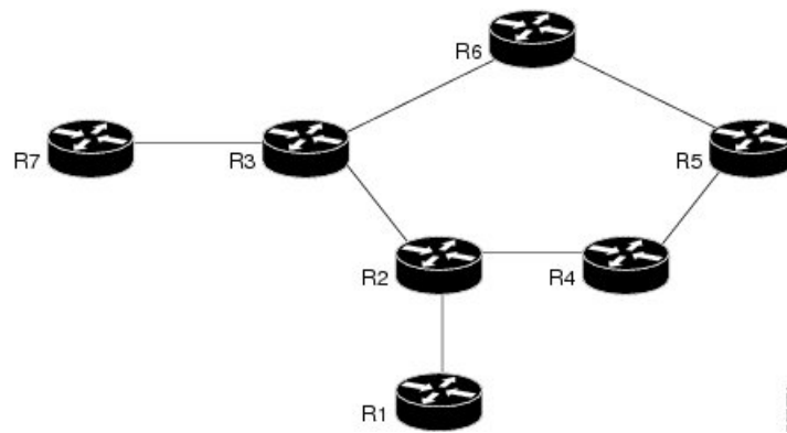
Figure 40: Remote LFA-FRR Link Protection
