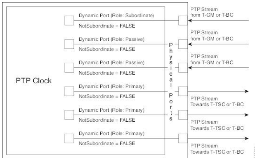
Figure 26: Boundary Clock
