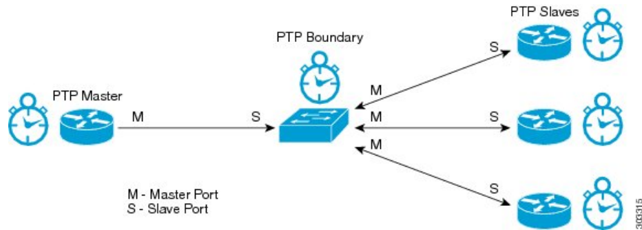
Figure 21: PTP Boundary Clock
