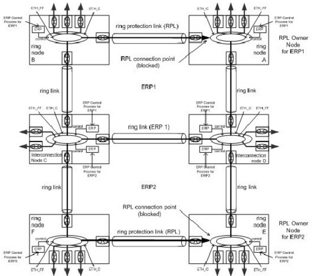
Figure 54: Multiple-Rings Topology
