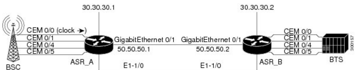
Figure 17: TDM over MPLS Configuration
