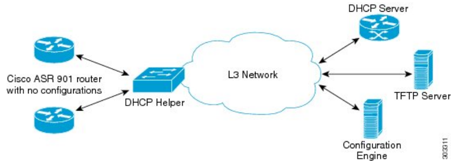
Figure 1: Zero-touch Deployment
