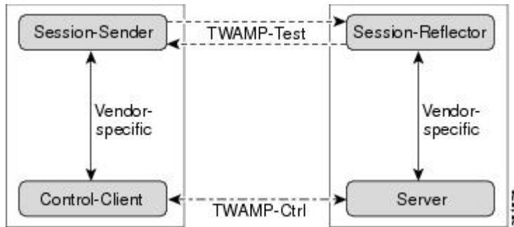
Figure 29: TWAMP Architecture
