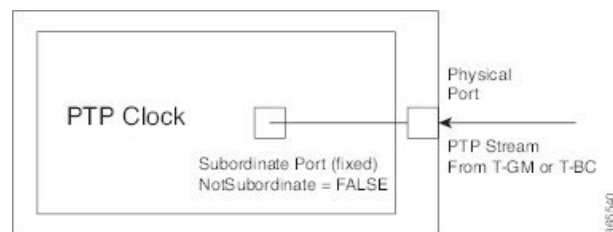
Figure 25: Ordinary Clock As Slave Clock (T-TSC)
