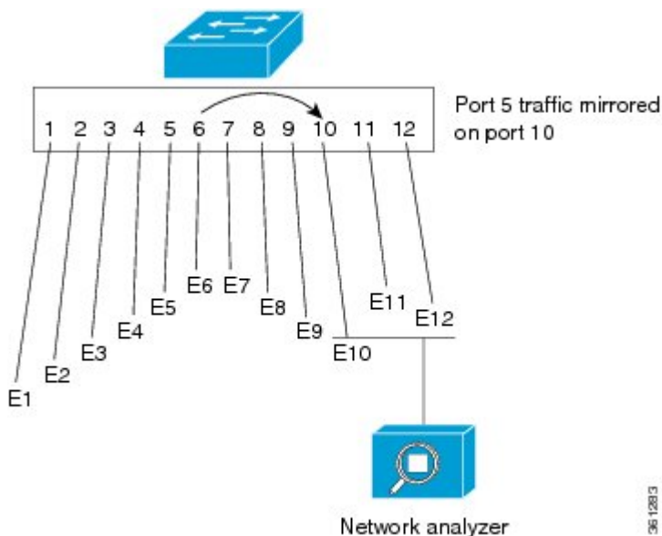
Figure 42: Example of Local SPAN Configuration
