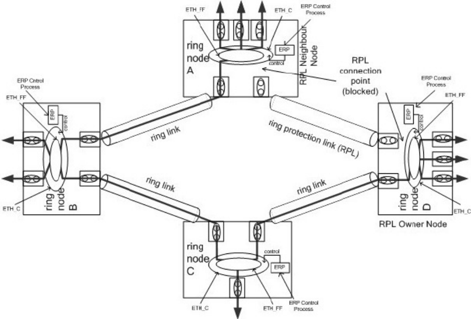
Figure 53: Single-Ring Topology
