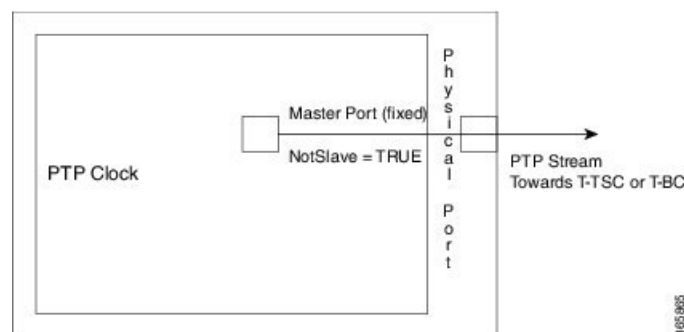
Figure 24: Ordinary Clock As T-GM
