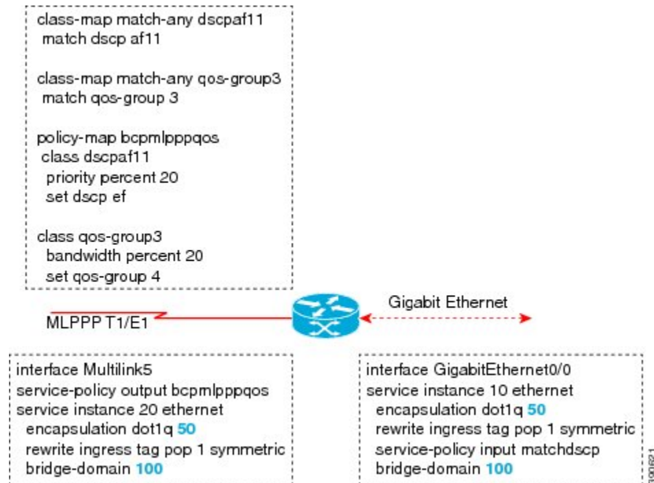
Figure 49: Multilink with QoS
