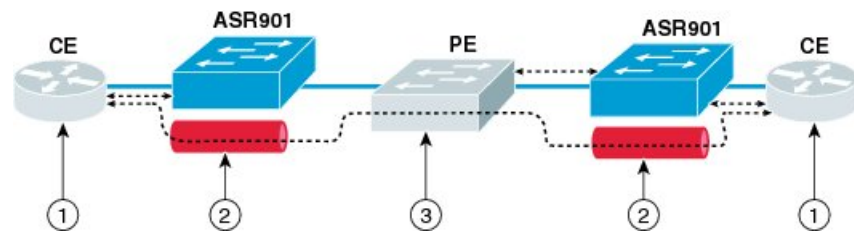
Figure 39: Layer 2 Protocol Tunneling
