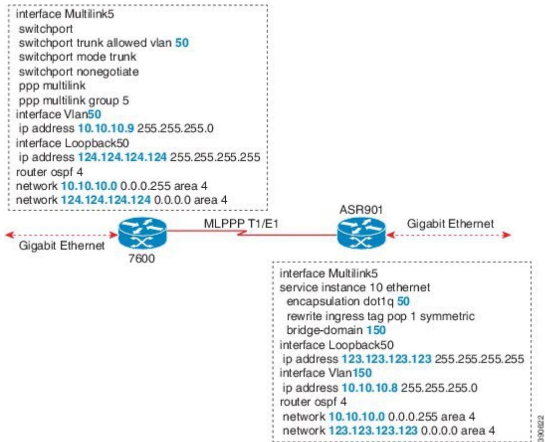
Figure 50: Multilink with Routing on an MLPPP Interface Running BCP
