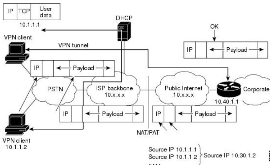
Figure 45: IPsec Packet with UDP Encapsulation
