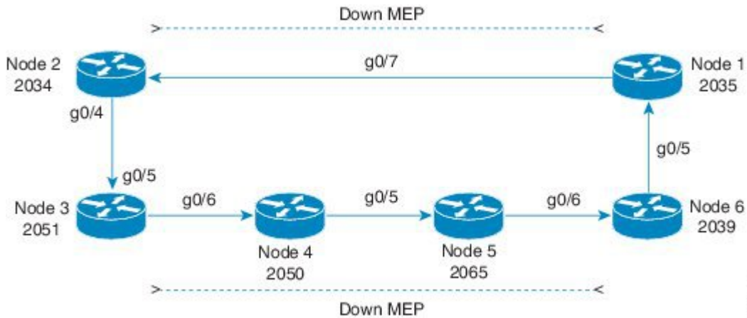
Figure 3: Sample G.8032 Topology with CFM Hardware Offload
