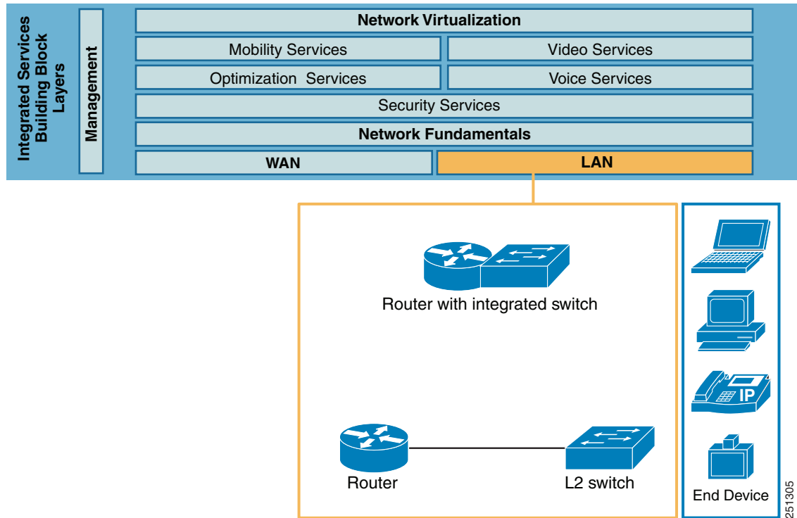
Figure 19 LAN Connectivity Options for Small Branch Office
