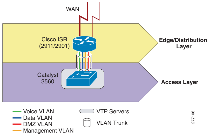
Figure 23 VLAN Trunks and VTP Configuration
