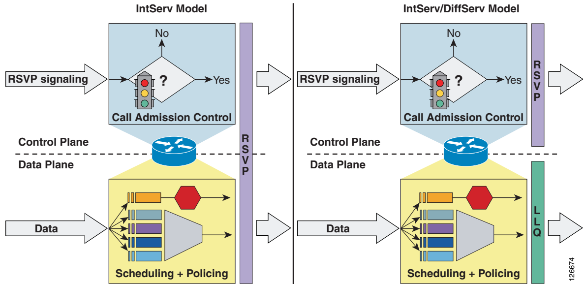
Figure 52 RSVP Operational Models: IntServ and IntServ/DiffServ
