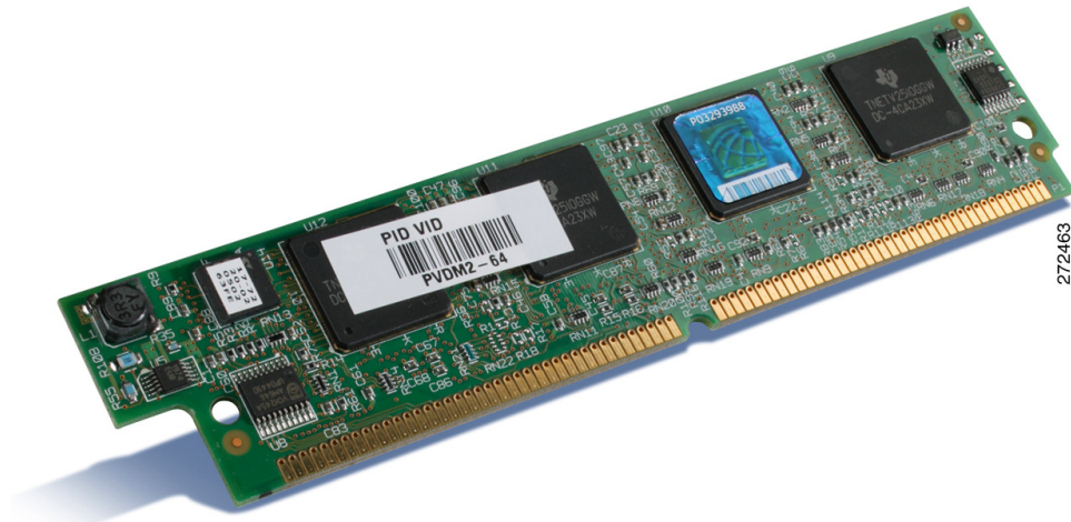
Figure 50 64-Channel Packet Fax/Voice DSP Module
