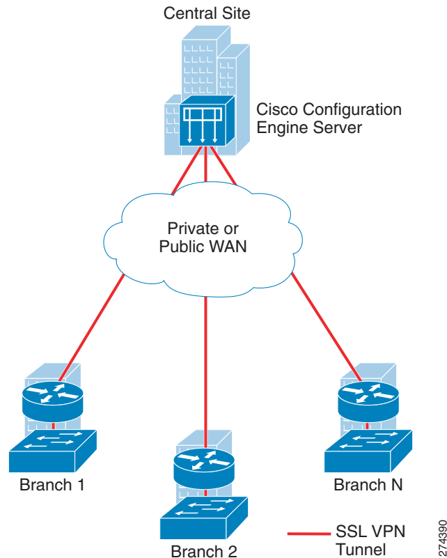
Figure 41 Deployment of CCE in the Streamlined Small Branch Network.
