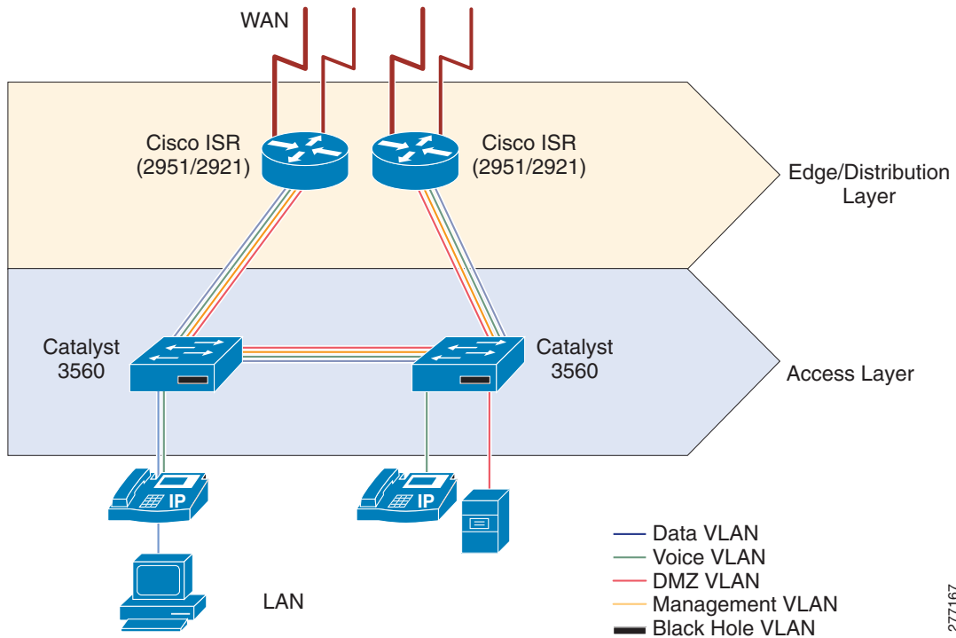
Figure 22 VLAN Design
