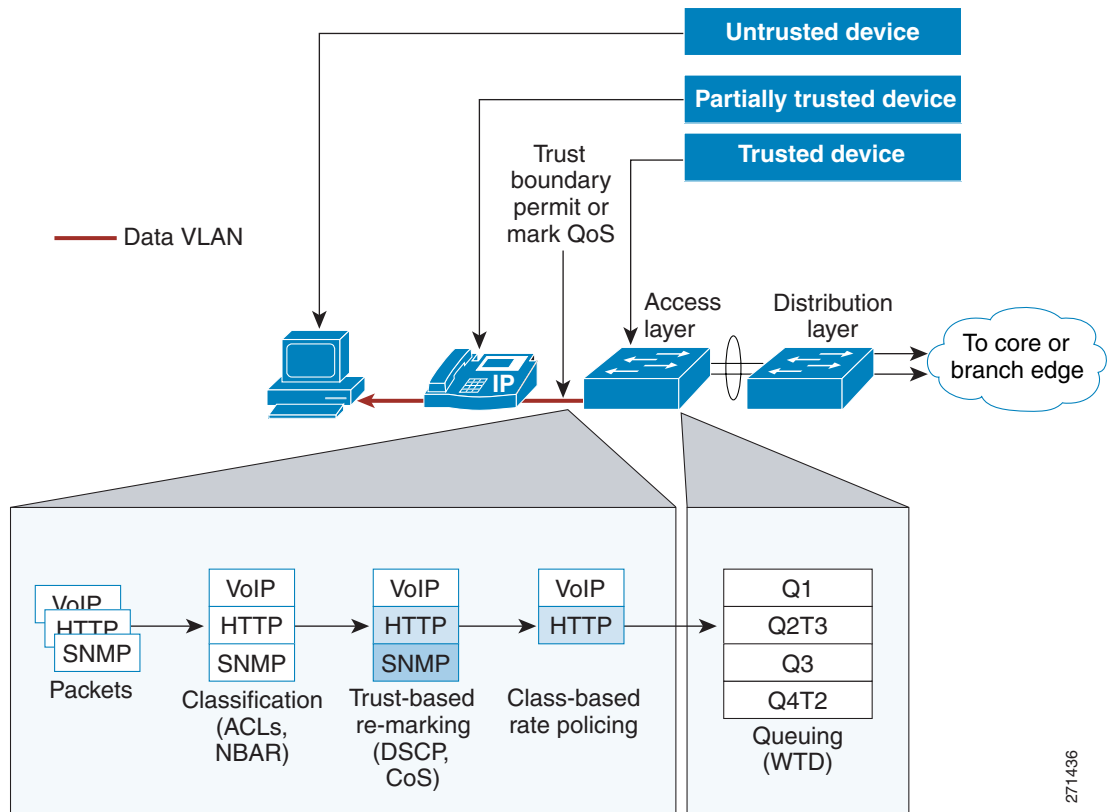
Figure 32 LAN Switch
