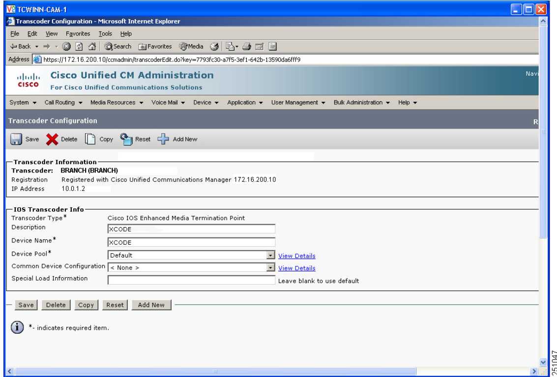
Figure 36 Transcoding Configuration for Cisco Unified SRST Mode
