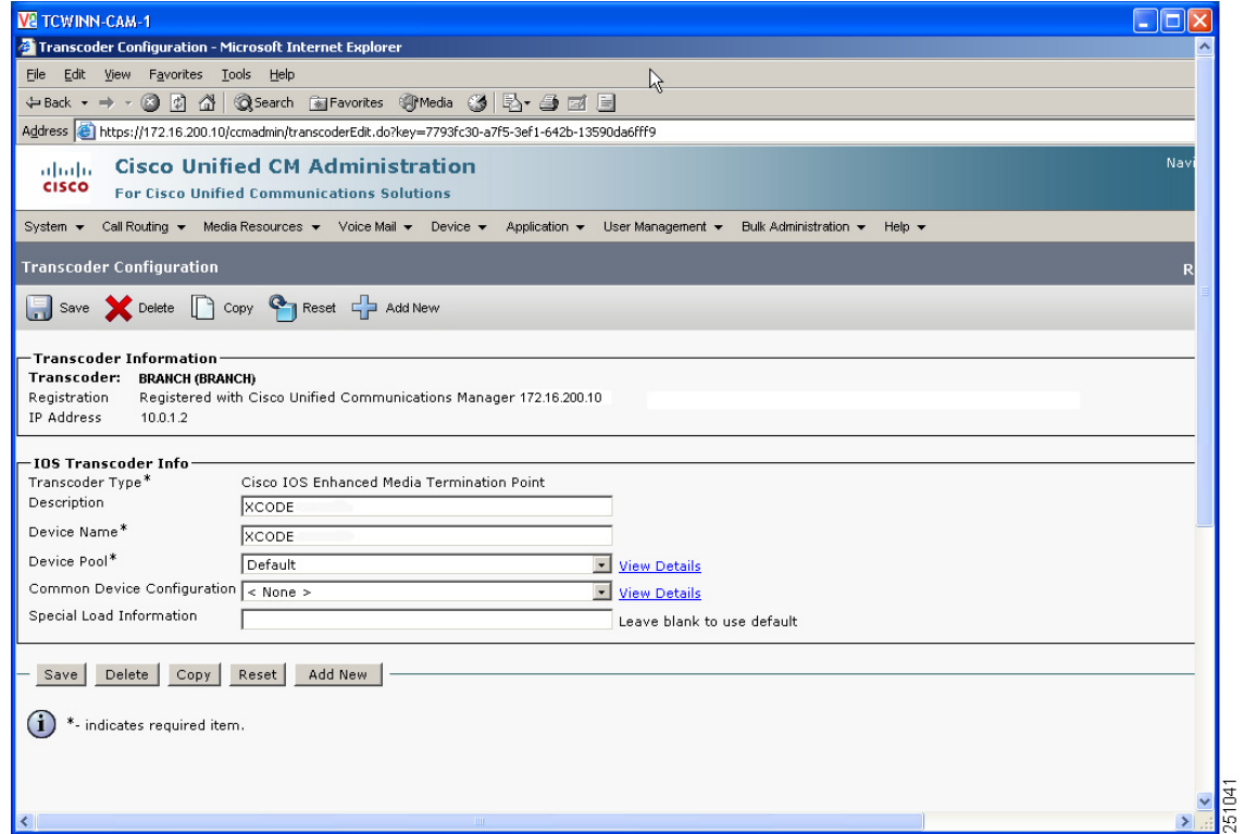
Figure 29 Transcoding Configuration for Cisco Unified SRST Mode
