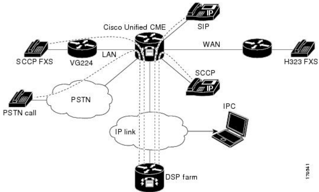
Figure 4: Cisco Unified CME and the DSP Farm on Different Routers
