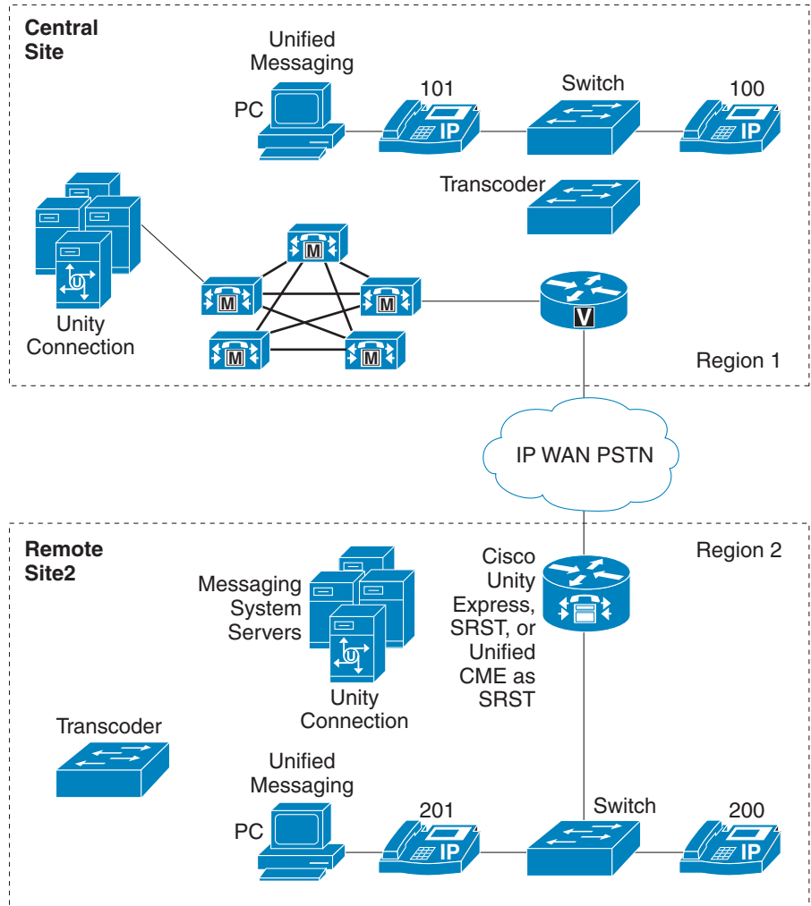
Figure 21-2 Distributed Messaging with Centralized Call Processing
