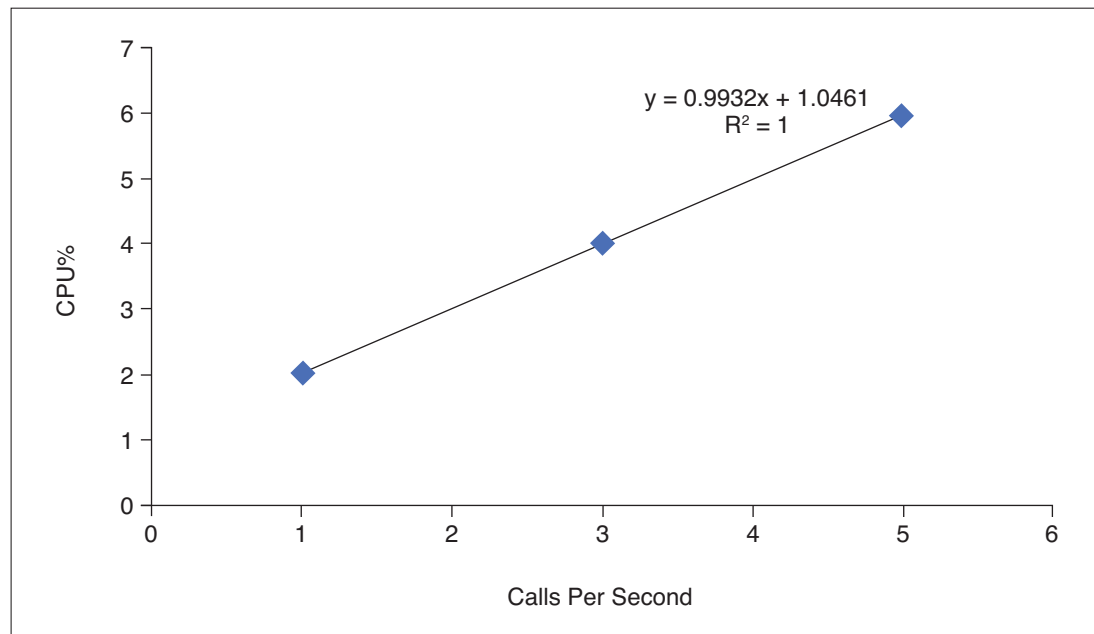
Figure 29-5 CPU Consumption Per Call Setup
