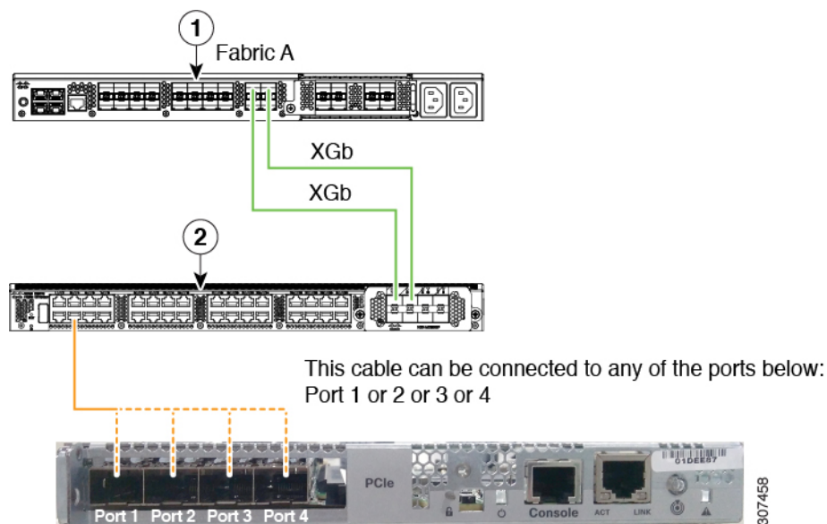
Figure 6: SingleConnect Cabling Configuration with Cisco - Single Cable
