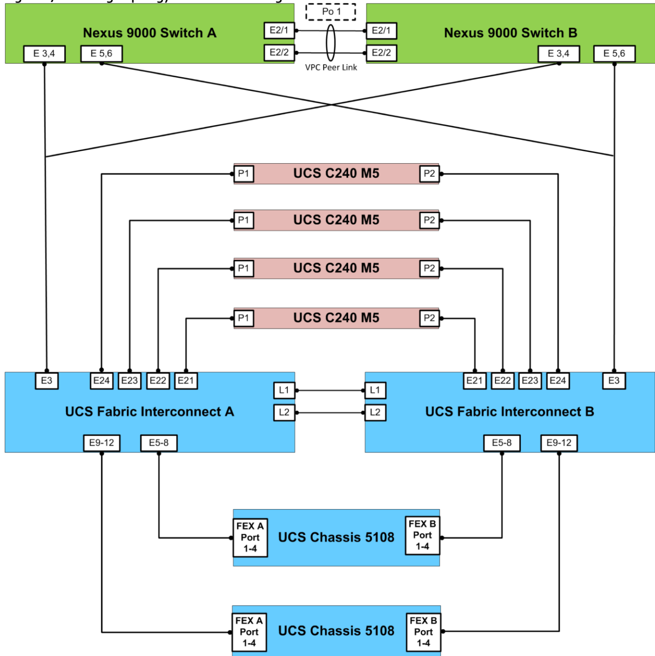
Figure 17 Cabling Topology for Cisco UCS Integrated Infrastructure for SAP HANA
