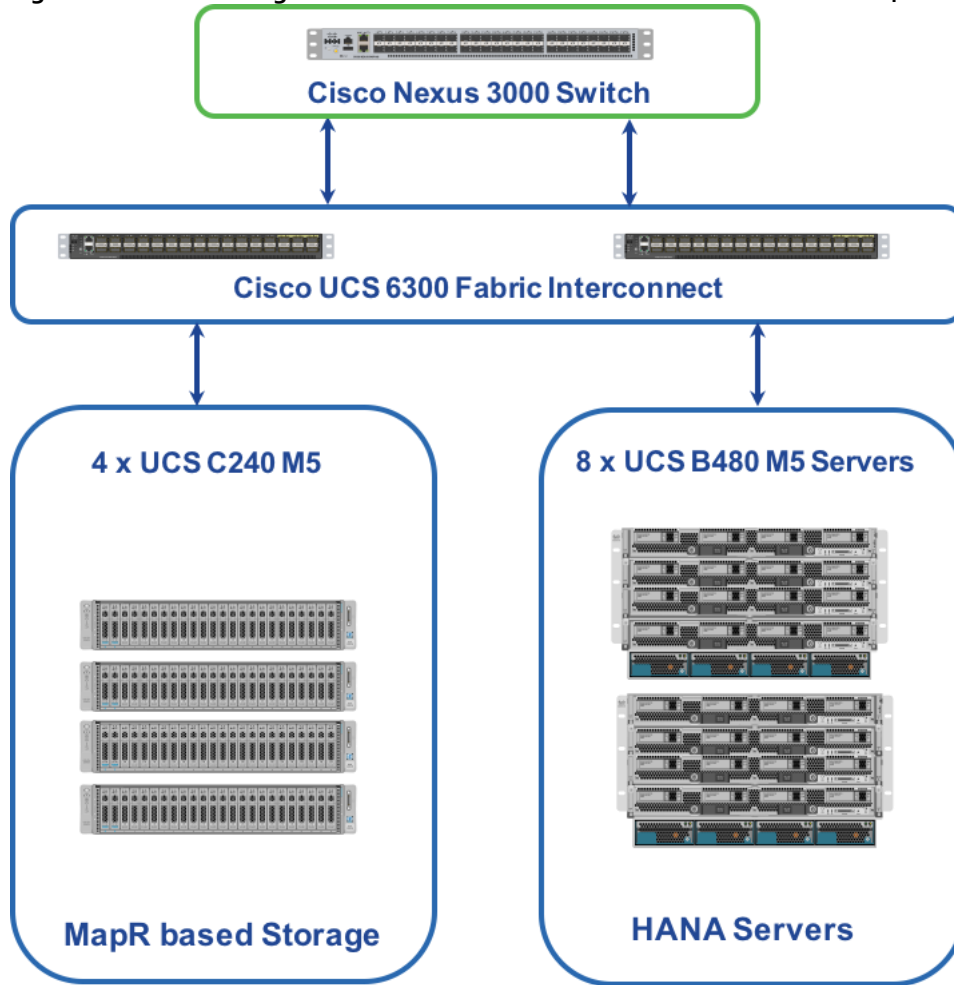
Figure 2 Cisco UCS Integrated Infrastructure for SAP HANA with Cisco UCS B480 M5
