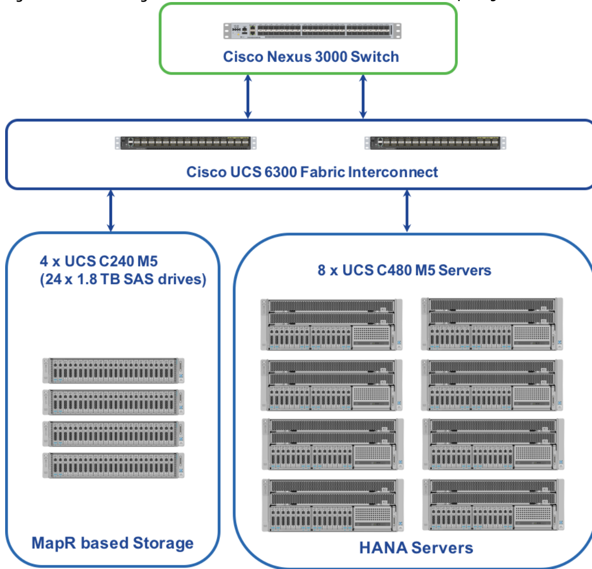
Figure 1 Cisco UCS Integrated Infrastructure for SAP HANA with Cisco UCS C480 M5
