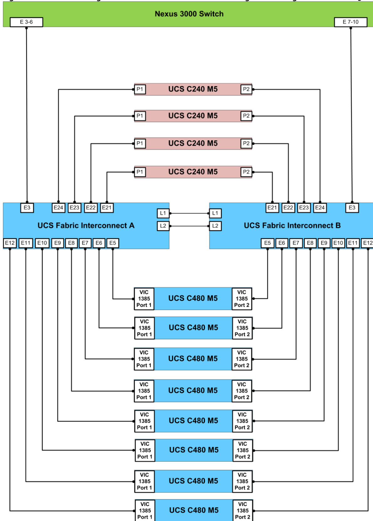
Figure 16 Cisco UCS Integrated Infrastructure for SAP HANA configuration using the Cisco Nexus 3000
