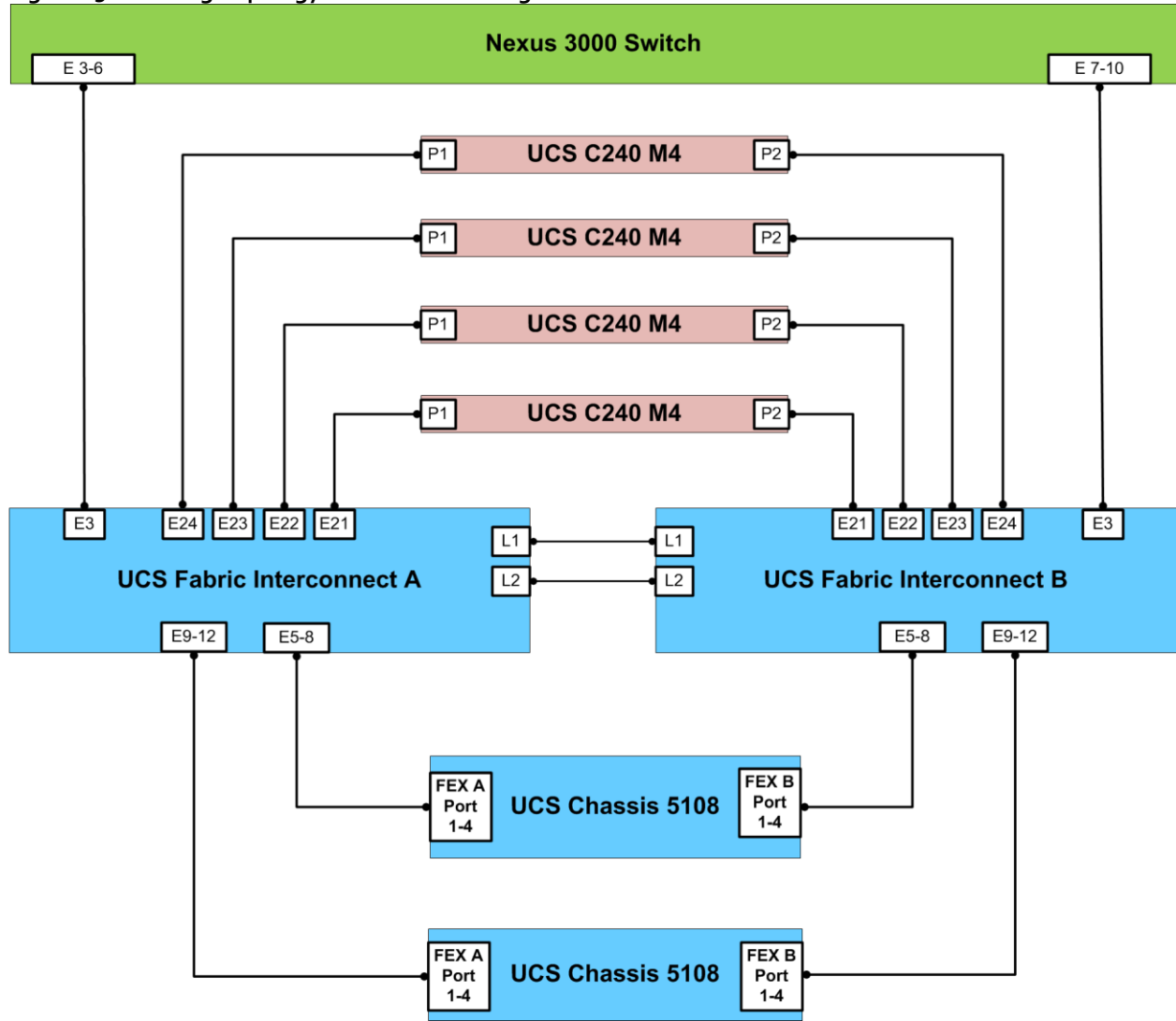
Figure 15 Cabling Topology for Cisco UCS Integrated Infrastructure for SAP HANA
