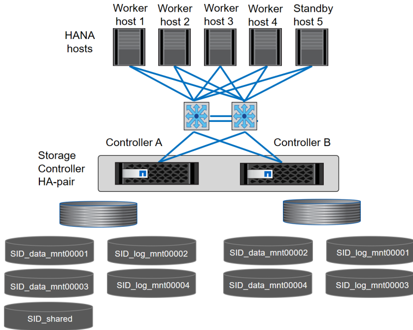
Figure 41 Volume Layout for SAP HANA Multiple-Host Systems
