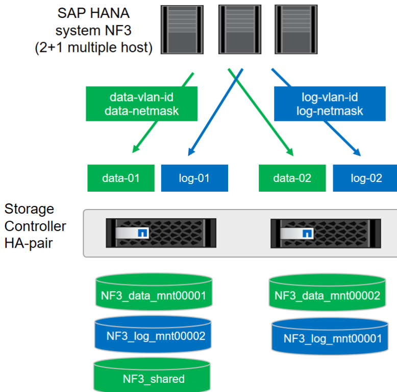
Figure 42 Configuration Example for SAP HANA Multiple-Host Systems
