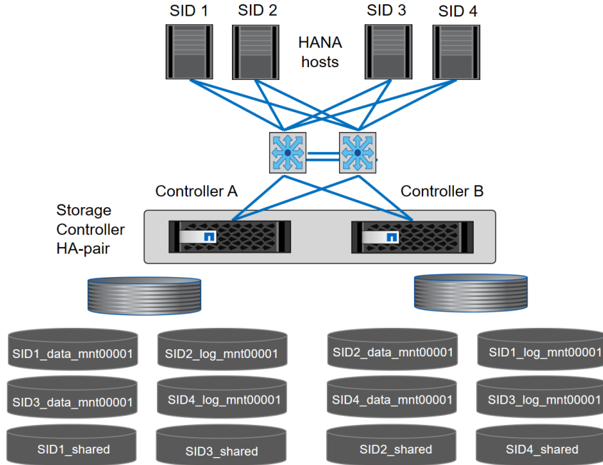
Figure 39 Volume Layout for SAP HANA Multiple Single-Host Systems
