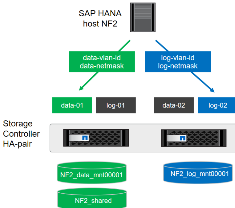
Figure 40 Configuration Example for a SAP HANA Single-Host System
