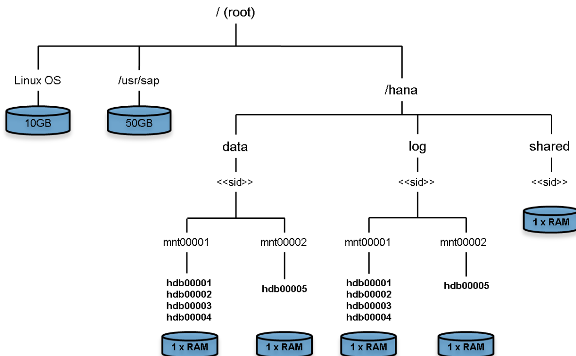
Figure 11 File System Layout for 2 Node Scale-Out System
