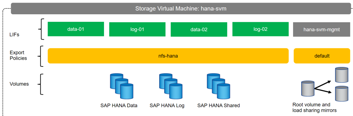
Figure 37 Overview of SAP HANA SVM Components
