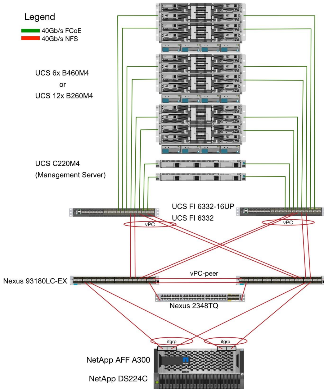
Figure 1 FlexPod Datacenter Reference Architecture for SAP HANA
