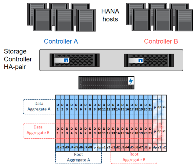
Figure 34 Disk Partitioning ADPv2
