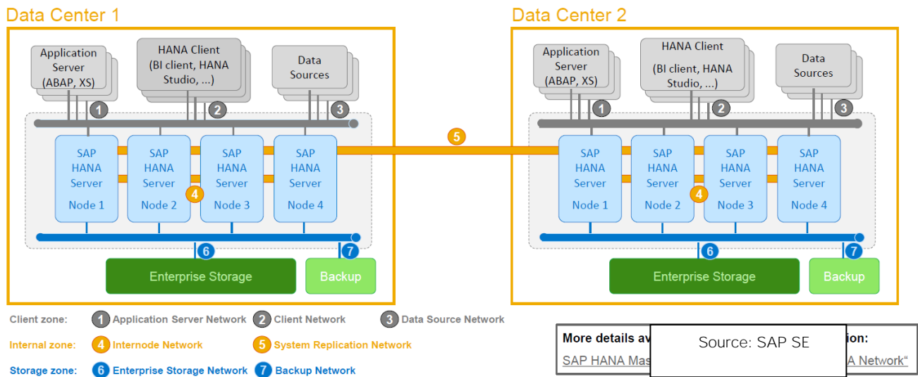
Figure 10 High-Level SAP HANA Network Overview High-Level SAP HANA Network Overview
