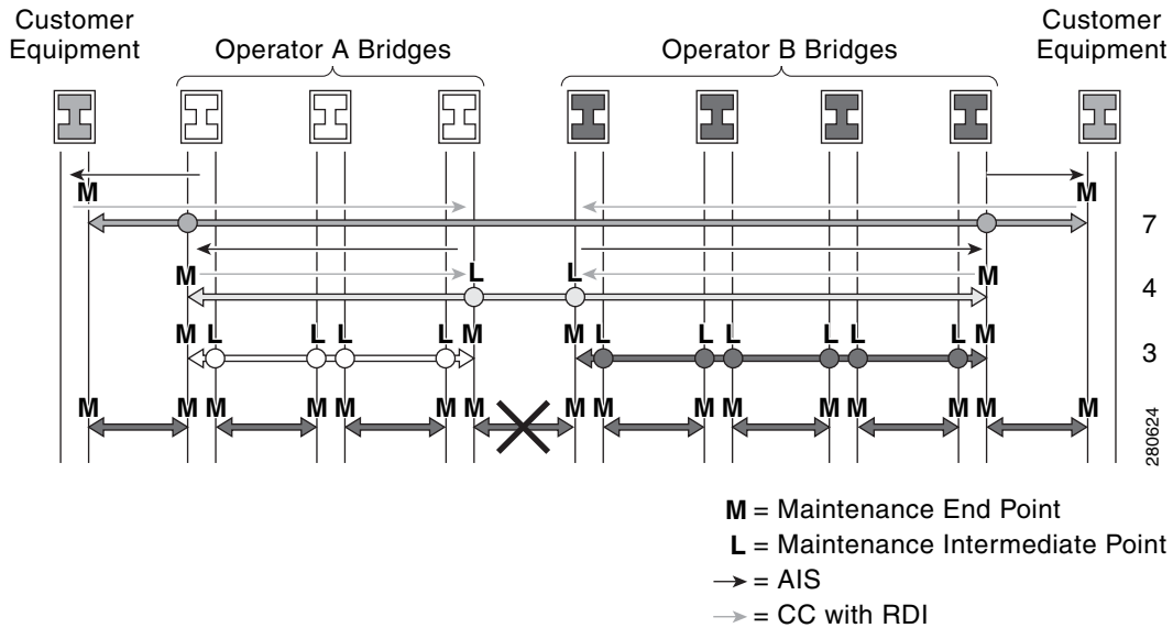
Figure 69-1 Generating and Propagating AIS Messages Upon a Defect (Link Fail)
