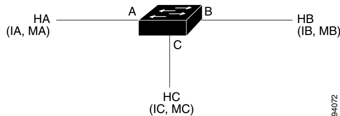
Figure 52-1 ARP Cache Poisoning
