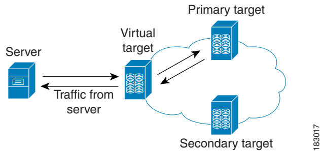
Figure 21-1 Target Virtualization
