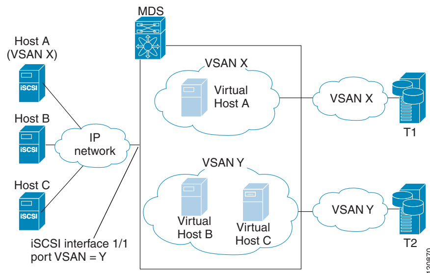
Figure 40-20 VSAN Membership for iSCSI Interfaces
