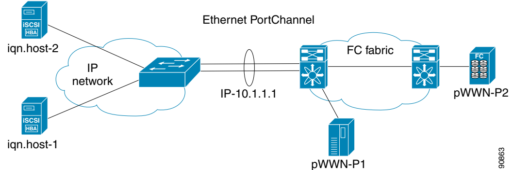
Figure 40-16 Ethernet PortChannel-Based iSCSI High Availability
