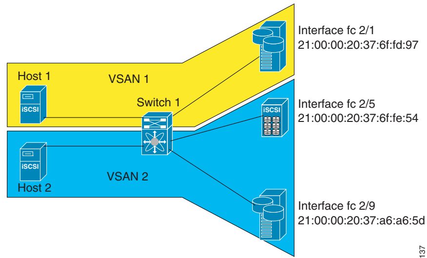
Figure 40-23 Target Storage Device with LUN Mapping
