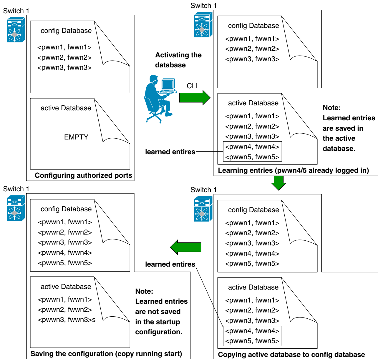
Figure 36-1 Port Security Database Scenarios
