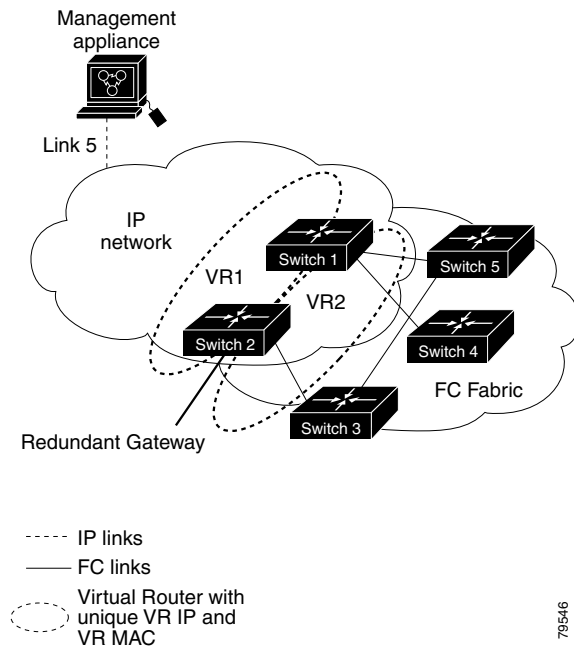
Figure 41-4 Redundant Gateway
