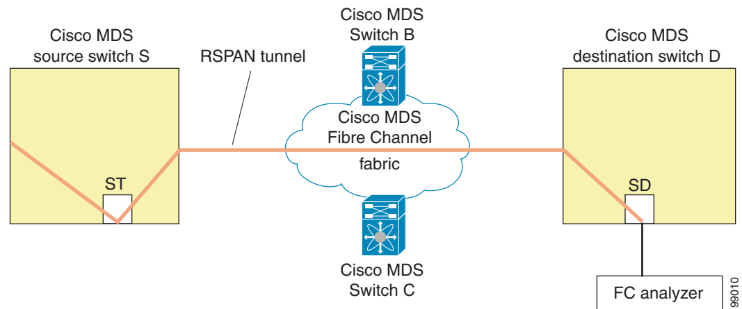
Figure 55-16 RSPAN Scenario with One Source Switch, One Destination Switch, and One Tunnel
