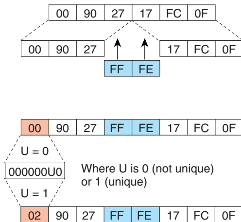
Figure 44-2 Interface Identifier Format
