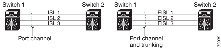
Figure 9-3 PortChanneling and Trunking
