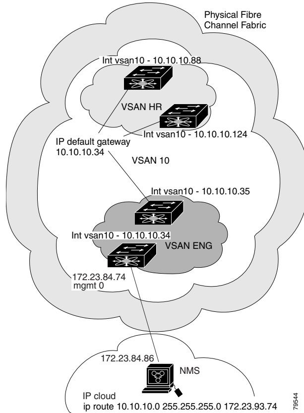
Figure 41-5 Overlay VSAN Configuration Example
