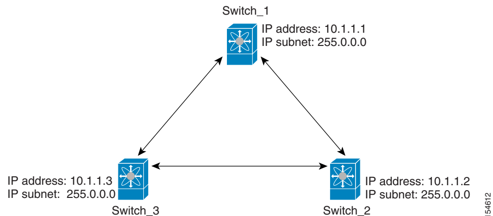
Figure 41-7 IPFC Example Network
