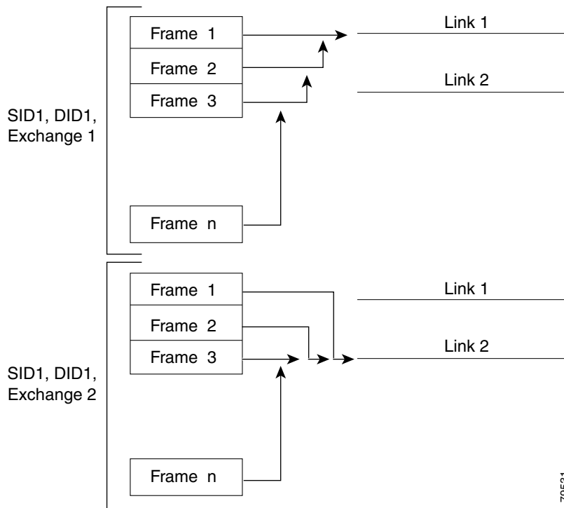
Figure 9-5 SID1, DID1, and Exchange-Based Load Balancing
