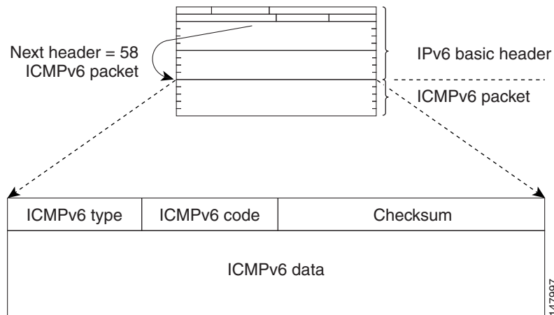
Figure 44-6 IPv6 ICMP Packet Header Format
