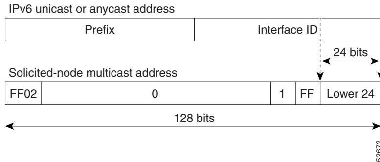
Figure 44-5 IPv6 Solicited-Node Multicast Address Format
