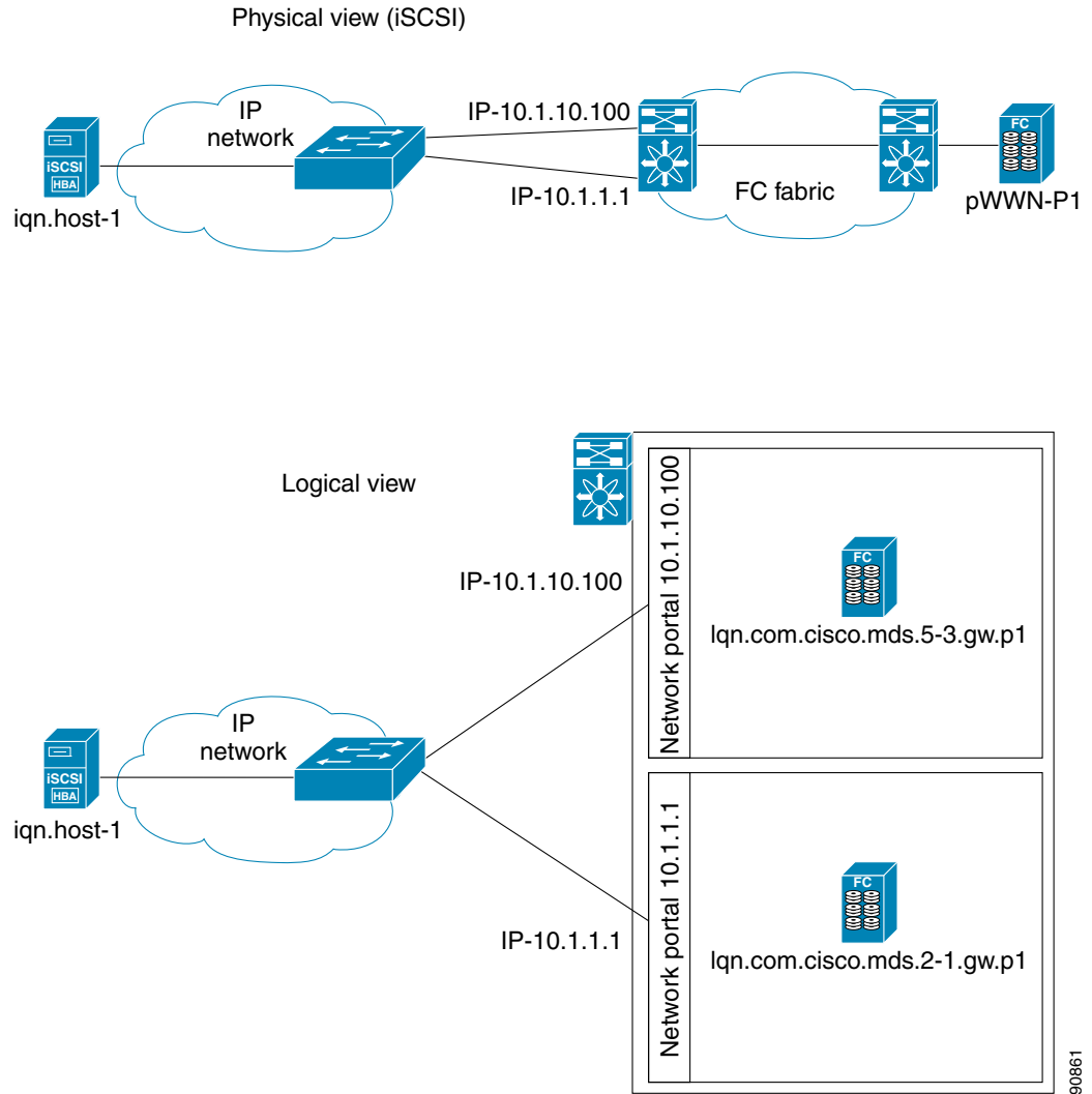
Figure 40-14 Multiple Gigabit Ethernet Interfaces in the Same IP Network
