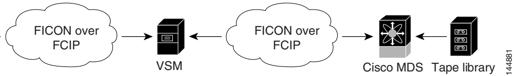
Figure 24-6 Host Accessing Standalone IBM-VTS (Virtual Tape Server) /STK-VSM (Virtual Shared Memory)
