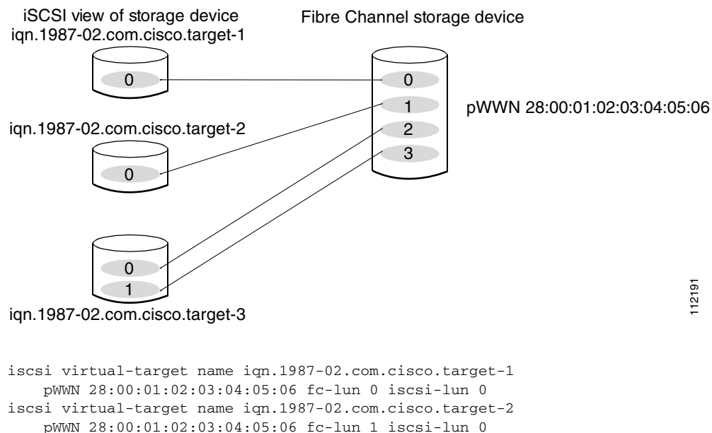
Figure 40-19 Mapping LUNs to Multiple iSCSI Node Names
