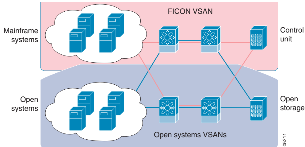
Figure 24-1 Shared System Storage Network
