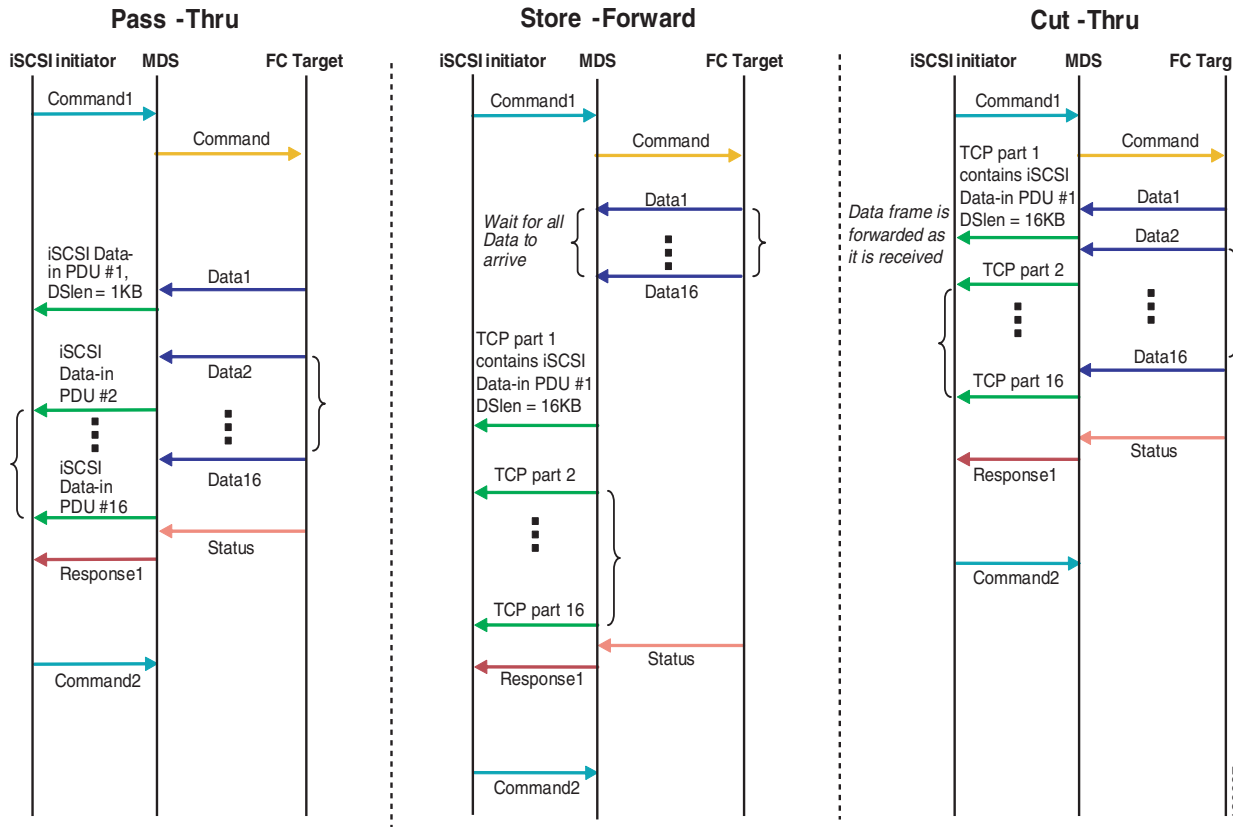
Figure 40-9 iSCSI Routing Modes
