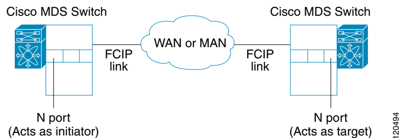
Figure 39-2 N Port Tuning Configuration Physical Example
