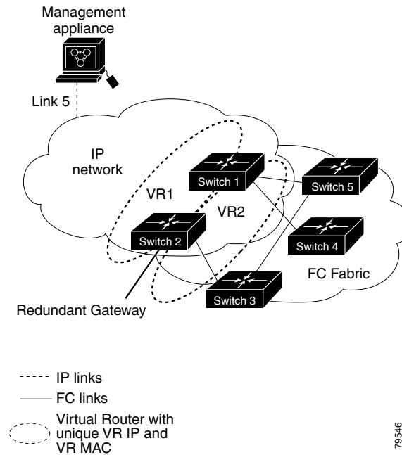
Figure 41-4 Redundant Gateway
