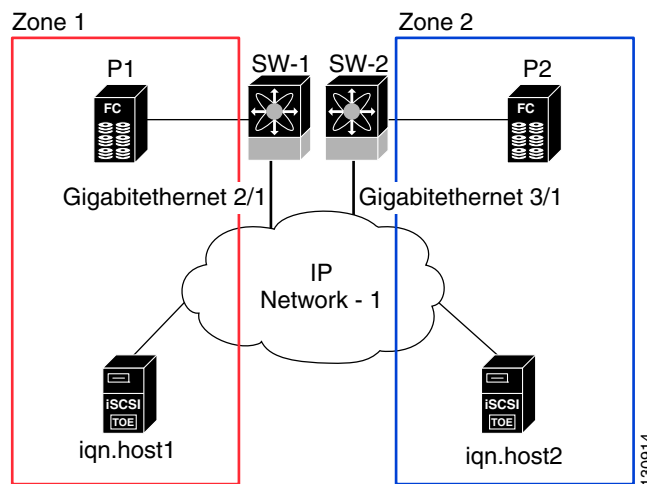
Figure 40-21 Using iSNS Servers in the Cisco MDS Environment
