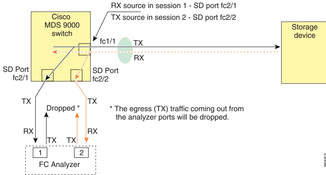
Figure 55-5 Fibre Channel Analyzer Using SPAN
