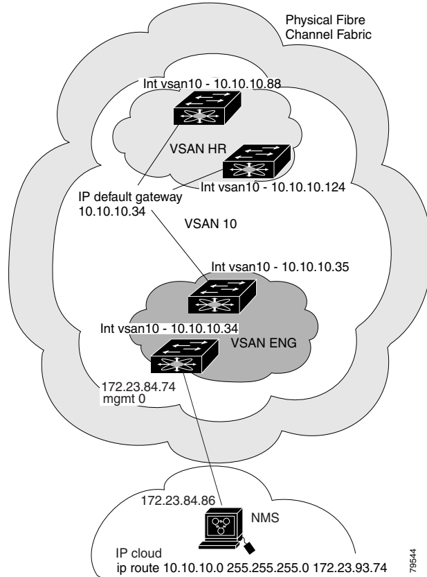
Figure 41-5 Overlay VSAN Configuration Example
