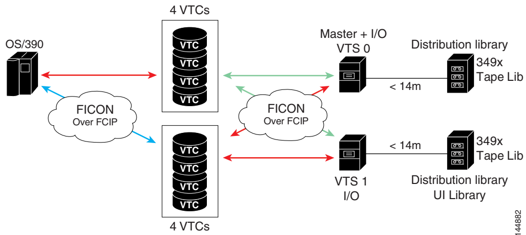
Figure 24-7 Host Accessing Peer-to-Peer VTS (Virtual Tape Server)
