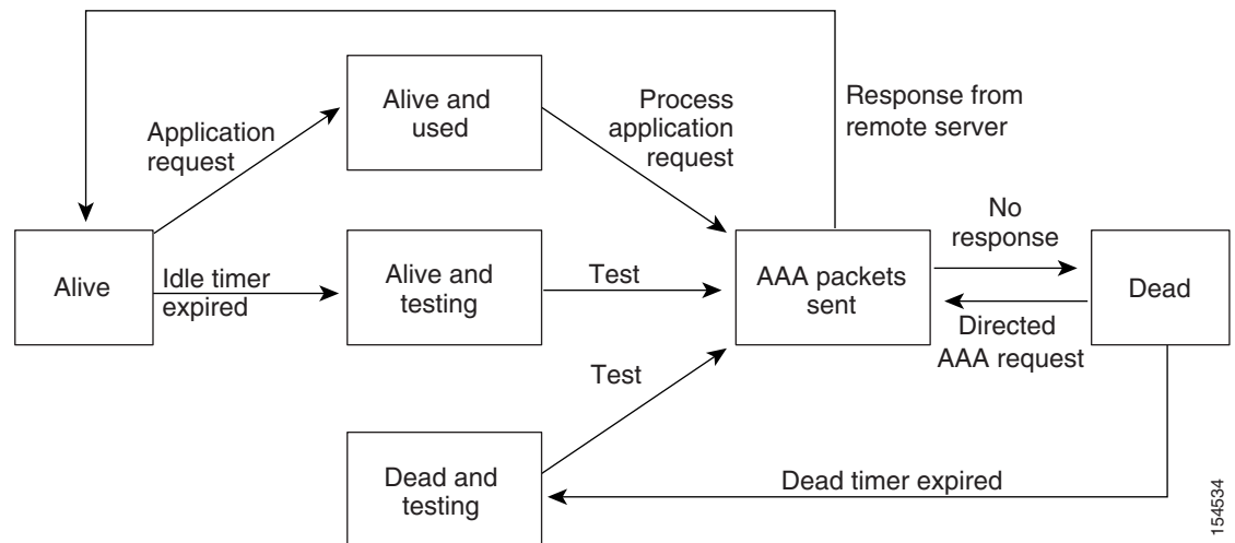
Figure 29-1 AAA Server States
