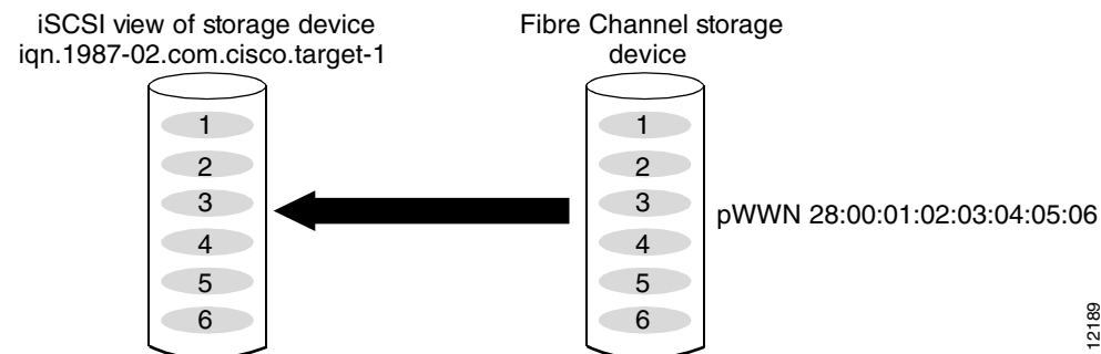
Figure 40-17 Assigning iSCSI Node Names
