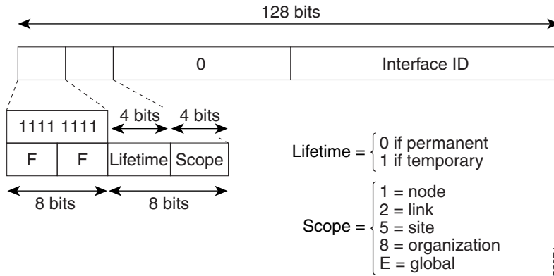
Figure 44-4 IPv6 Multicast Address Format
