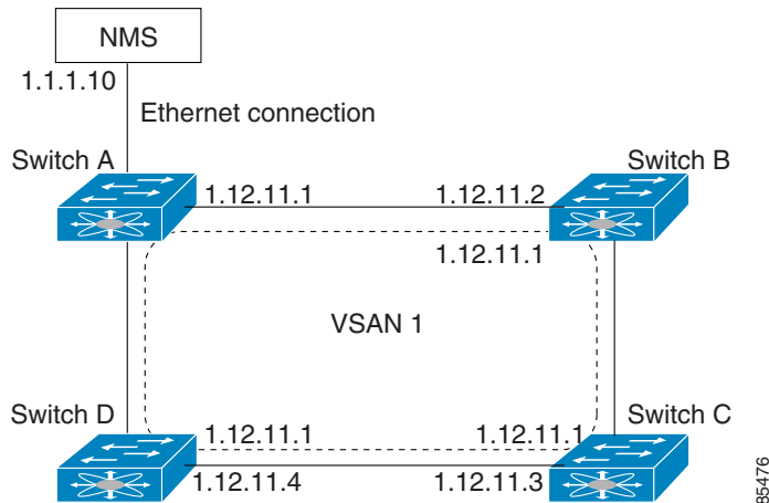
Figure 41-2 Overlay VSAN Functionality
