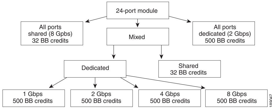
Figure 60-3 BB_Credit Buffer Allocation in 24-Port 8-Gbps Switching Modules
