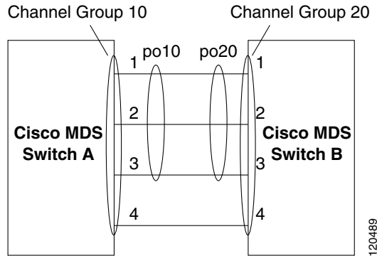
Figure 9-6 Autocreating Channel Groups
