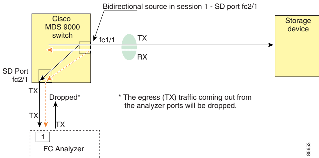
Figure 55-6 Fibre Channel Analyzer Using a Single SD Port
