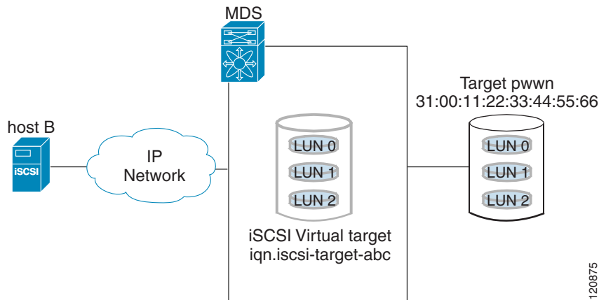
Figure 40-6 Statically Mapped iSCSI Targets
