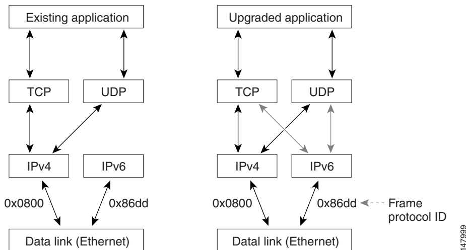
Figure 44-9 Dual IPv4 and IPv6 Protocol Stack Technique
