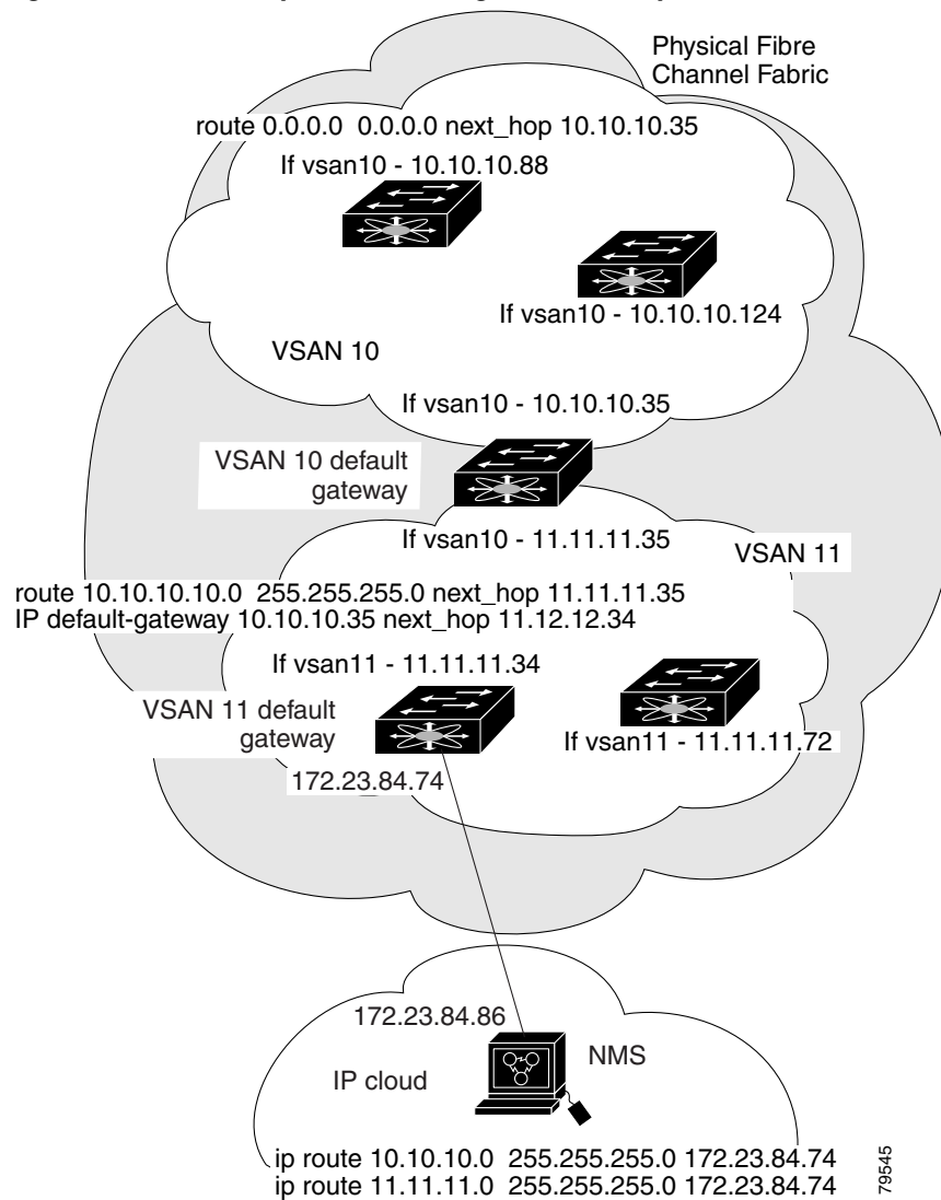
Figure 41-6 Multiple VSAN Configuration Example
