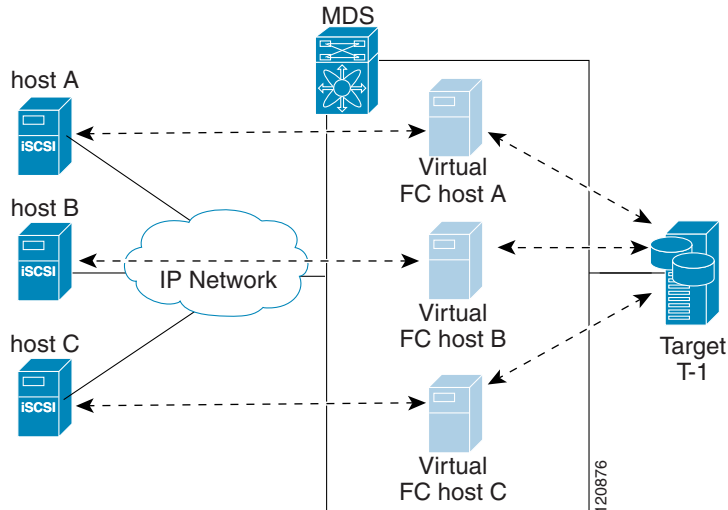
Figure 40-7 Virtual Host HBA Port
