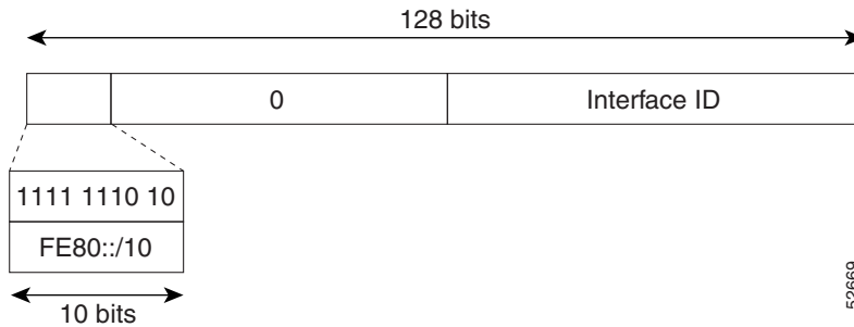
Figure 44-3 Link-Local Address Format
