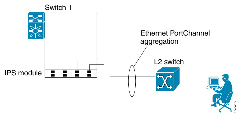
Figure 42-5 Ethernet PortChannel Scenario
