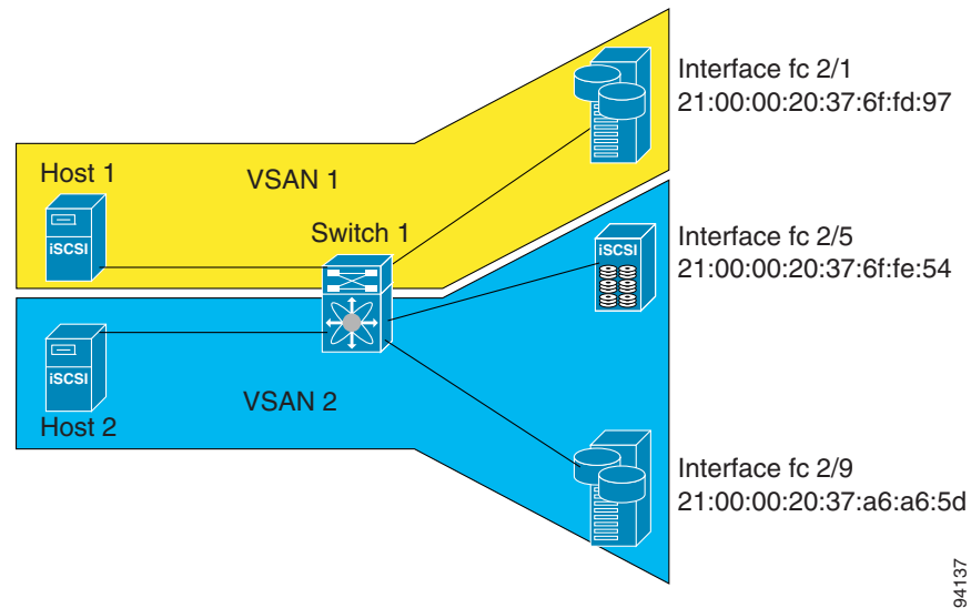
Figure 40-23 Target Storage Device with LUN Mapping
