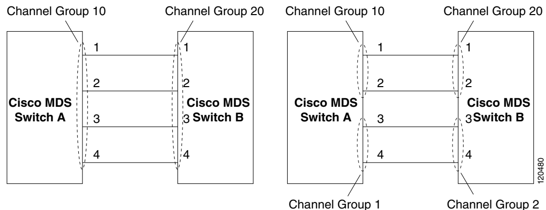
Figure 9-7 Valid PortChannel Configurations
