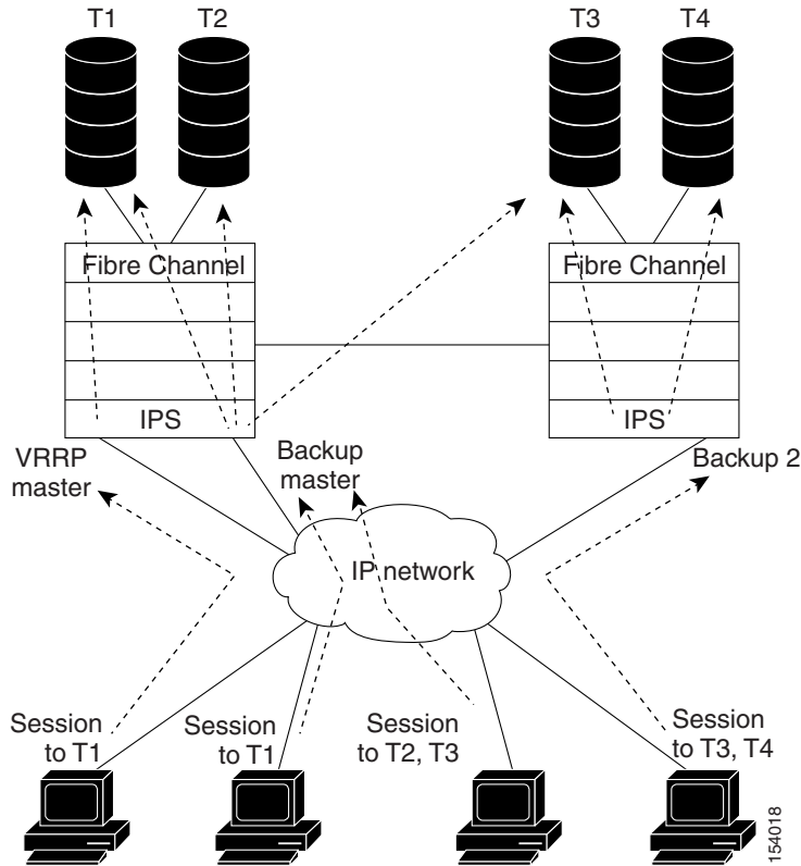
Figure 40-10 iSLB Initiator Load Balancing Example
