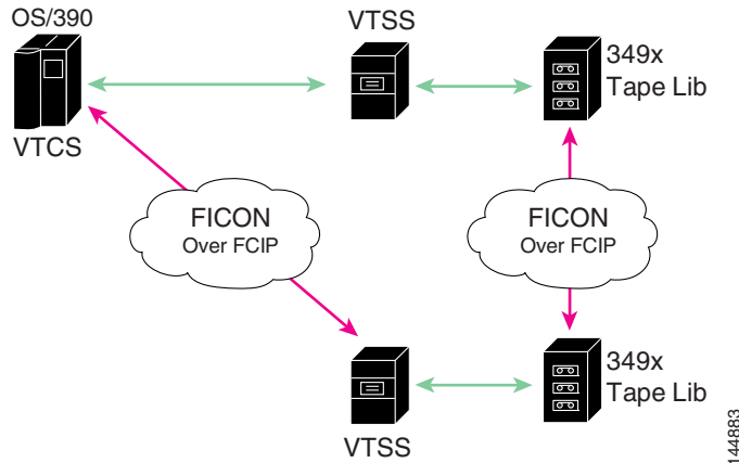
Figure 24-8 Host Accessing Peer-to-Peer VTS (Virtual Tape Server)
