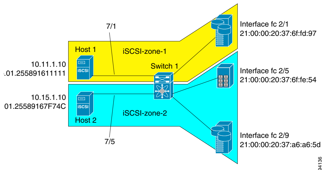
Figure 40-22 iSCSI Transparent Mode Initiator
