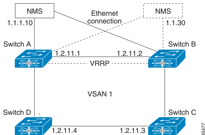
Figure 41-3 VRRP Functionality
