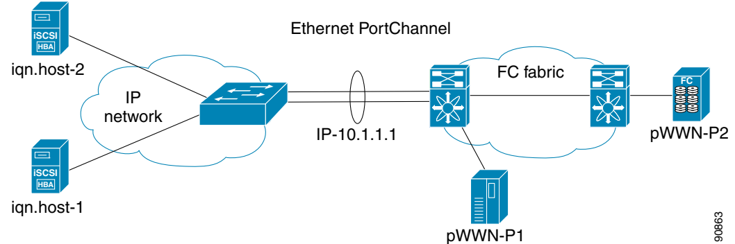
Figure 40-16 Ethernet PortChannel-Based iSCSI High Availability
