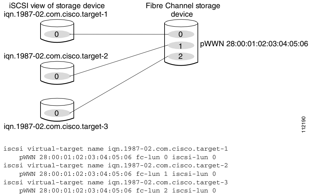
Figure 40-18 Mapping LUNs to an iSCSI Node Name
