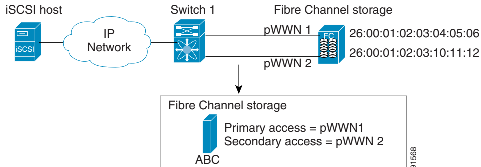
Figure 40-12 Static Target Importing Through Two Fibre Channel Ports
