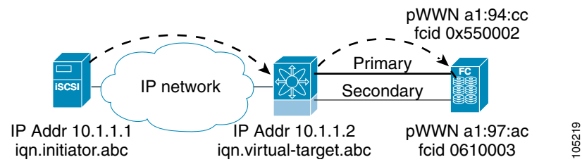
Figure 40-13 Virtual Target with an Active Primary Port
