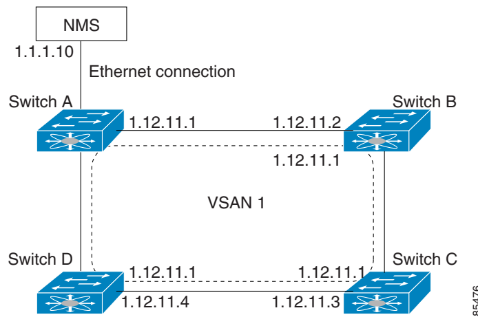
Figure 41-2 Overlay VSAN Functionality
