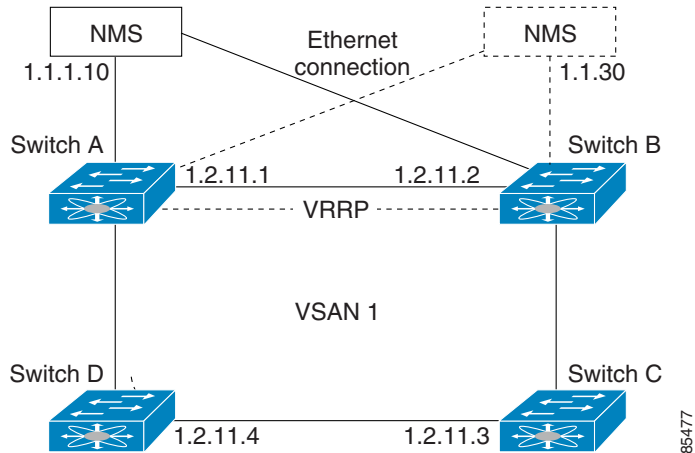
Figure 41-3 VRRP Functionality
