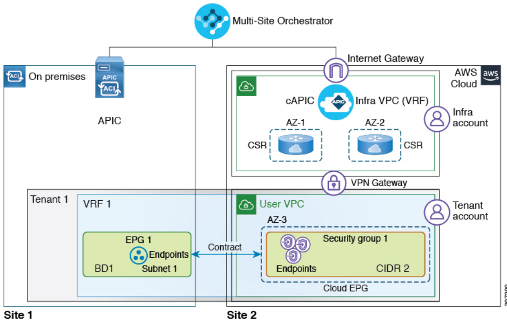
Figure 1: Stretched VRF, On-Premises and AWS
