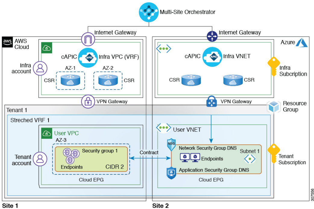
Figure 3: Stretched VRF, Multi-Cloud
