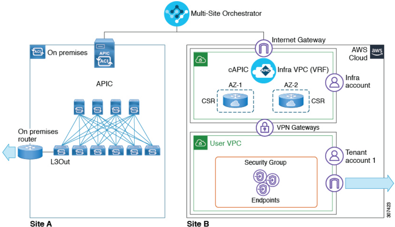
Figure 1: Internet Services for AWS
