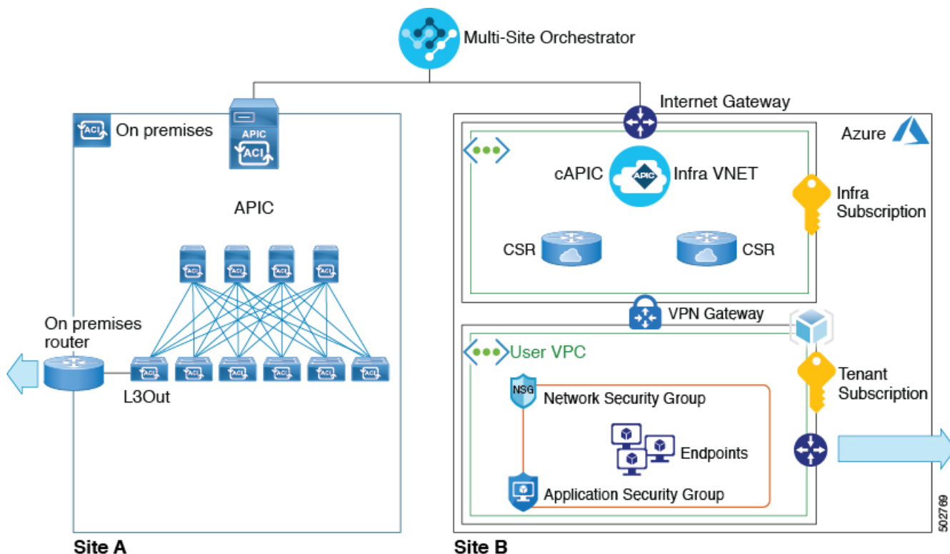
Figure 2: Internet Services for Azure
