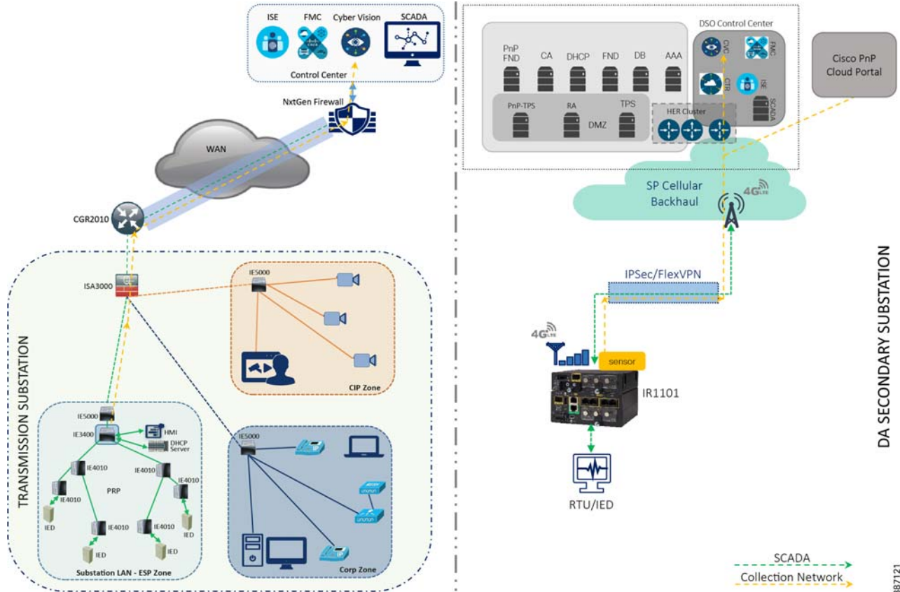
Figure 7 Grid Security Solution Validation Topology
