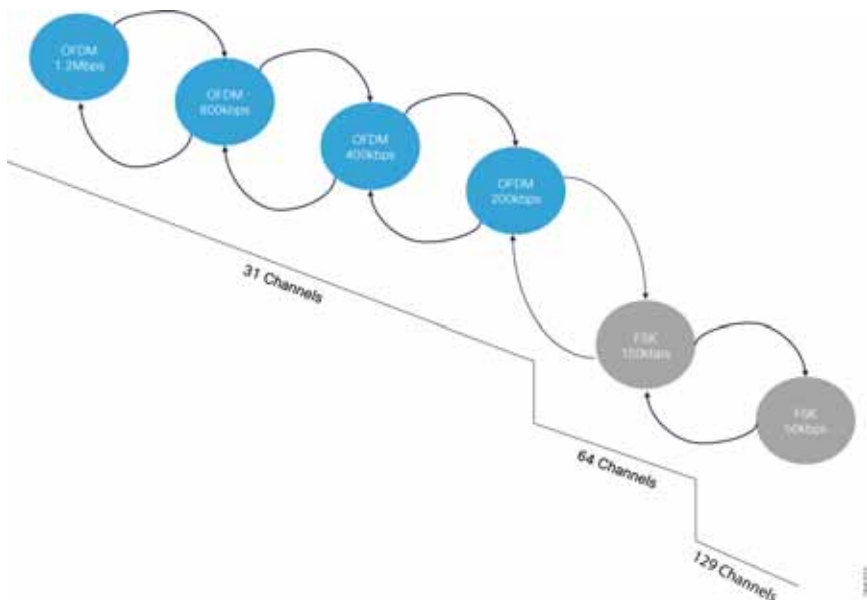
Figure 165 Adaptive Modulation Feature
