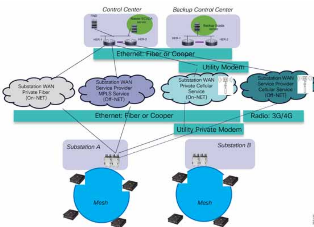
Figure 130 Supported WAN Transport Services
