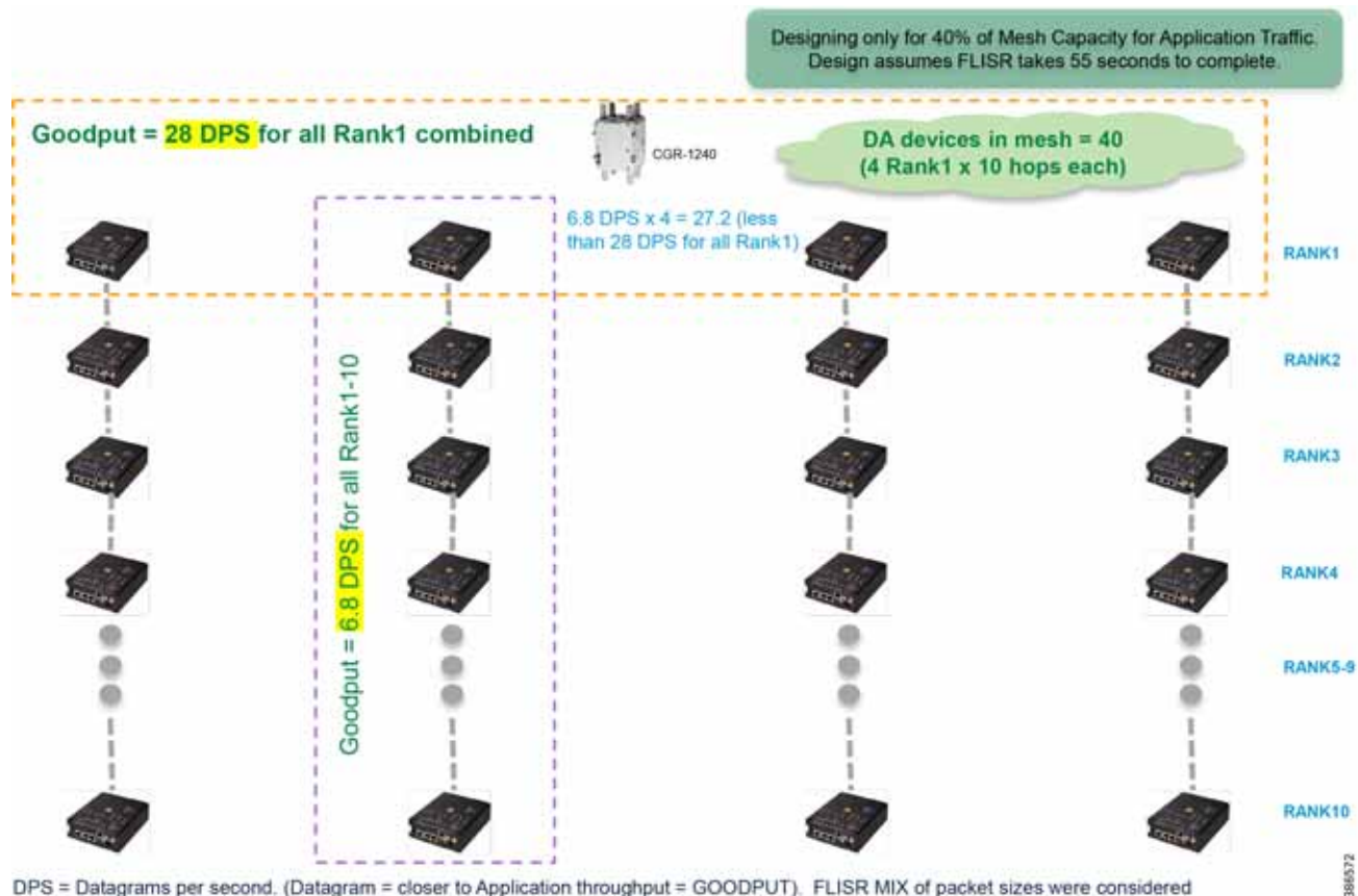
Figure 39 Considering up to 10 nodes per rank1 hierarchy
