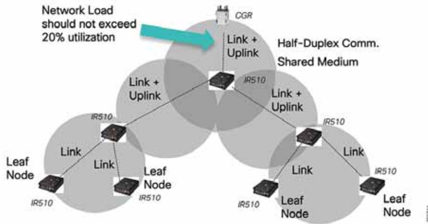
Figure 157 Capacity Planning
