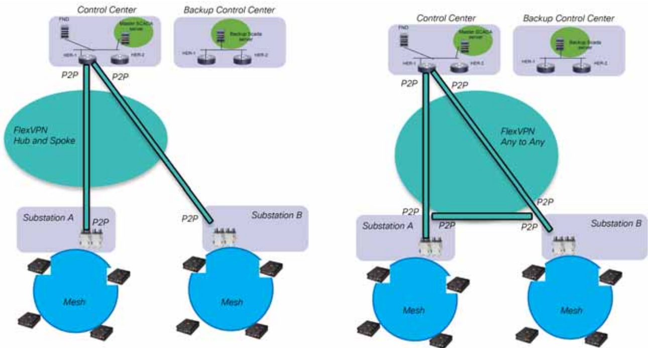
Figure 132 FlexVPN Network Topologies
