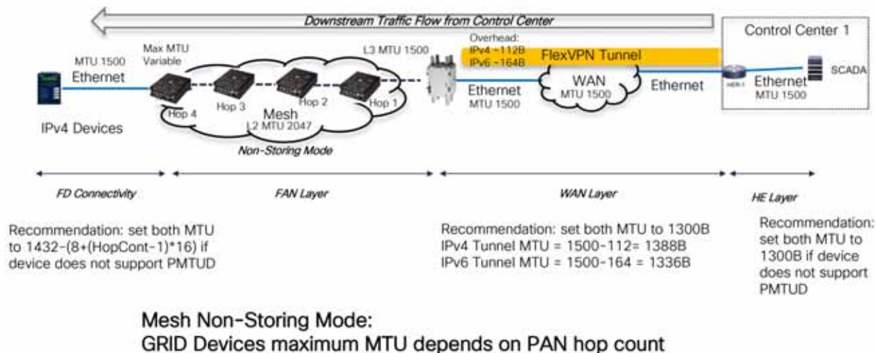
Figure 68 Non-Storing Mode MTU Considerations
