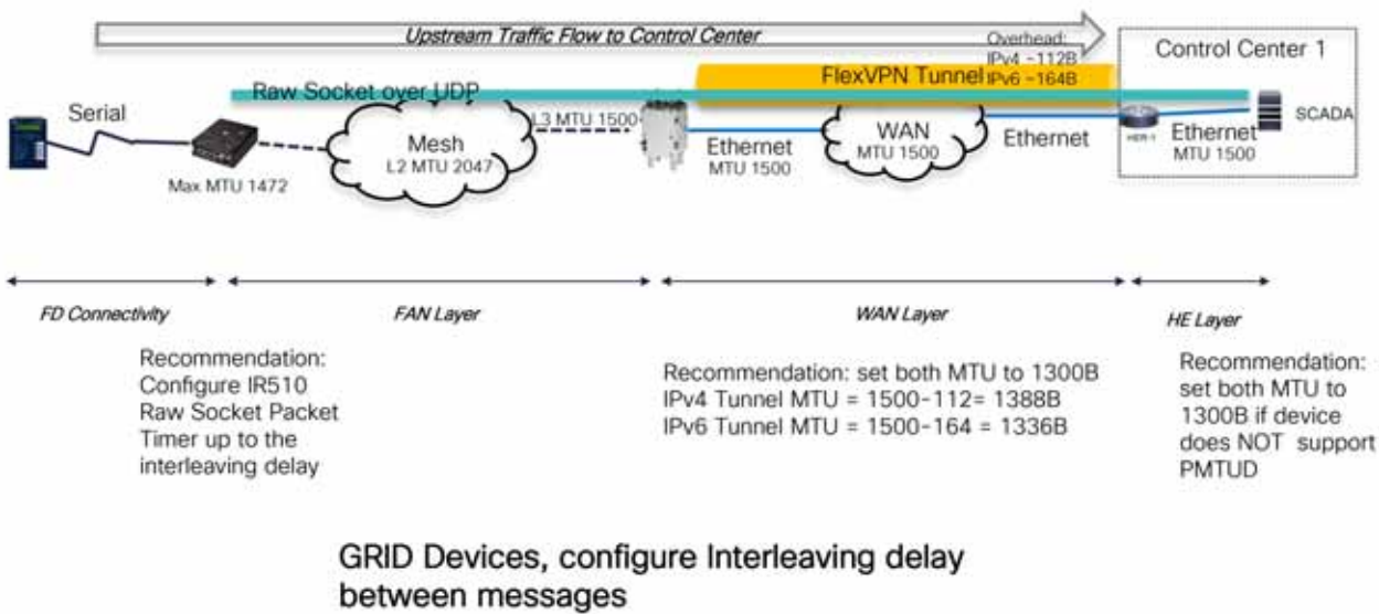
Figure 67 Raw Socket Packet Length for Serial Connectivity
