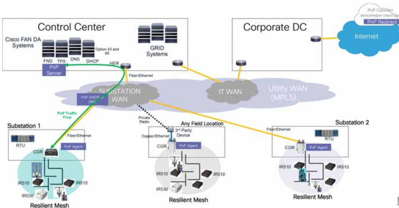
Figure 102 FAR ZTD 2.0 over Ethernet
