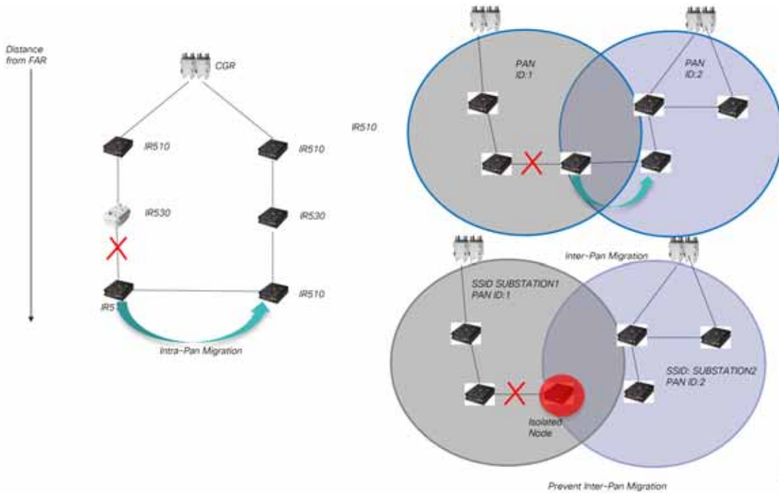
Figure 127 Node Migration
