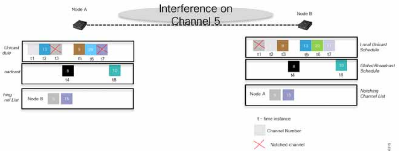
Figure 161 Channel Notching List Feature
