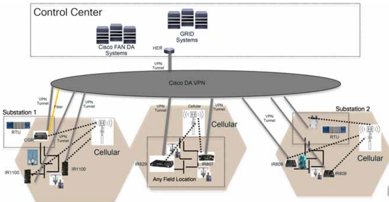
Figure 55 Cellular DA Design
