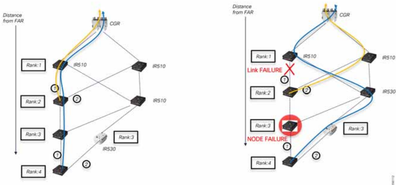
Figure 120 Upstream Link and Node Redundancy: Normal Conditions with Upstream Redundancy and Link & Node Failure
