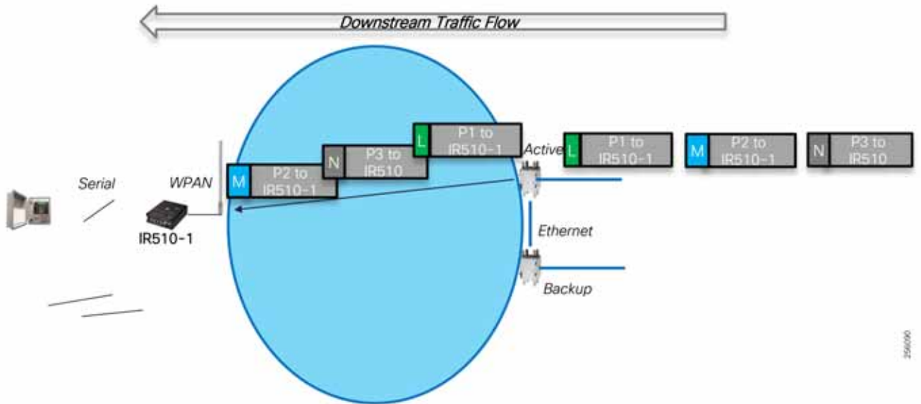
Figure 86 QoS Queuing and Scheduling
