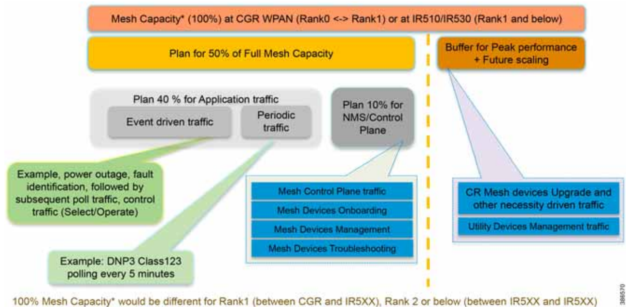
Figure 37 captures a sample mesh capacity allocation for different types of traffic that competes for bandwidth.
