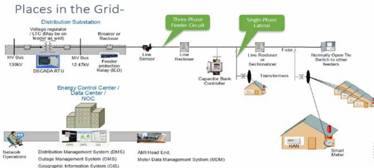
Figure 2 Distribution Feeder
