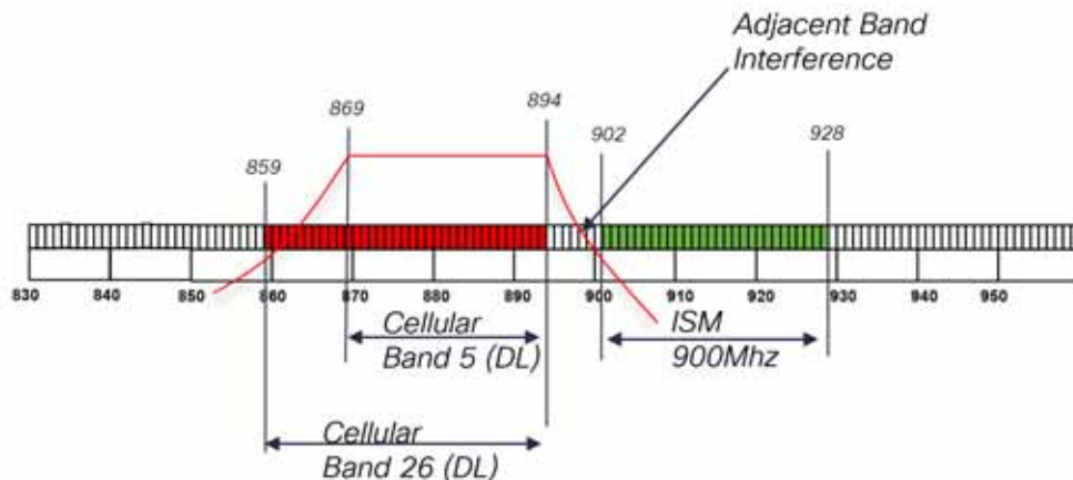
Figure 136 ISM Adjacent Frequency Bands Considerations
