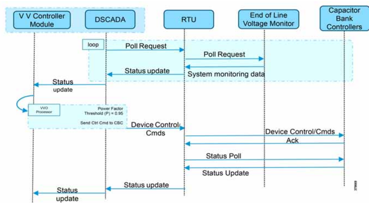
Figure 5 Power Factor Regulation Flows
