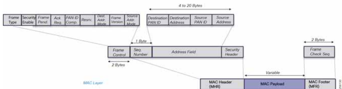
Figure 142 MHR Fields
