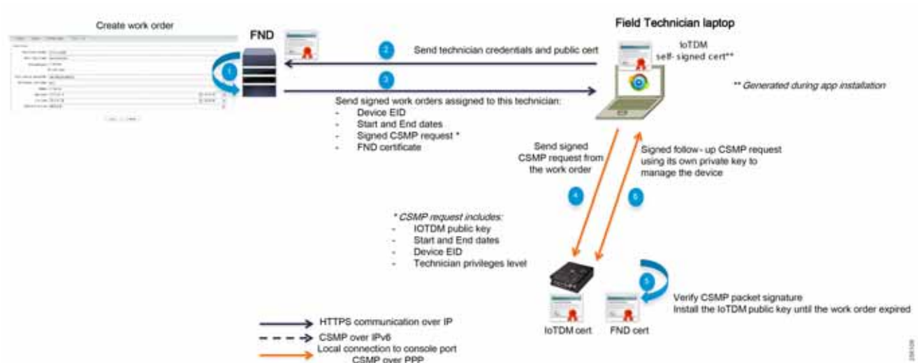
Figure 117 Work Order Process Flow
