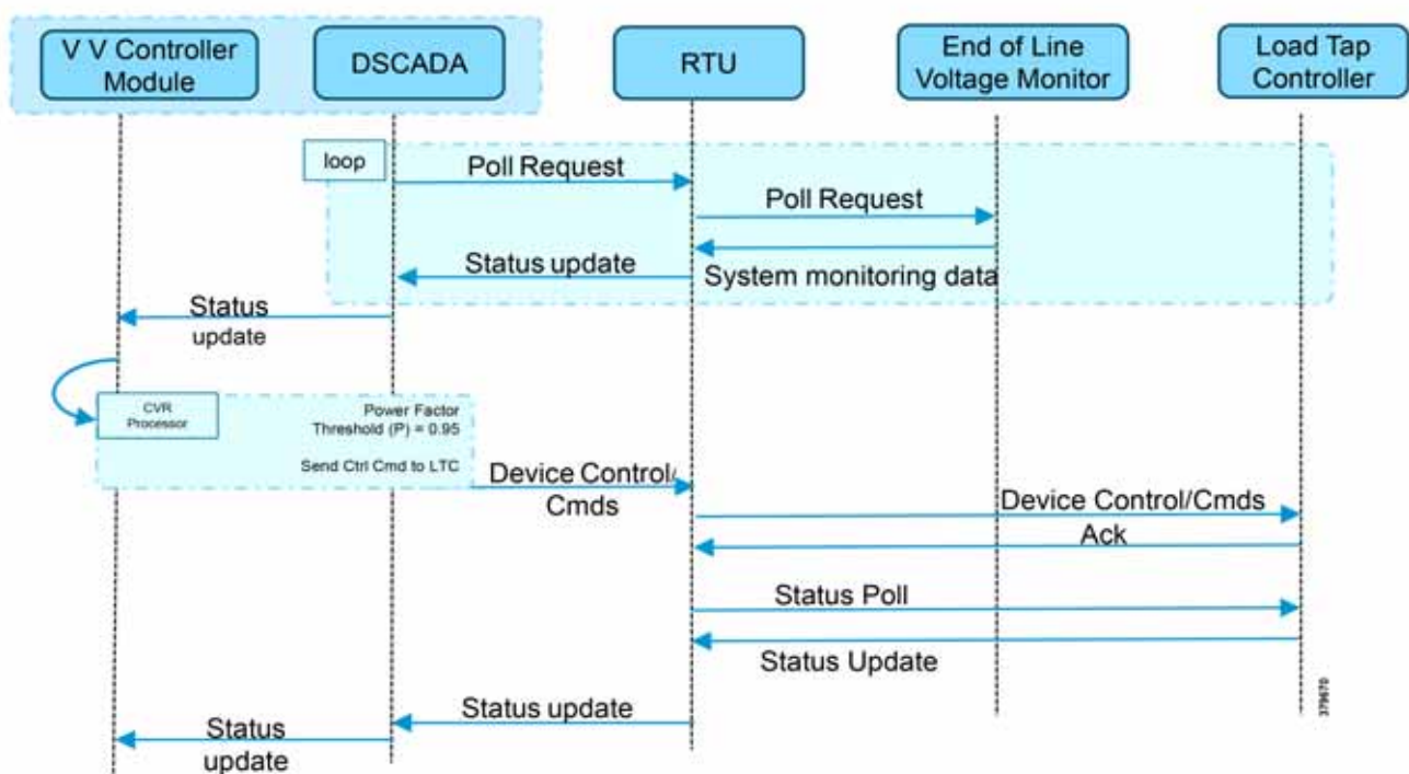
Figure 6 Conservation Voltage Regulation (CVR)
