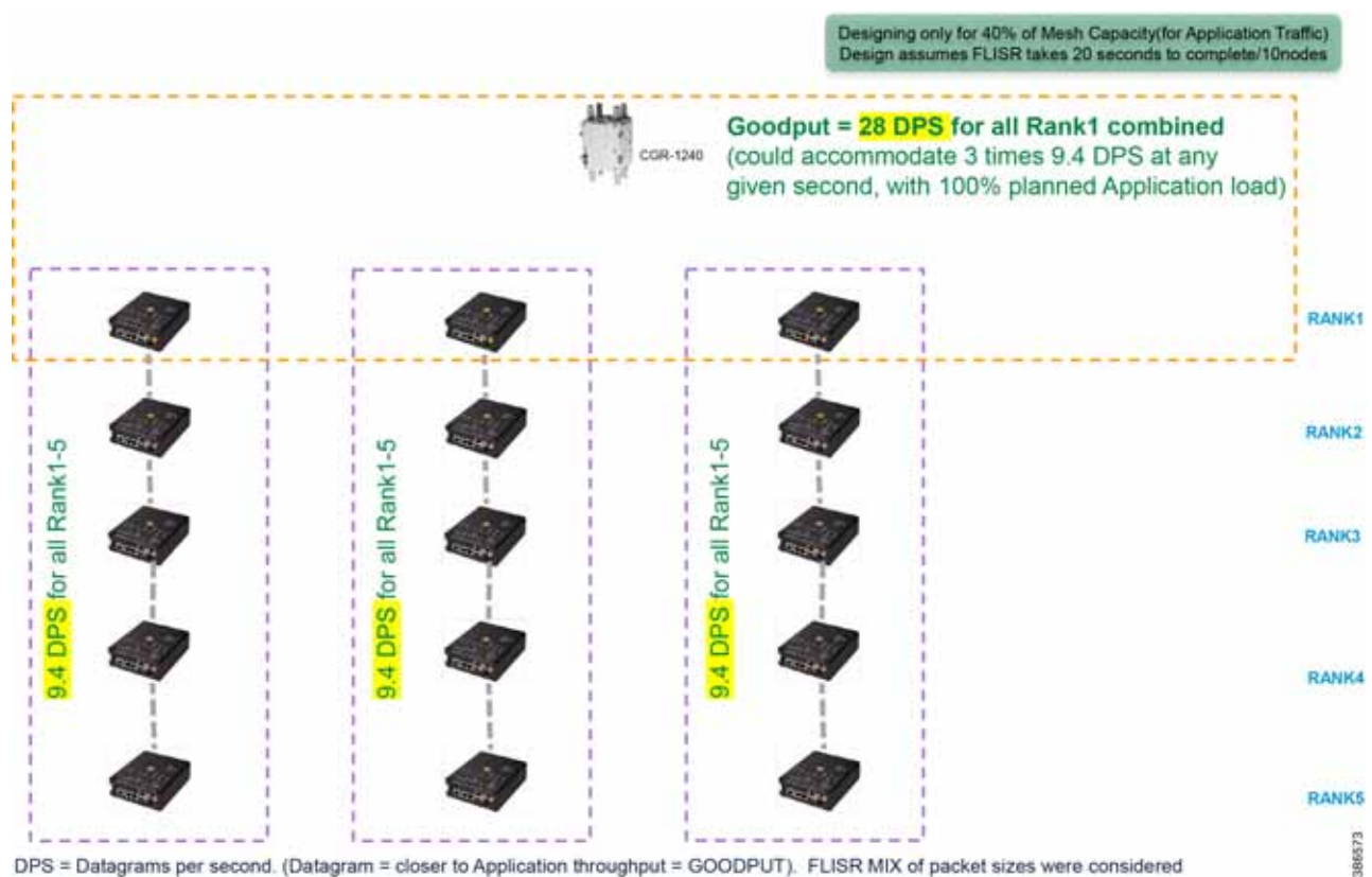
Figure 40 Considering up to 5 nodes per rank1 hierarchy
