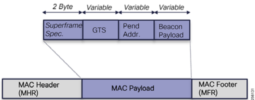
Figure 143 MAC Beacon Frame Fields
