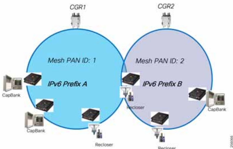
Figure 62 CGR WPAN and IPv6 Address Assignment
