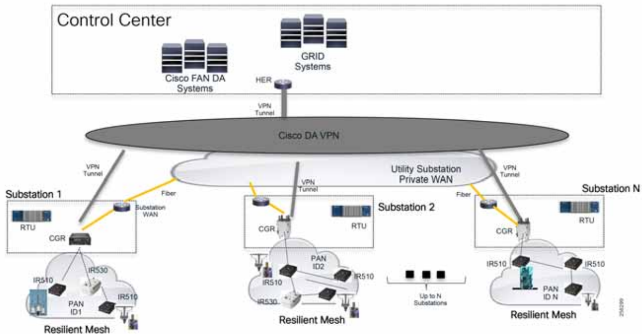
Figure 57 High Level Design Topology
