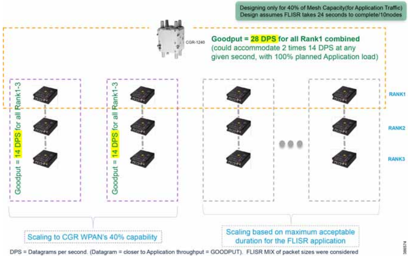
Figure 41 Considering up to 3 nodes per rank1 hierarchy
