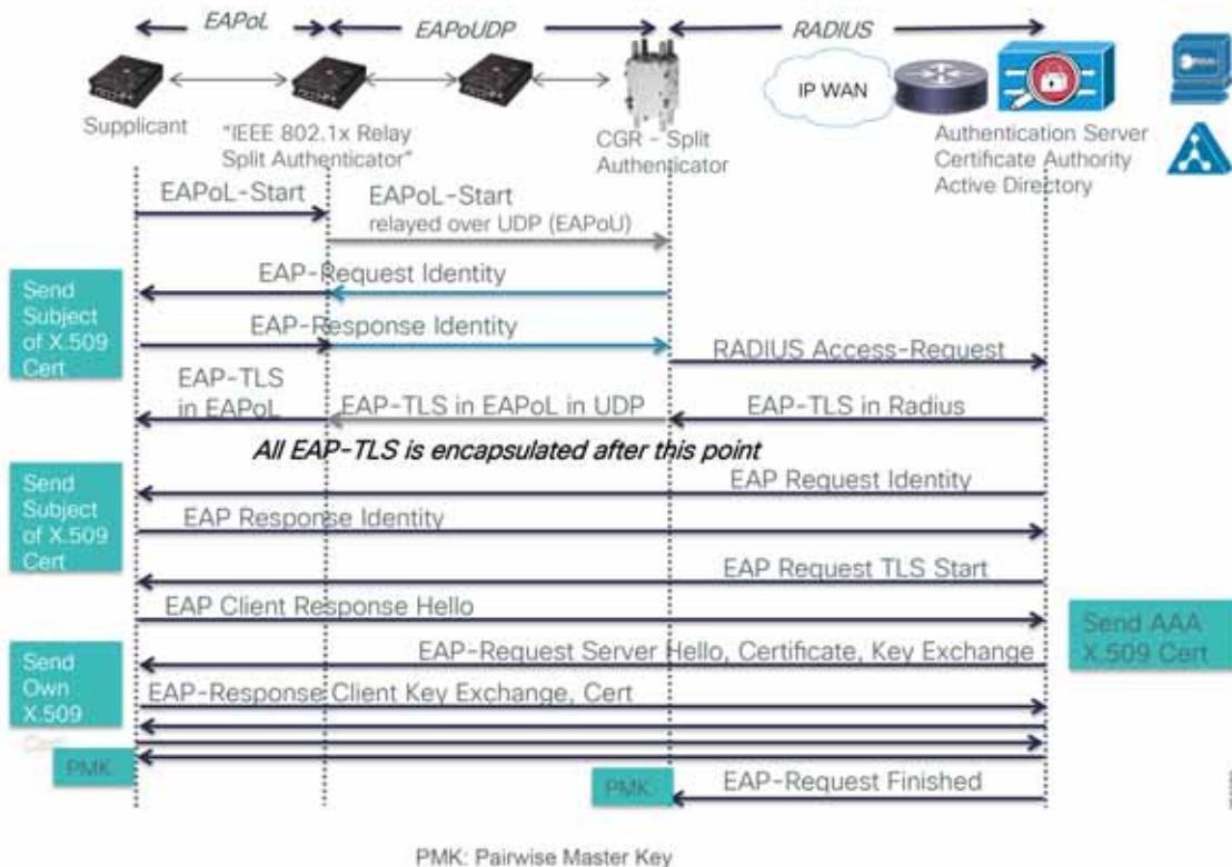
Figure 94 IEEE 802.1x Device Authentication
