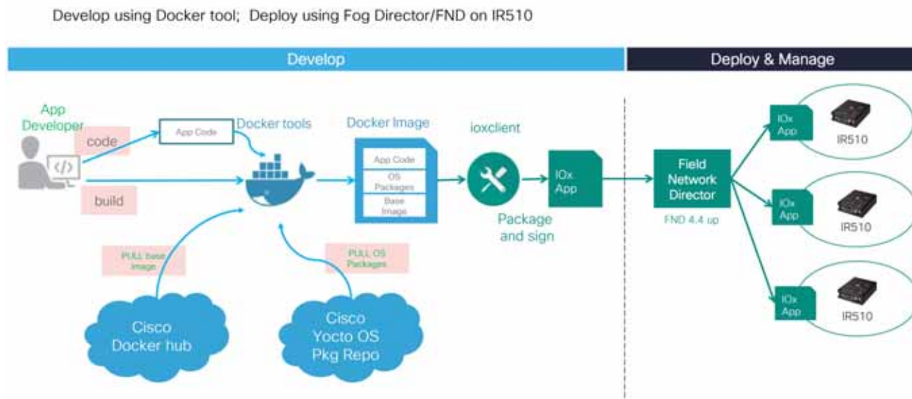
Figure 113 Edge Compute Develop and Deployment Overview
