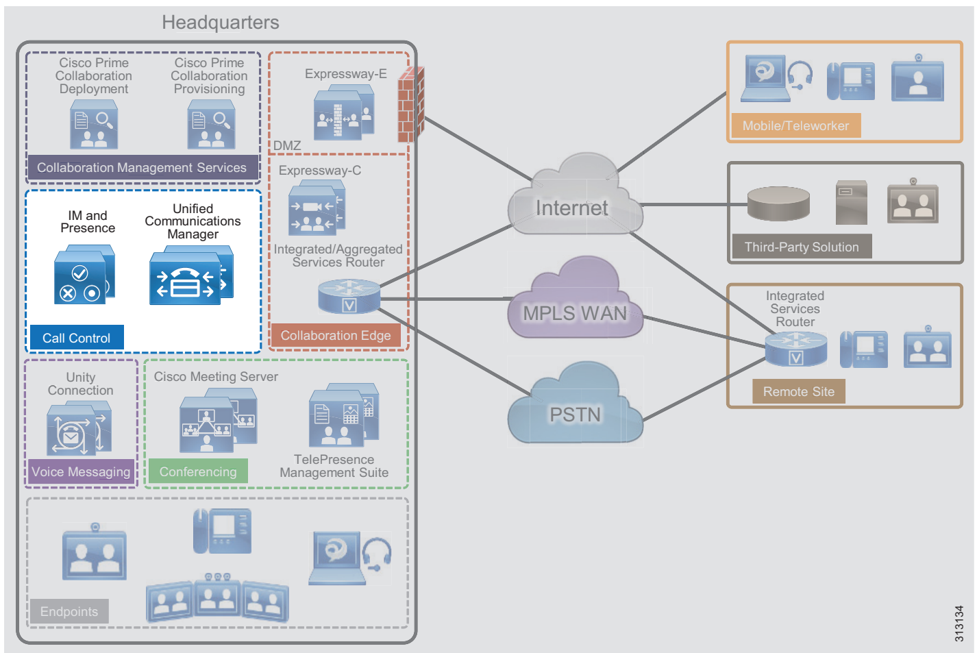
Figure 6 Architecture for Call Control
