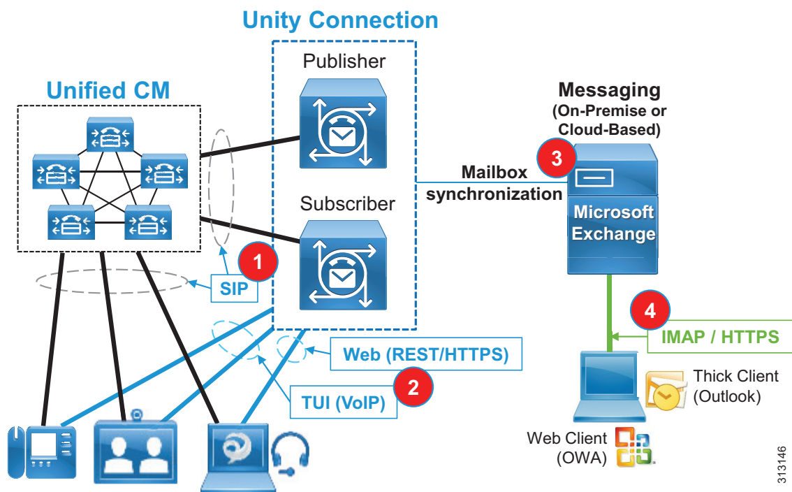
Figure 19 Unified Messaging Architecture
