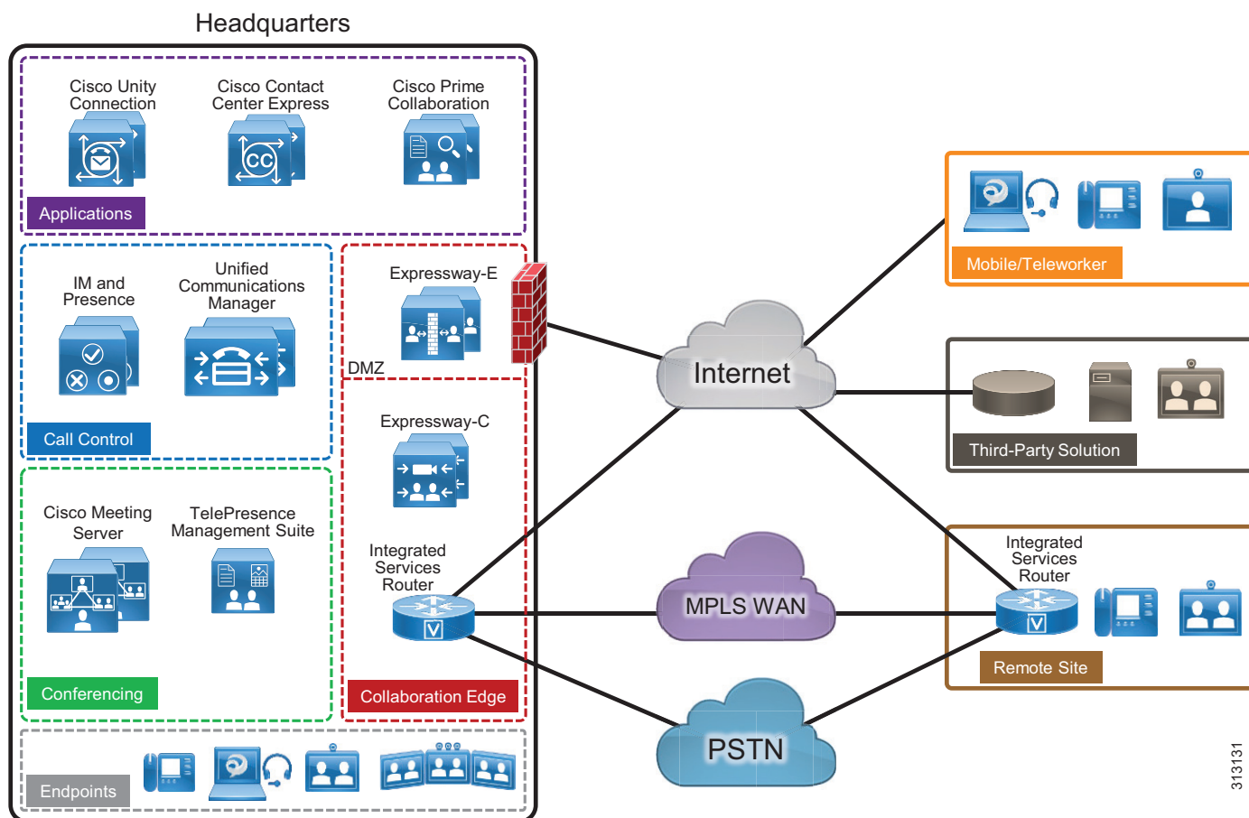
Figure 3 Cisco Collaboration On-Premises Preferred Architecture for Midmarket
