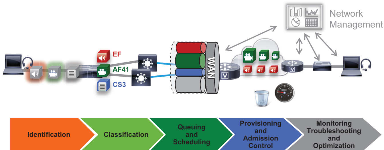
Figure 24 Architecture for Bandwidth Management
