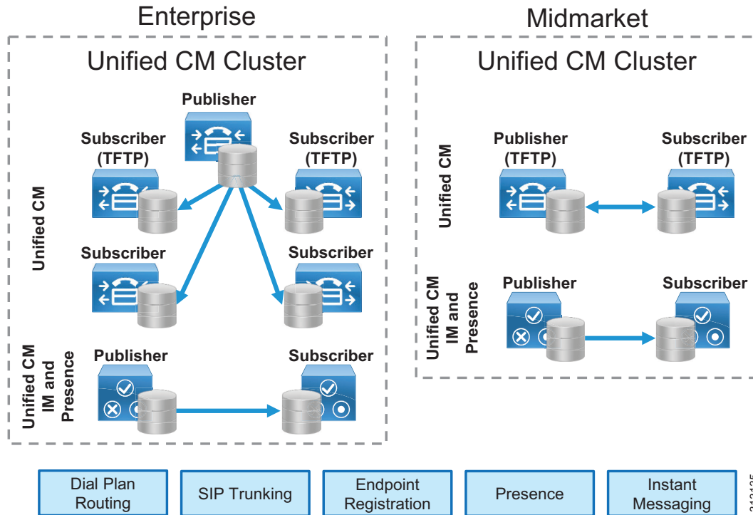
Figure 7 Cisco Unified CM Cluster
