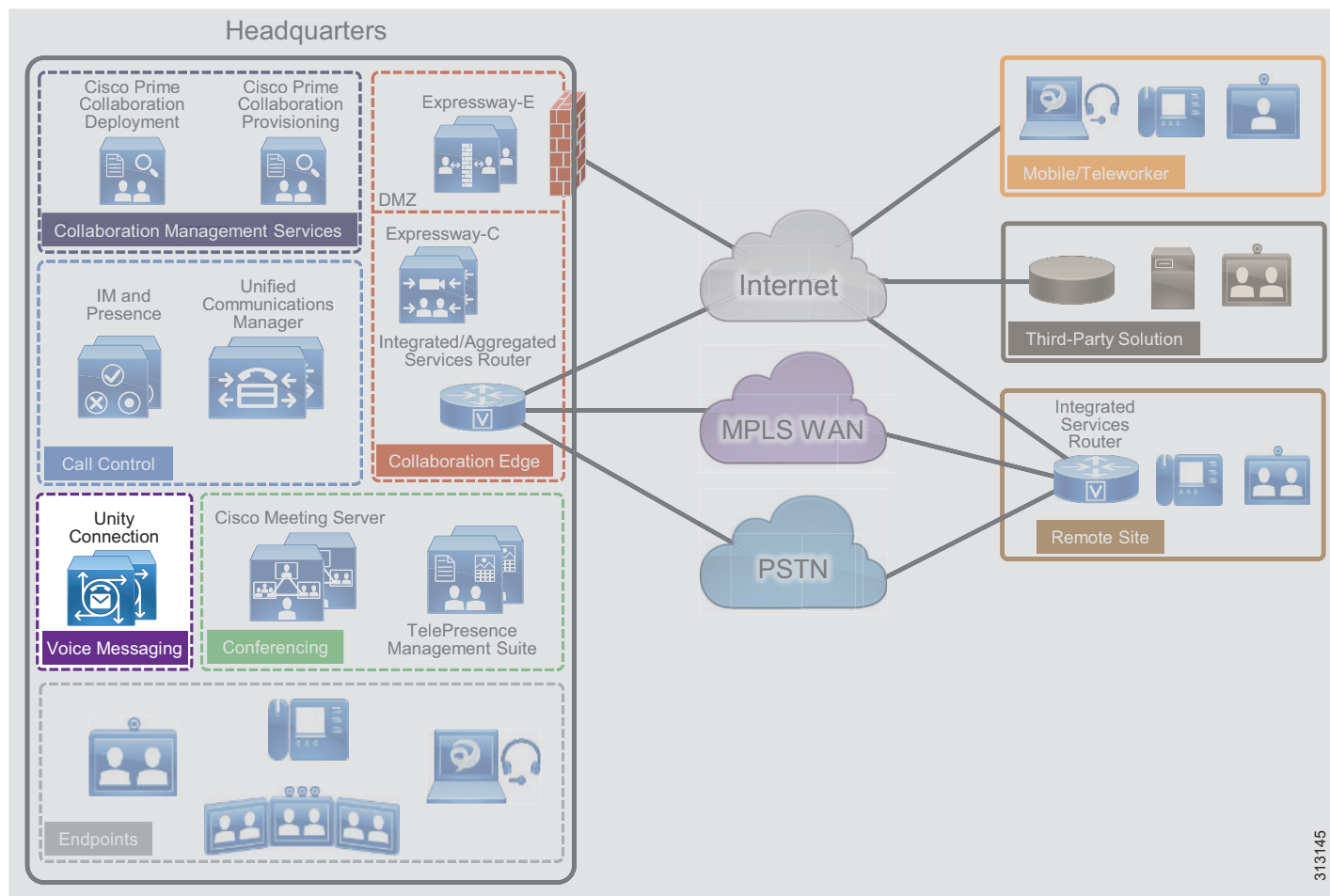
Figure 18 Architecture for Voice Messaging
