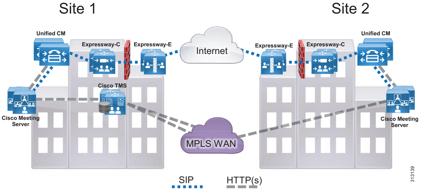
Figure 11 Multiple Call Processing Sites with Conferencing
