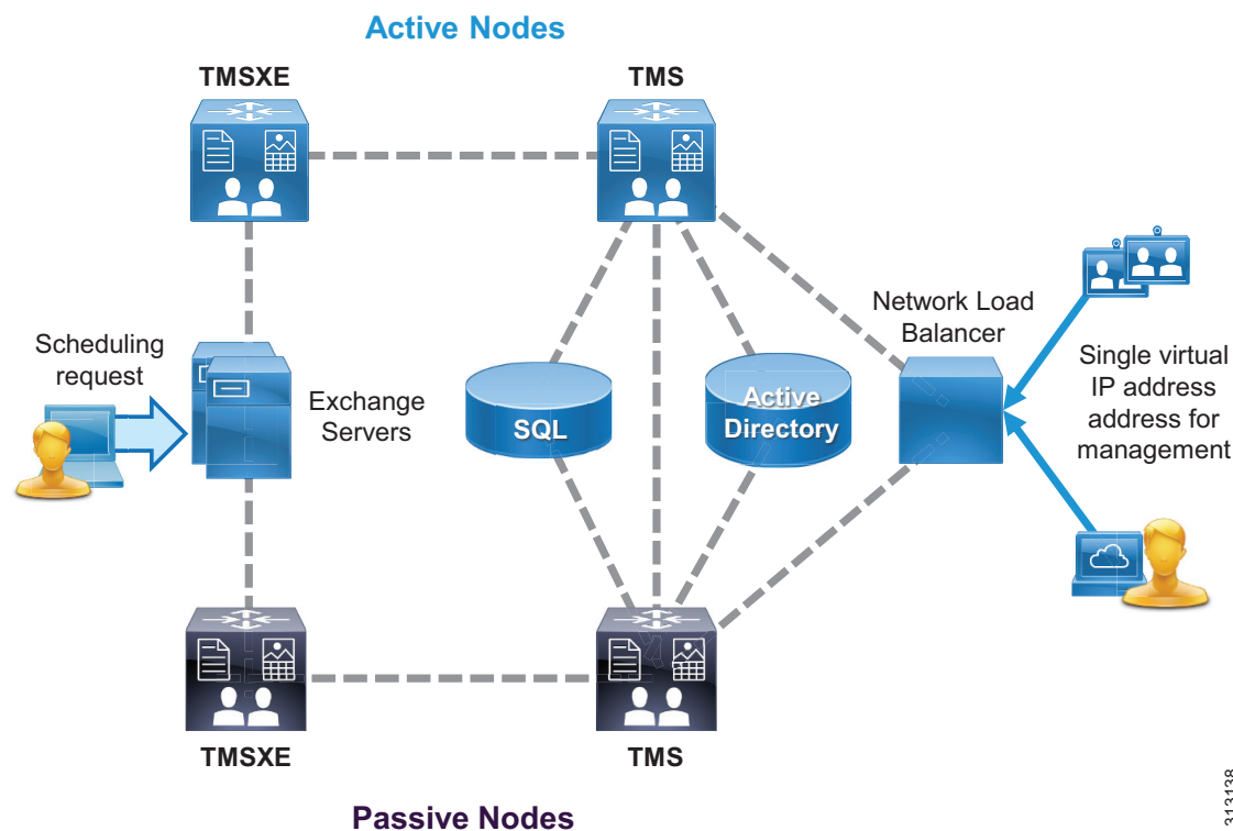
Figure 10 Cisco TMS Redundancy Model
