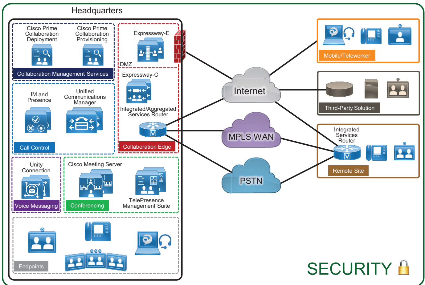
Figure 23 Secure All Components of the Enterprise Collaboration Preferred Architecture
