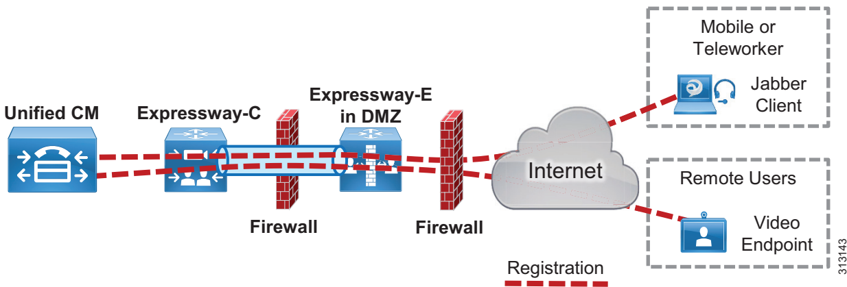
Figure 15 Traversal for Endpoint Registrations Through Firewall with Expressway-C and Expressway-E
