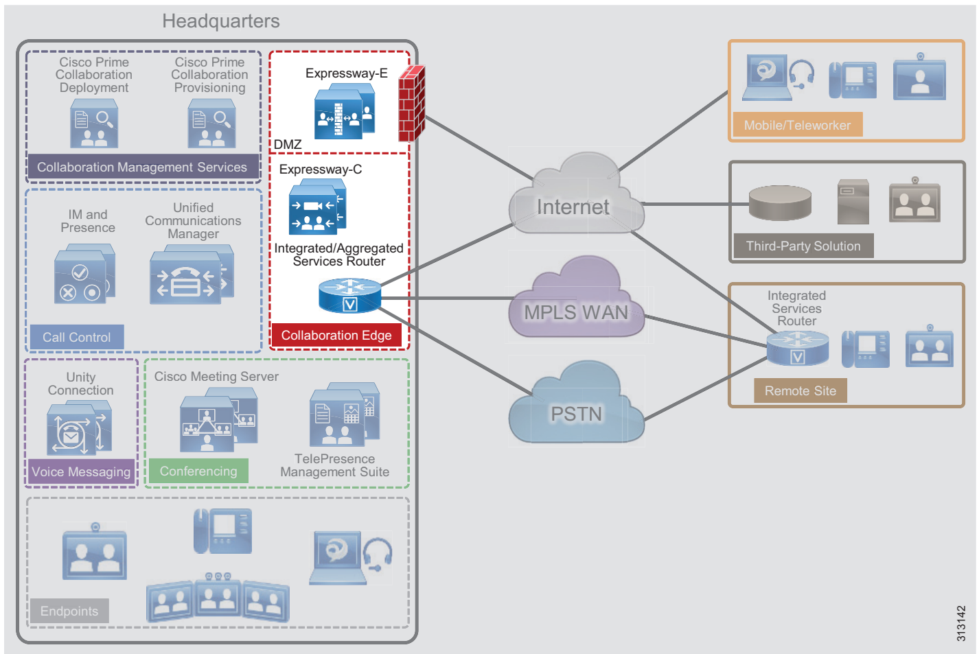
Figure 14 Architecture for Collaboration Edge
