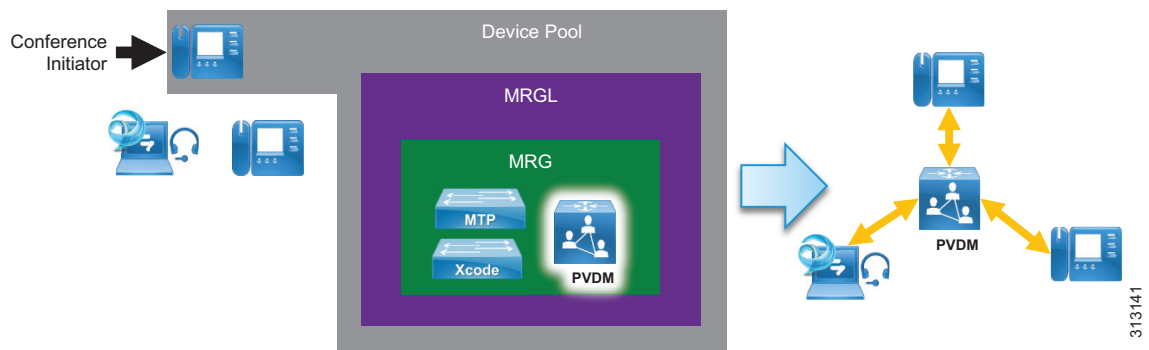
Figure 13 Media Resource Group List (MRGL) Example
