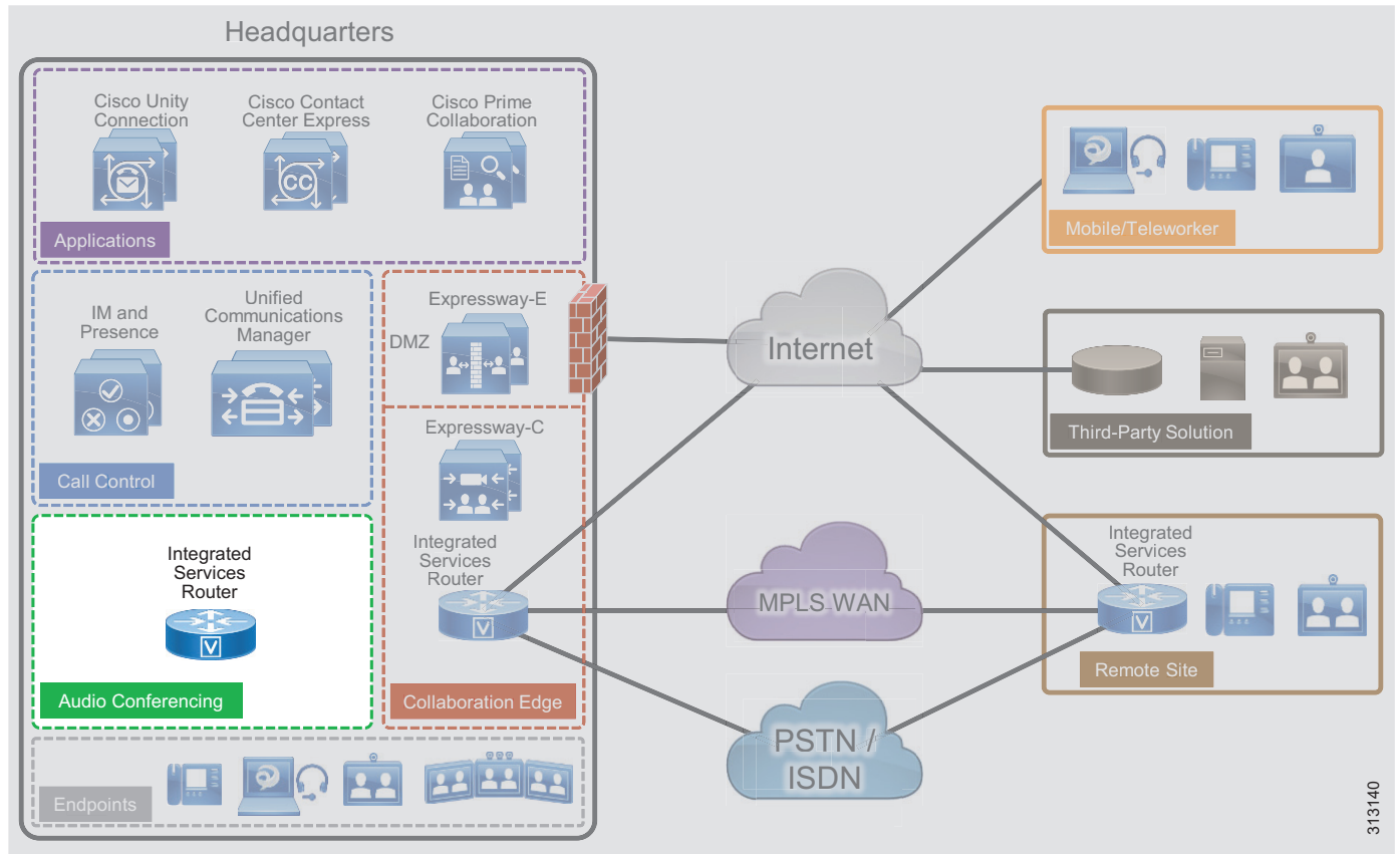
Figure 12 Architecture for Audio-Only Conferencing
