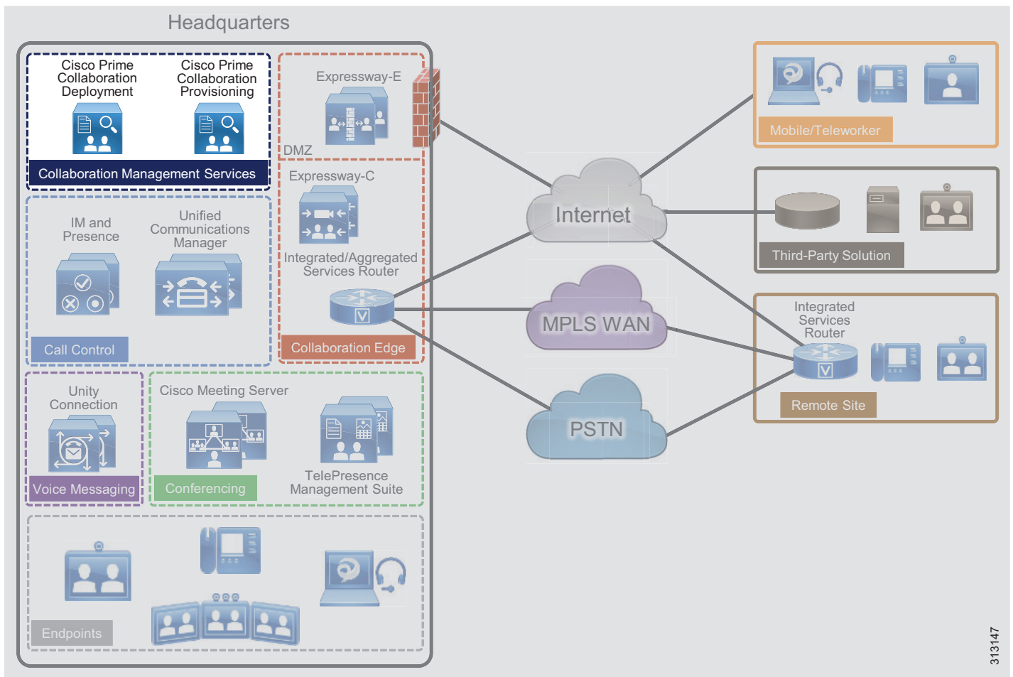
Figure 20 Architecture for Collaboration Management Services
