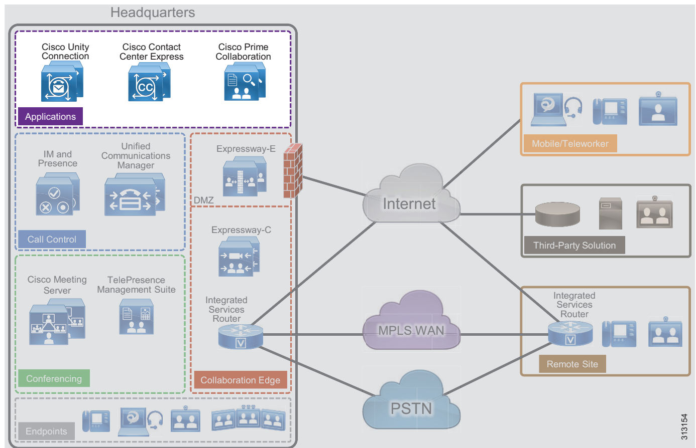
Figure 25 Architecture for Midmarket Applications
