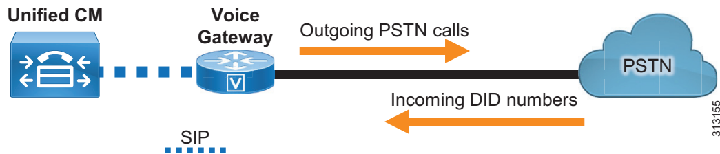
Figure 17 PSTN Connectivity
