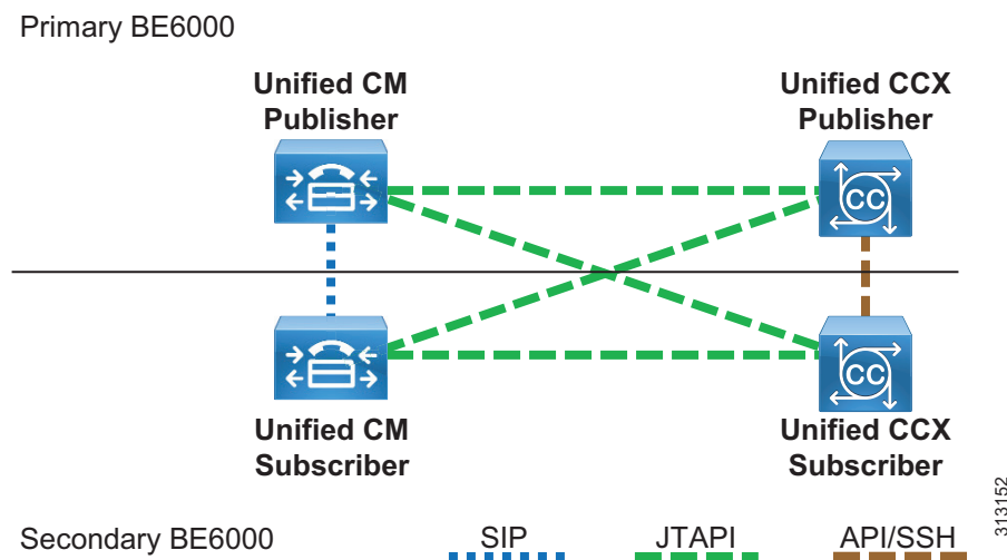
Figure 26 Cisco Unified Contact Center Express Cluster
