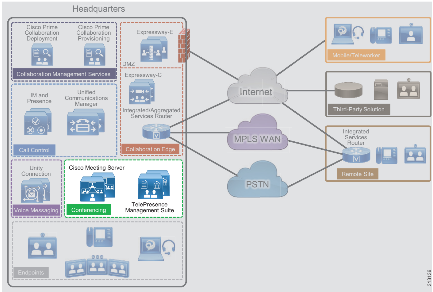
Figure 8 Architecture for Conferencing
