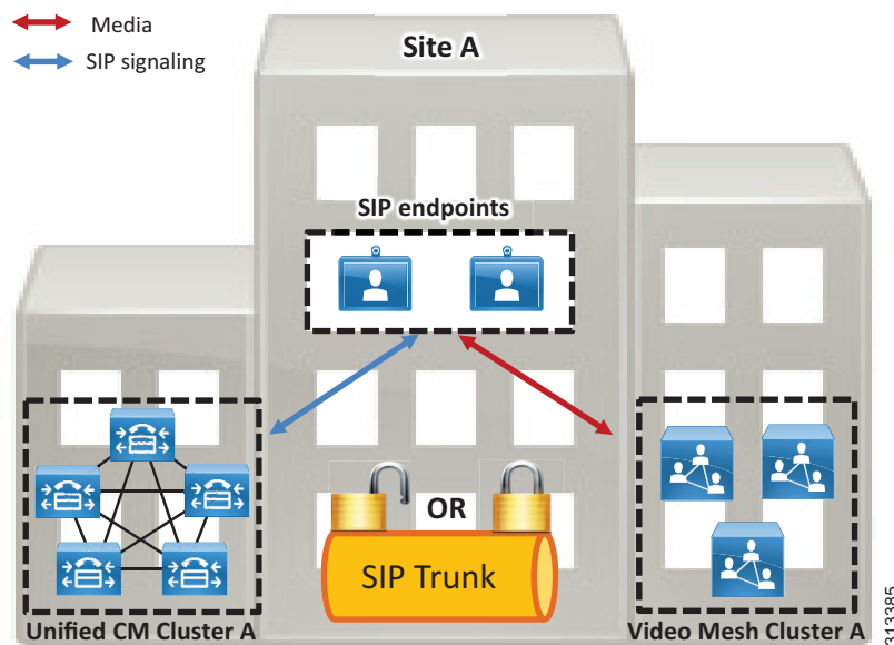
Figure 4-12 SIP Trunk Configured to Point to a Video Mesh Cluster
