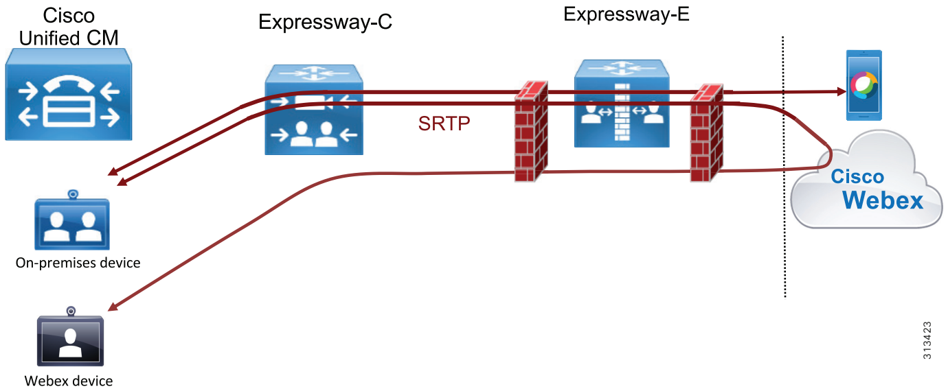
Figure 5-10 Device-terminated encryption
