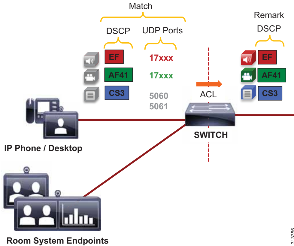
Figure 8-25 Desktop and Room System Endpoint QoS
