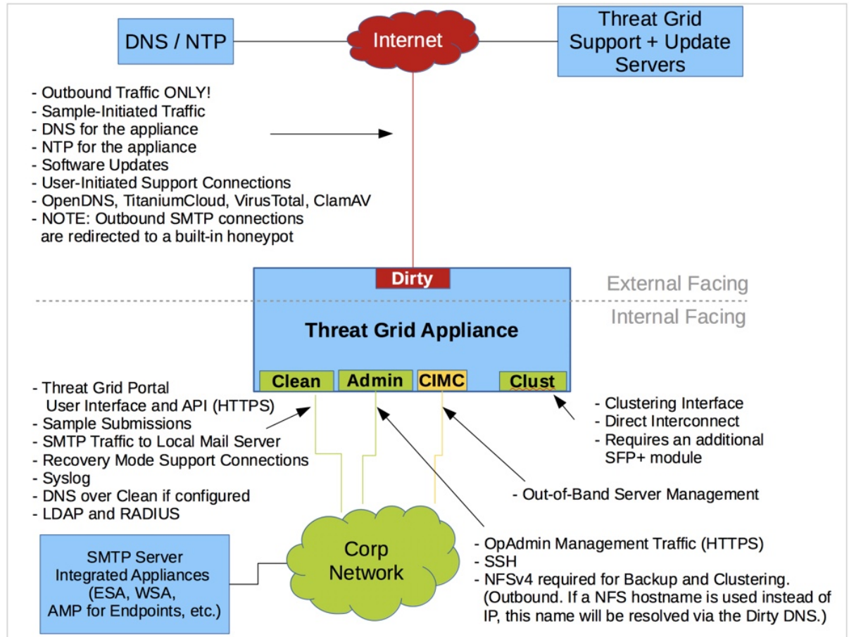
Figure 2: Network Interfaces Setup Diagram
