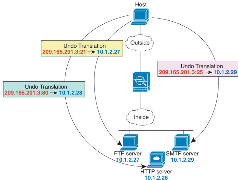
Figure 18: Static NAT-with-Port-Translation
