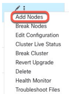
Figure 9: Add Nodes
