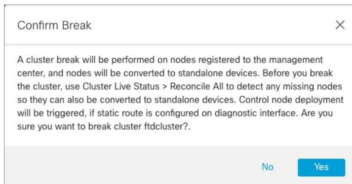
Figure 15: Confirm Break
