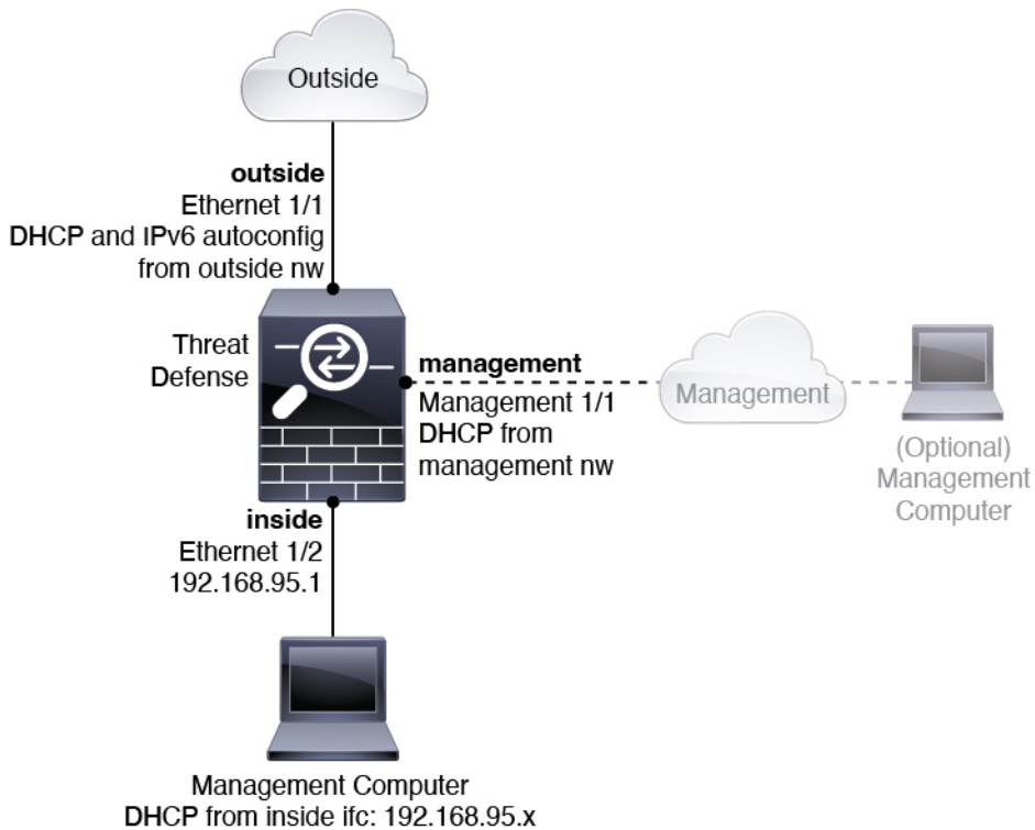
Figure 73: Suggested Network Deployment
