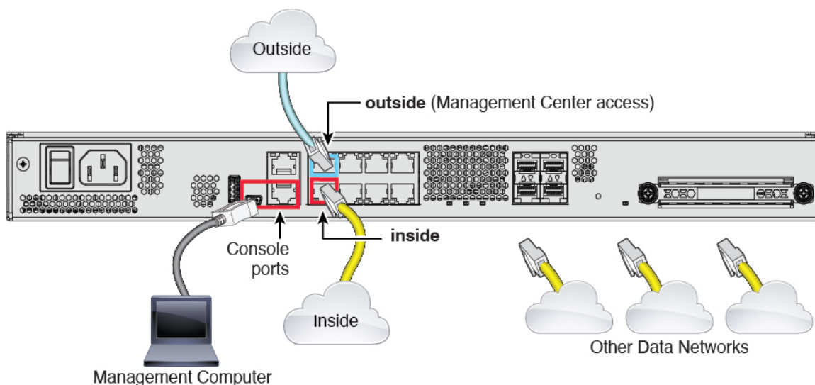
Figure 39: Cabling a Remote Management Deployment
