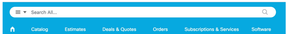
Figure 5: License Search
