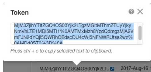
Figure 2: Copy Token
