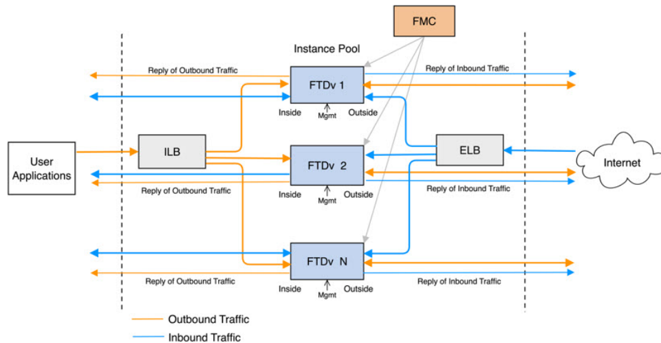
Figure 41: Secure Firewall Threat Defense Virtual Auto Scale Use Case Diagram
