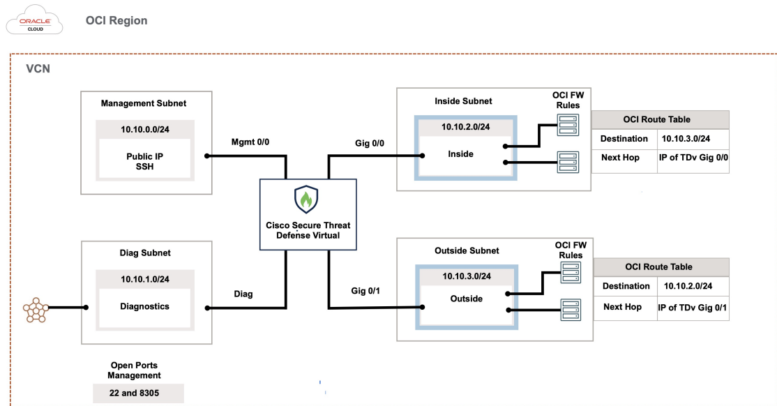
Figure 39: Sample Threat Defense Virtual on OCI Deployment with four subnets in a VCN
