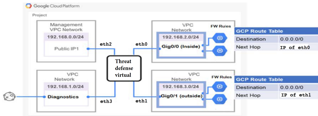
Figure 46: Sample Threat Defense Virtual on GCP Deployment
