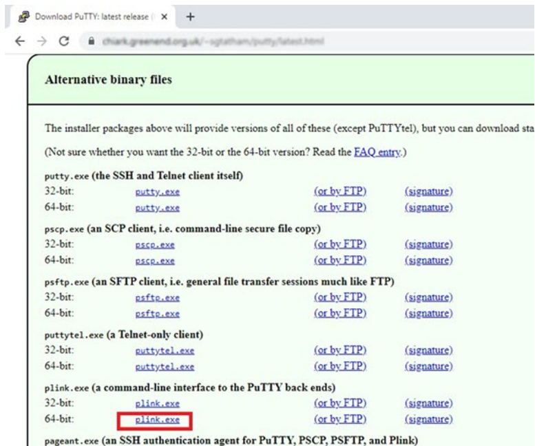
Figure 23: Download PuTTY
