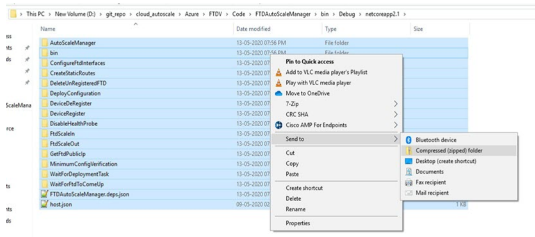
Figure 35: Build ASM_Function.zip
