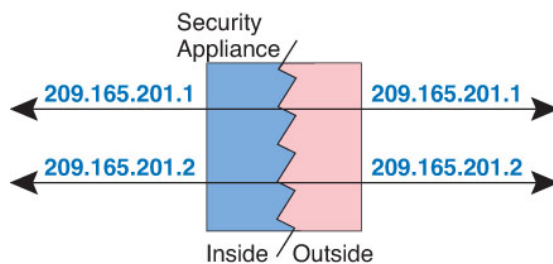
Figure 12: Identity NAT
