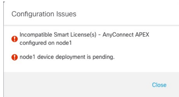
Figure 4: Configuration Issues
