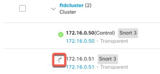
Figure 19: Node Registration
