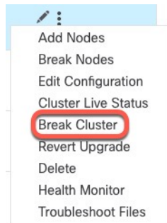
Figure 22: Break Cluster
