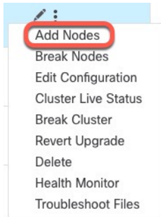
Figure 17: Add Nodes
