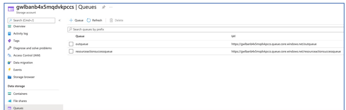
Figure 12: Queues
