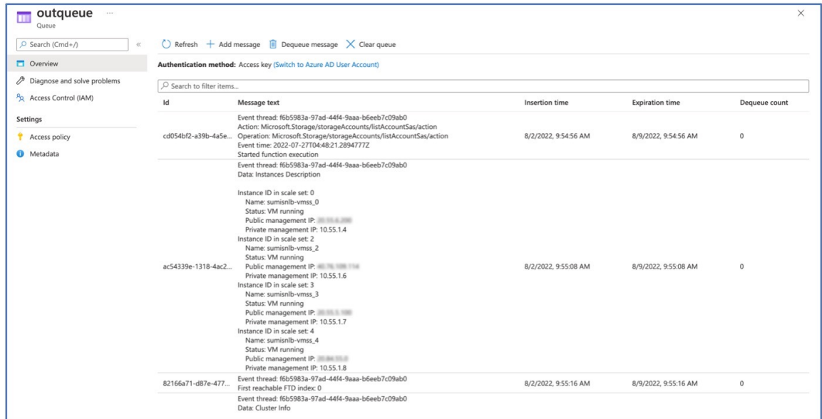
Figure 13: Outqueue
