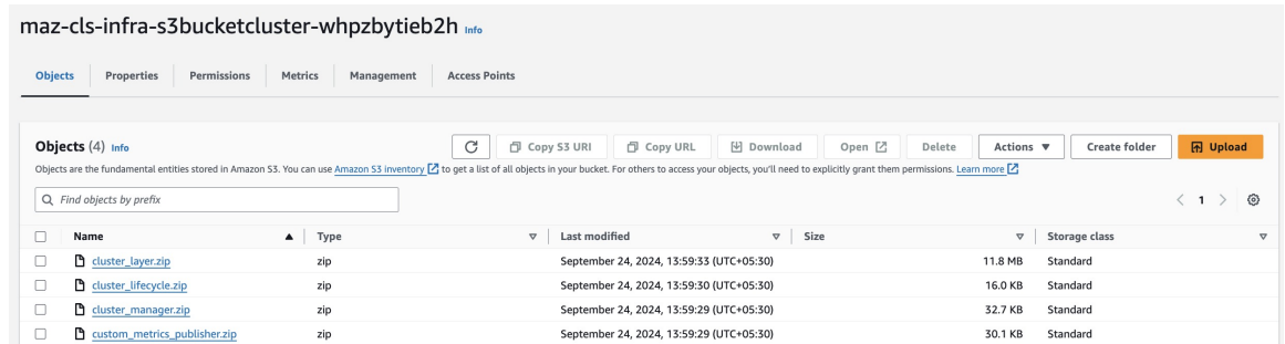
Figure 3: S3 Bucket
