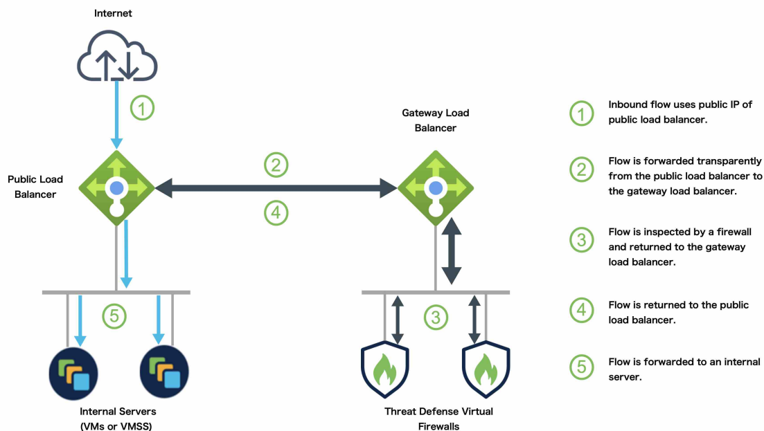
Figure 7: Inbound Traffic Use Case and Topology with GWLB
