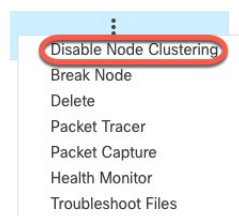
Figure 19: Disable Clustering
