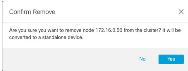
Figure 16: Confirm Break
