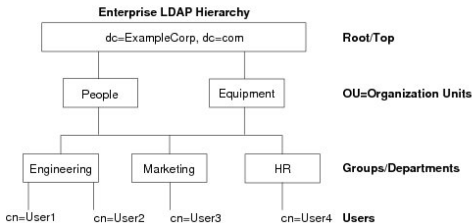
Figure 84: A Multi-Level LDAP Hierarchy
