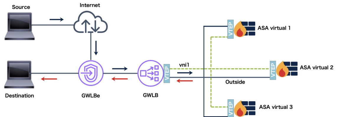
Figure 60: Geneve Single-Arm Proxy
