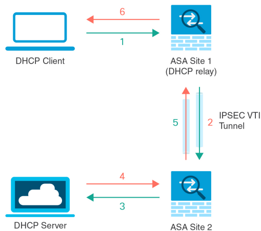
Figure 75: DHCP Relay Server over VTI
