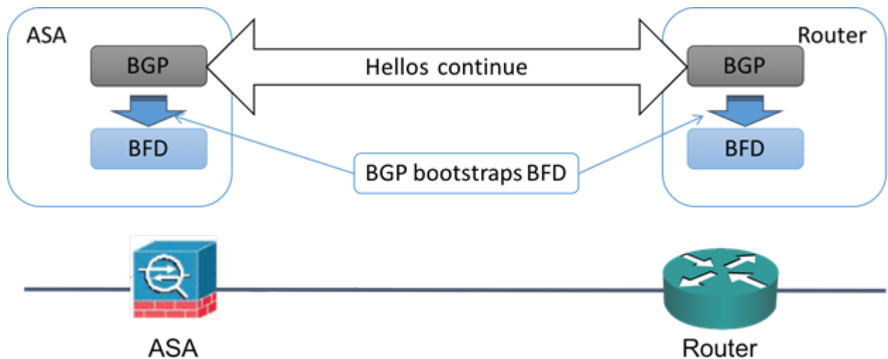
Figure 78: Established BFD Session
