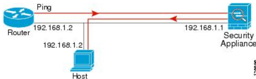
Figure 91: Ping Failure Because of IP Addressing Problems
