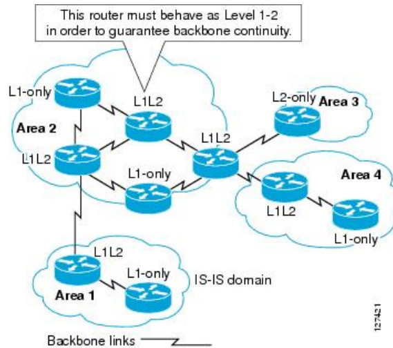
Figure 81: Level-1, Level-2, Level 1-2 Devices in an IS-IS Network Topology
