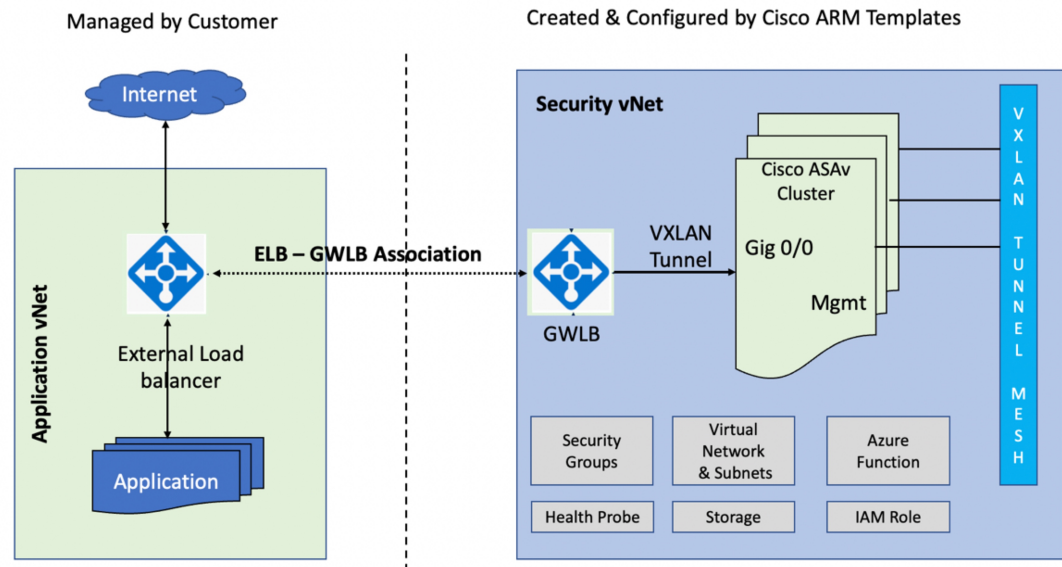
Figure 63: ASAv Clustering on Azure with GWLB
